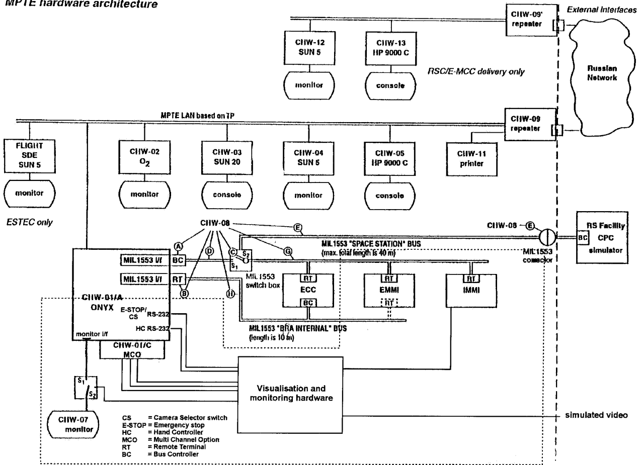
MPTE hardware architecture
