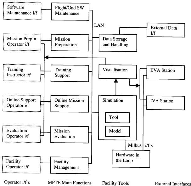
Figure 3.: MPTE Functional Breakdown
