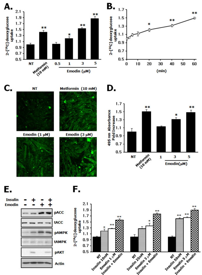
FIGURE 2. Increase of GLUT4 translocation and glucose uptake in response to emodin. A , L6 myotubes were equilibrated in glucose-free Krebs-Ringer buffer for 1 h and then incubated with the indicated concentrations of emodin for 1 h. [ 14 C]2-DOG uptake was measured as described under "Experimental Procedures." B , L6 myotubes were incubated with 3 \mu M emodin for 0 to 1 h, and glucose uptake was measured. C , immunofluorescent detection of surface GLUT4 on confluent, quiescent L6 myotubes. The cells were treated with 3 \mu M emodin for 1 h, and surface GLUT4 levels were determined. NT , not treated with emodin. D , quantitative analysis of surface GLUT4. Exposure of GLUT4 was detected using the anti-Myc antibody and coupled to the o -phenylenediamine assay as described under "Experimental Procedures." E , co-treatment with 3 \mu M emodin and 25 nM insulin for 5 min. AMPK phosphorylation was quantified by densitometry and normalized to the total AMPK. Data represent one out of four independent experiments. F , [ 14 C]2-DOG uptake was measured with emodin for 1 h and/or insulin for 10 min at the indicated concentration in L6 myotubes. Values are means \pm S.E. of three independent experiments performed in triplicate. *, p < 0.05 , and **, p < 0.01 versus untreated cells.
