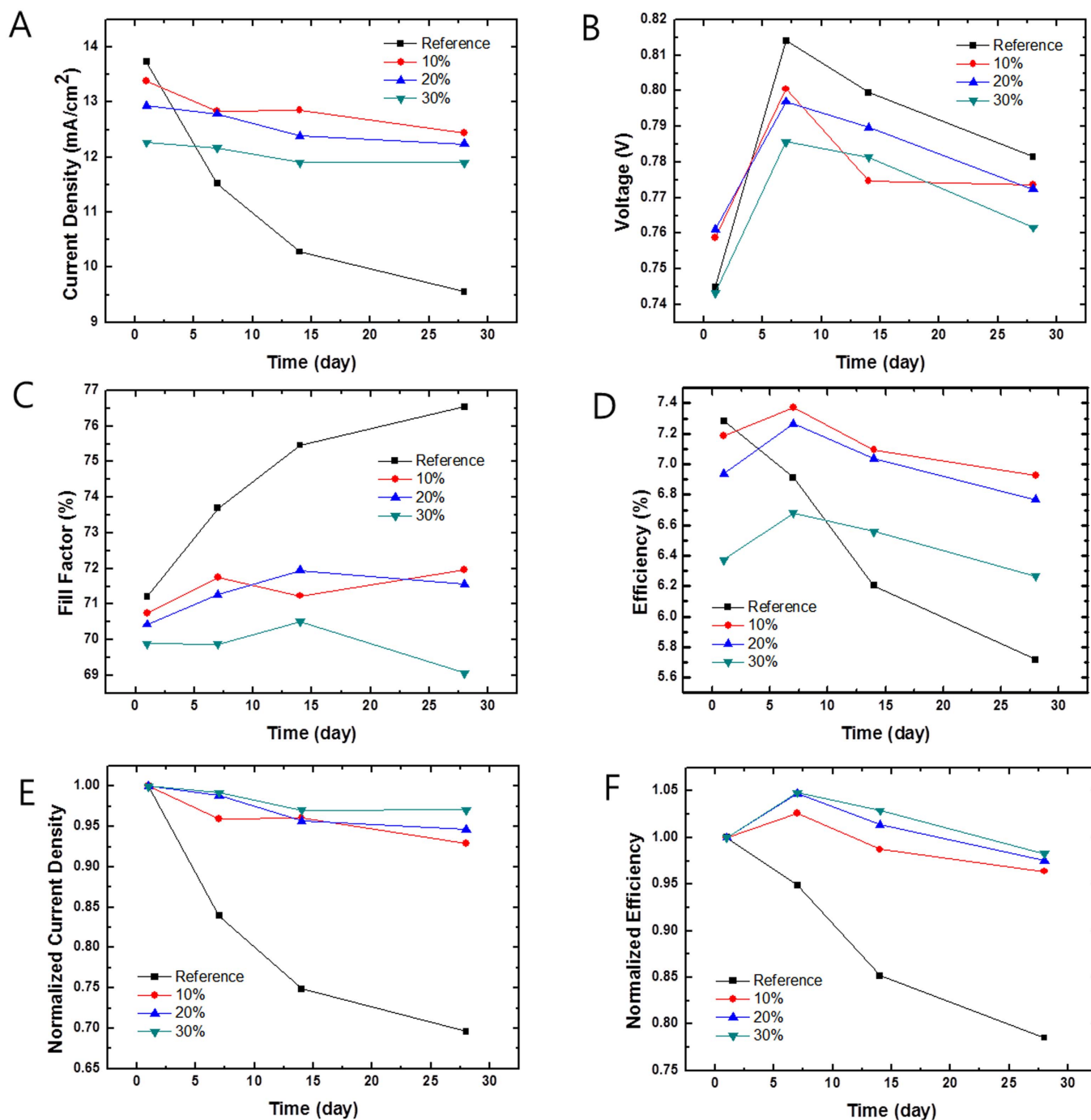
Figure 4 | Cell parameter decays for 28 days: J_{sc} (A), V_{oc} (B), FF (C) and Efficiency (D). Cell parameter decay normalized by its initial value over the 28 day period ((E) normalized J_{sc} and (F) normalized Efficiencies).
