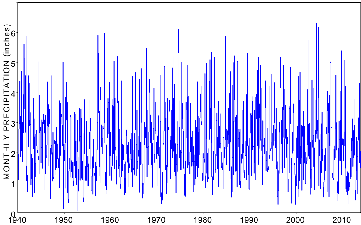
Figure 3.2 Monthly Precipitation during 1940-2013 for the 92 Quadrangles
