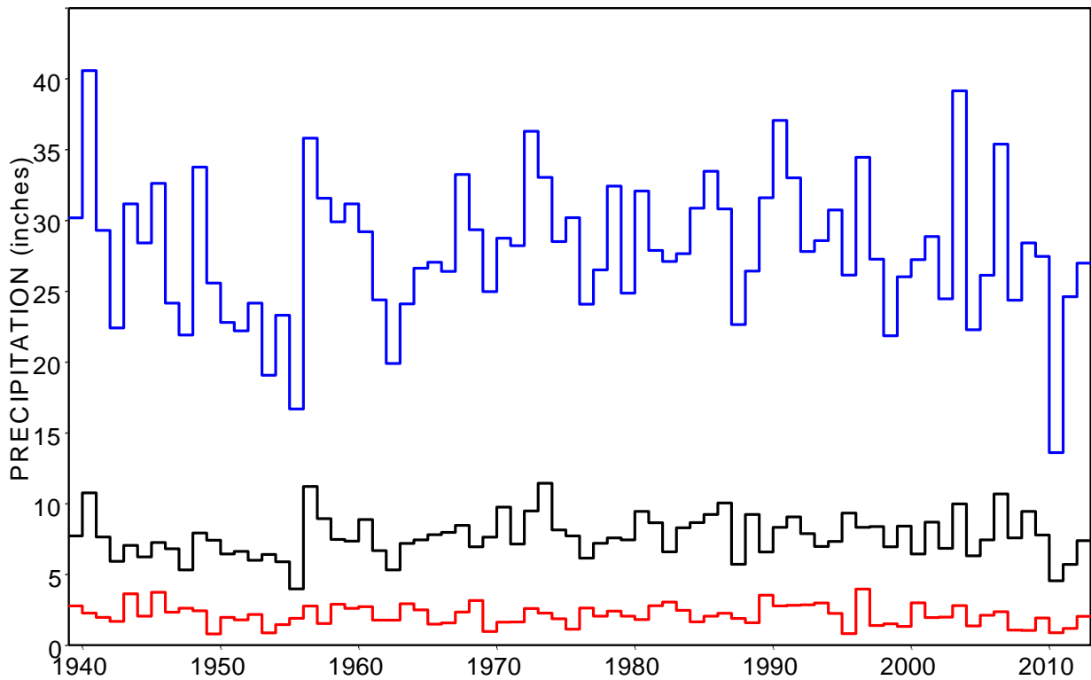
Figure 3.3 Annual Total, 2-Month Maximum, and 2-Month Minimum Precipitation During Each Year of 1940-2013 for the 92 Quadrangles
