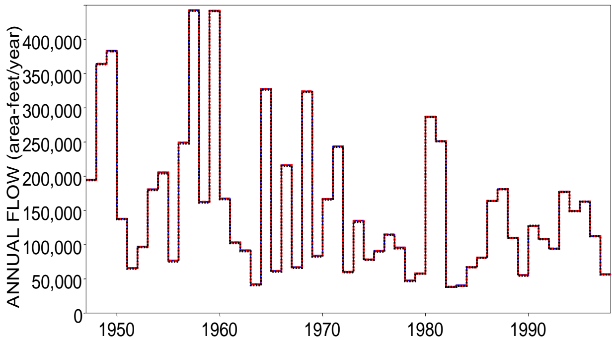
Naturalized (blue solid), Regulated (red dashed), and Observed (black dotted) Annual Flows for Canadian River near Amarillo
