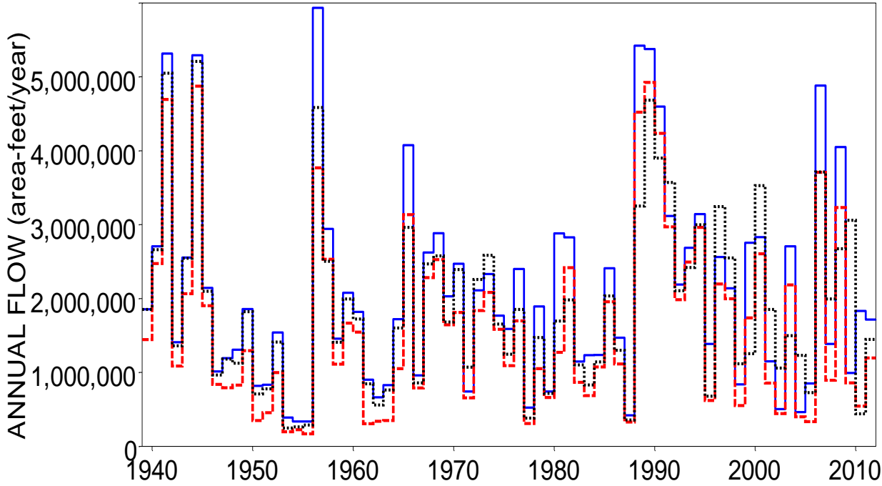
Naturalized (blue solid), Regulated (red dashed), and Observed (black dotted) 2-Month Maximum Annual Flows for Trinity River near Oakwood
