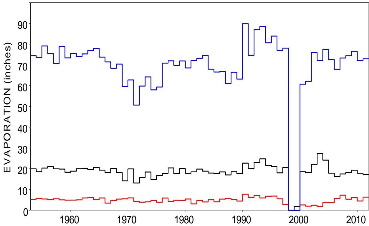
Annual Total, 2-Month Maximum, and 2-Month Minimum Evaporation for Quadrangles 701 (missing date form 1999-2000)
