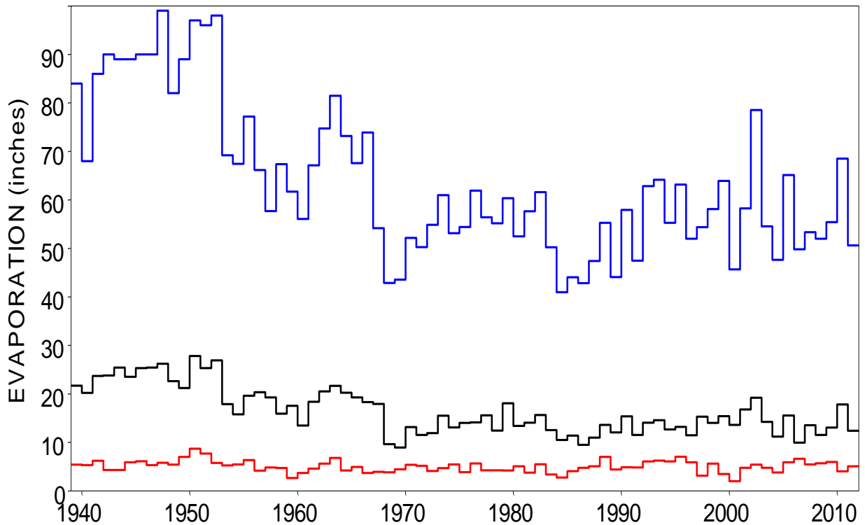
Annual Total, 2-Month Maximum, and 2-Month Minimum Evaporation for Quadrangles 704
