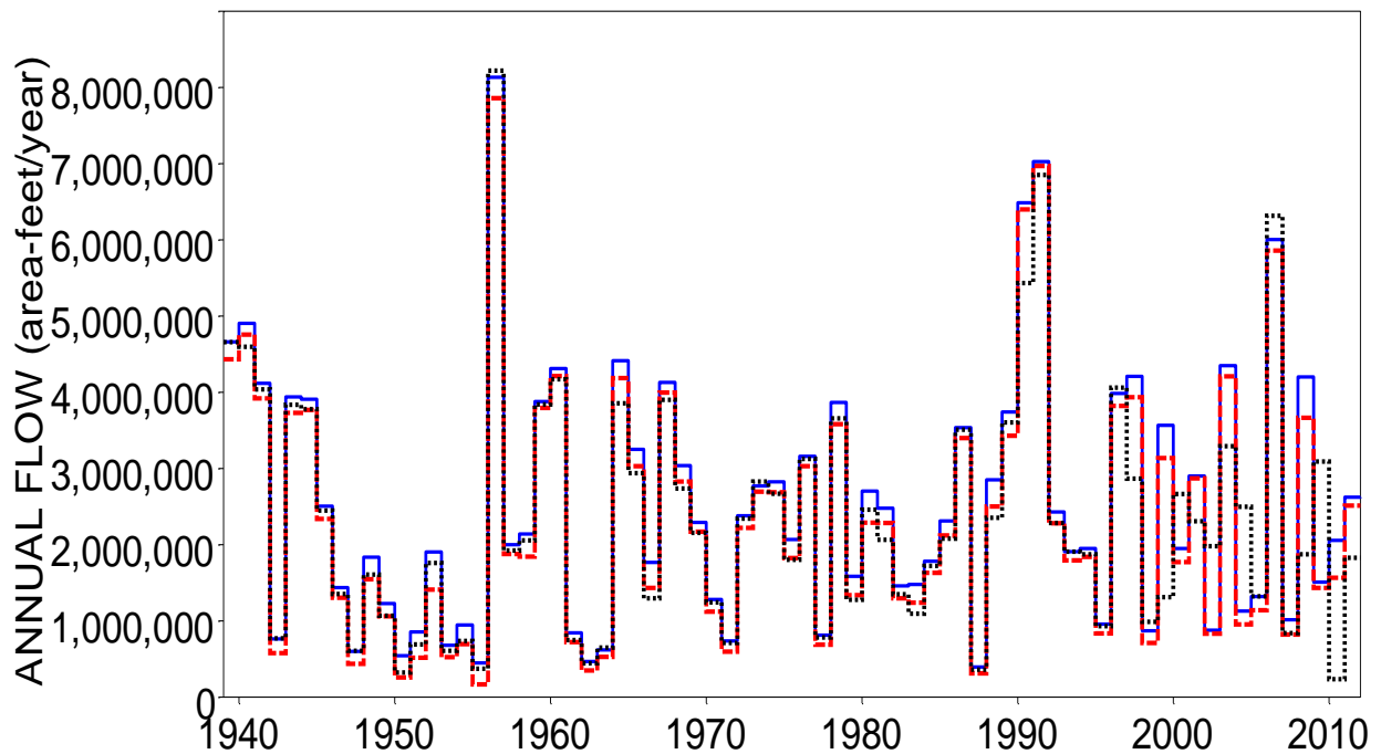
Naturalized (blue solid), Regulated (red dashed), and Observed (black dotted) 2-Month Maximum Annual Flows for Brazos River at Richmond
