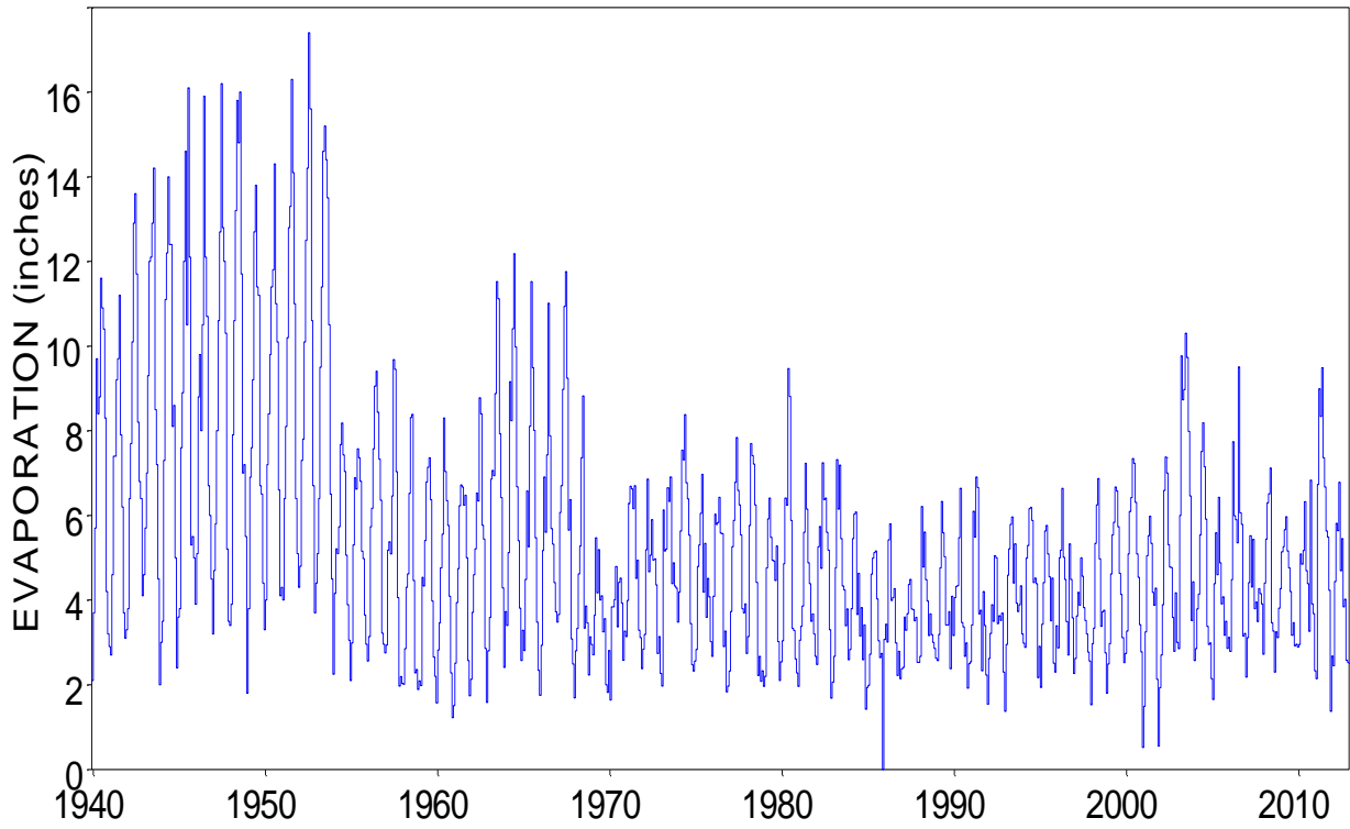
Monthly Evaporation for Quadrangle 804
