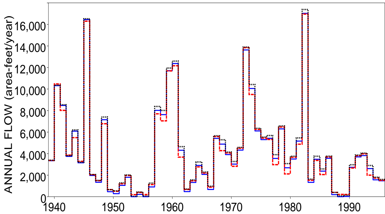
Naturalized (blue solid), Regulated (red dashed), and Observed (black dotted) 2-Month Minimum Annual Flows for Lavaca River near Edna
