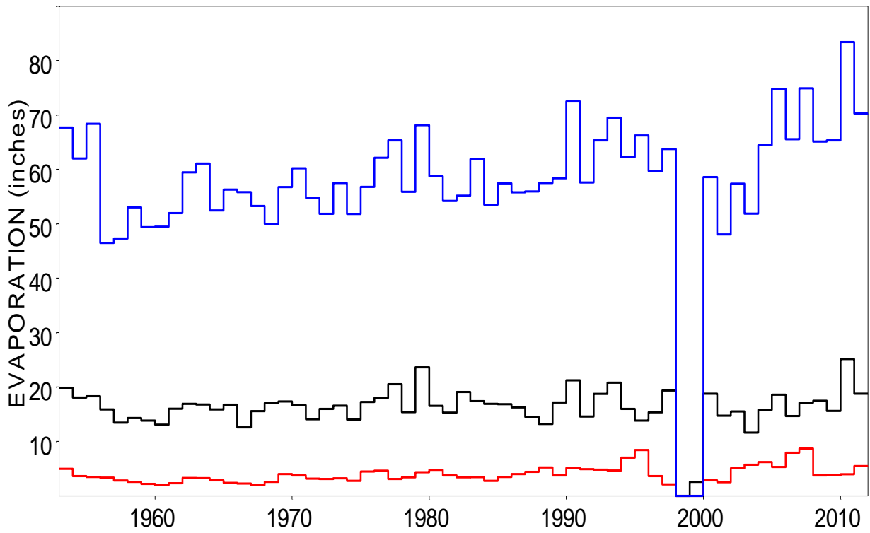
Annual Total, 2-Month Maximum, and 2-Month Minimum Evaporation for Quadrangles 108 (missing data from 1999-2000)
