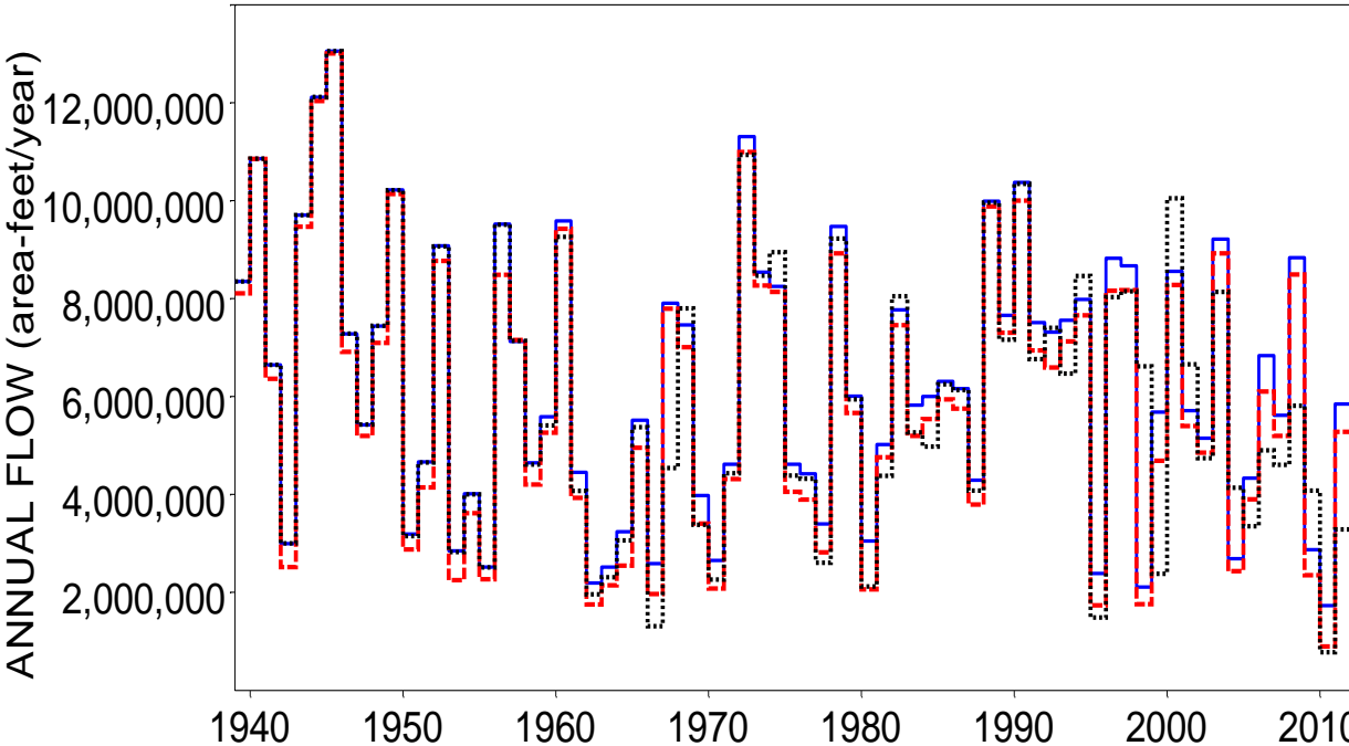
Naturalized (blue solid), Regulated (red dashed), and Observed (black dotted) Annual Flows for Sabine River near Ruliff
