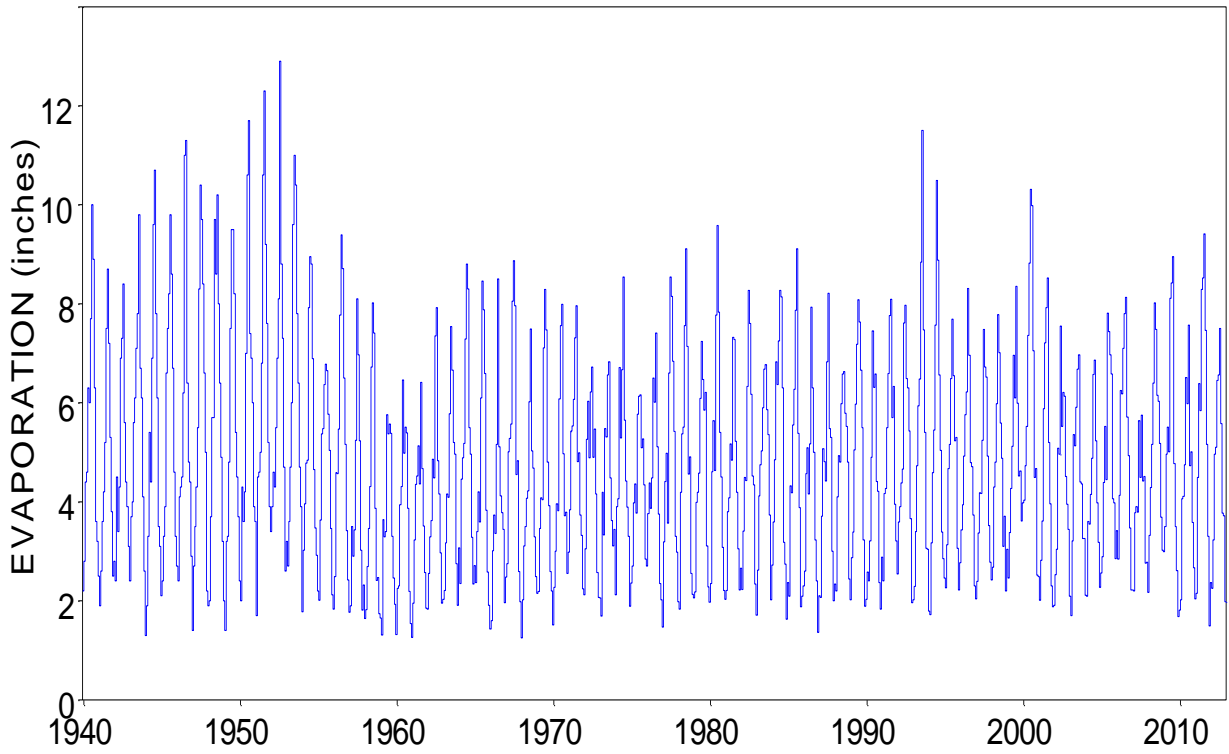
Monthly Evaporation for Quadrangle 709
