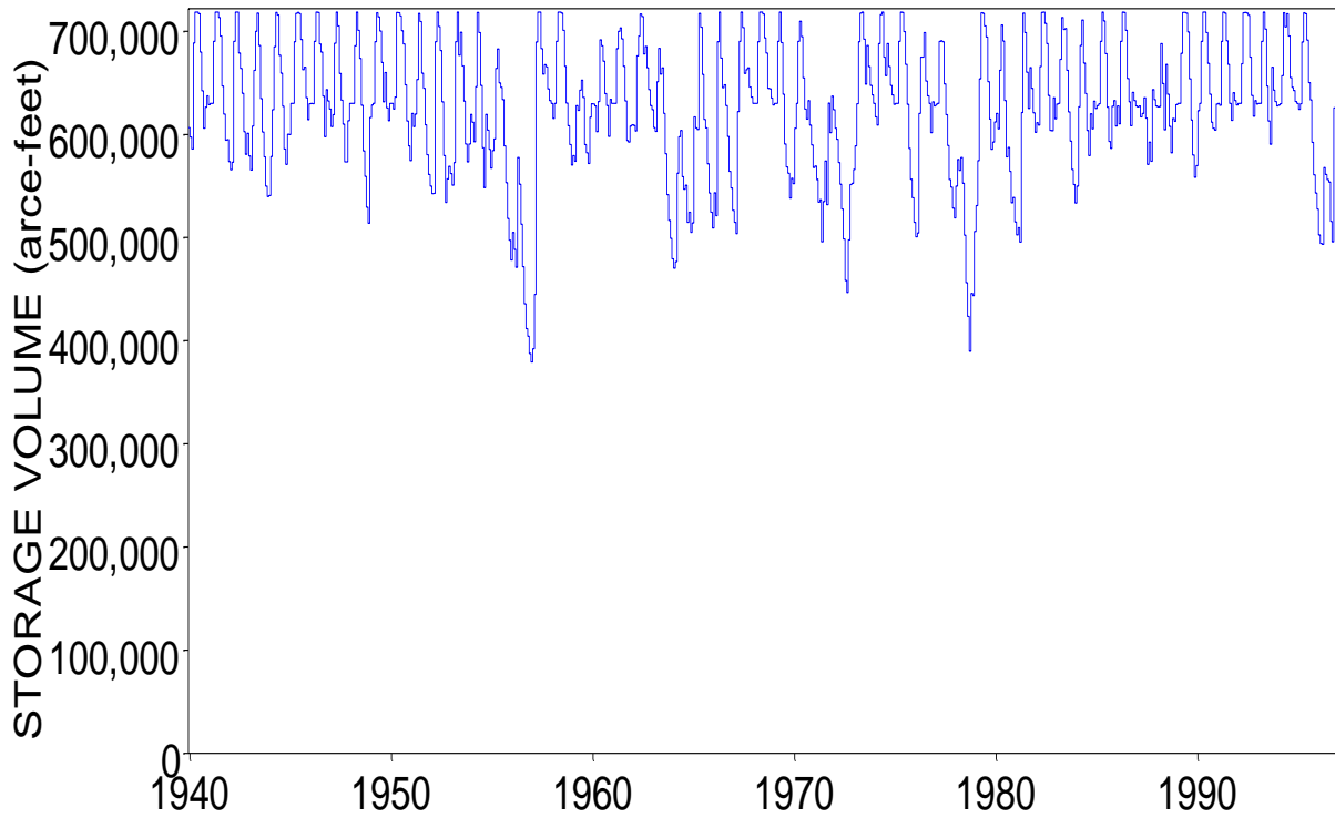
Total Storage all Reservoirs in the Sulphur River Basin
