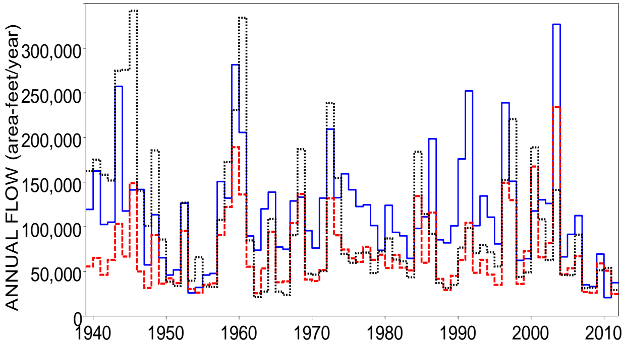
Naturalized (blue solid), Regulated (red dashed), and Observed (black dotted) 2-Month Minimum Annual Flows for Colorado River at Columbus
