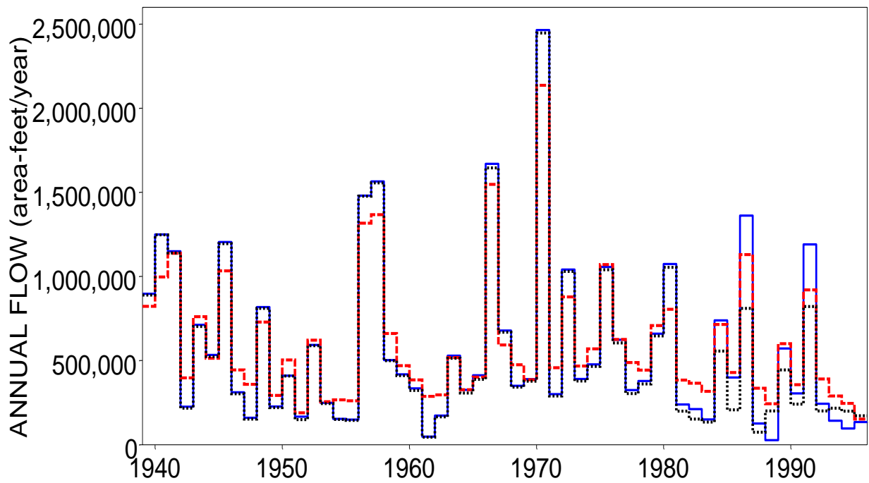
Naturalized (blue solid), Regulated (red dashed), and Observed (black dotted) Annual Flows for Nueces River at Three Rivers
