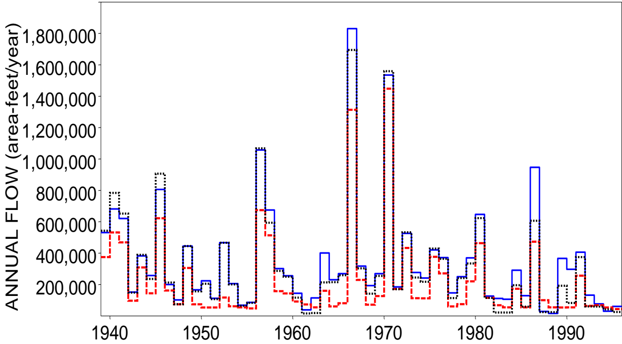
Naturalized (blue solid), Regulated (red dashed), and Observed (black dotted) 2-Month Maximum Annual Flows for Nueces River at Mathis
