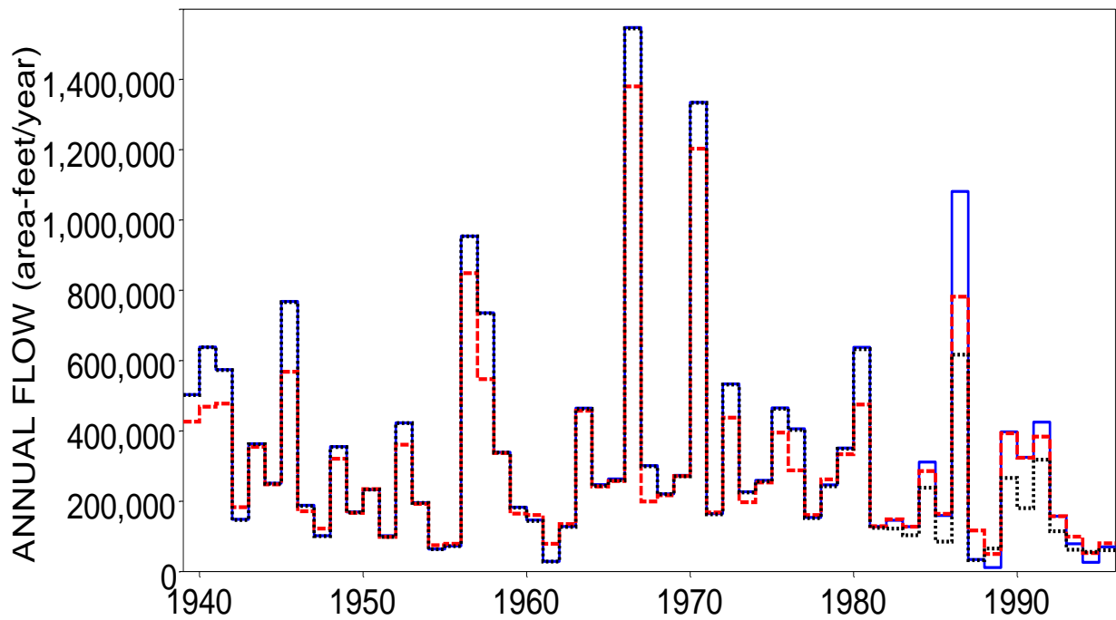
Naturalized (blue solid), Regulated (red dashed), and Observed (black dotted) 2-Month Maximum Annual Flows for Nueces River at Three Rivers
