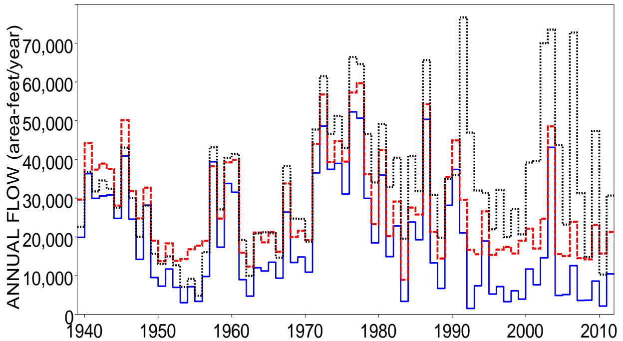
Naturalized (blue solid), Regulated (red dashed) and Observed (black dotted) 2-Month Minimum Annual Flows for San Antonio River at Goliad
