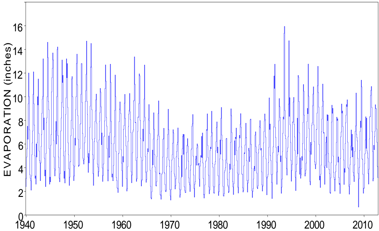
Monthly Evaporation for Quadrangle 1008
