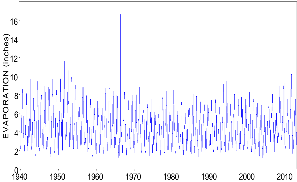
Monthly Evaporation for Quadrangle 710
