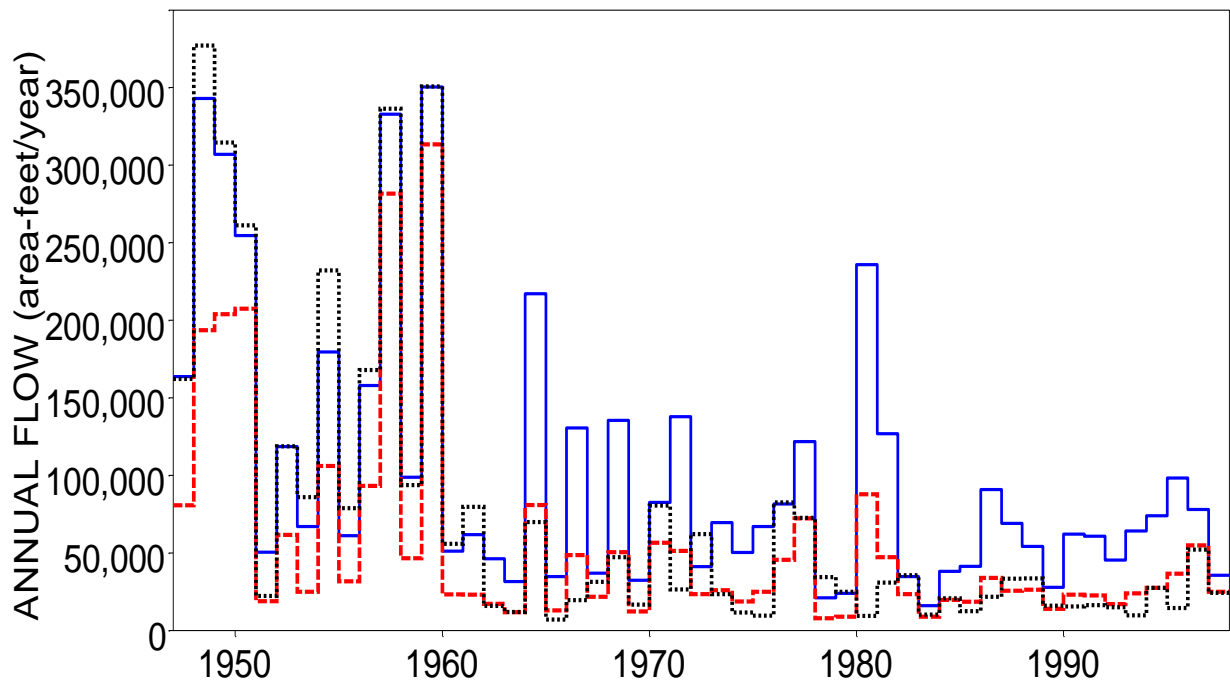
Naturalized (blue solid), Regulated (red dashed), and Observed (black dotted) 2-Month Maximum Annual Flows for Canadian River near Canadian
