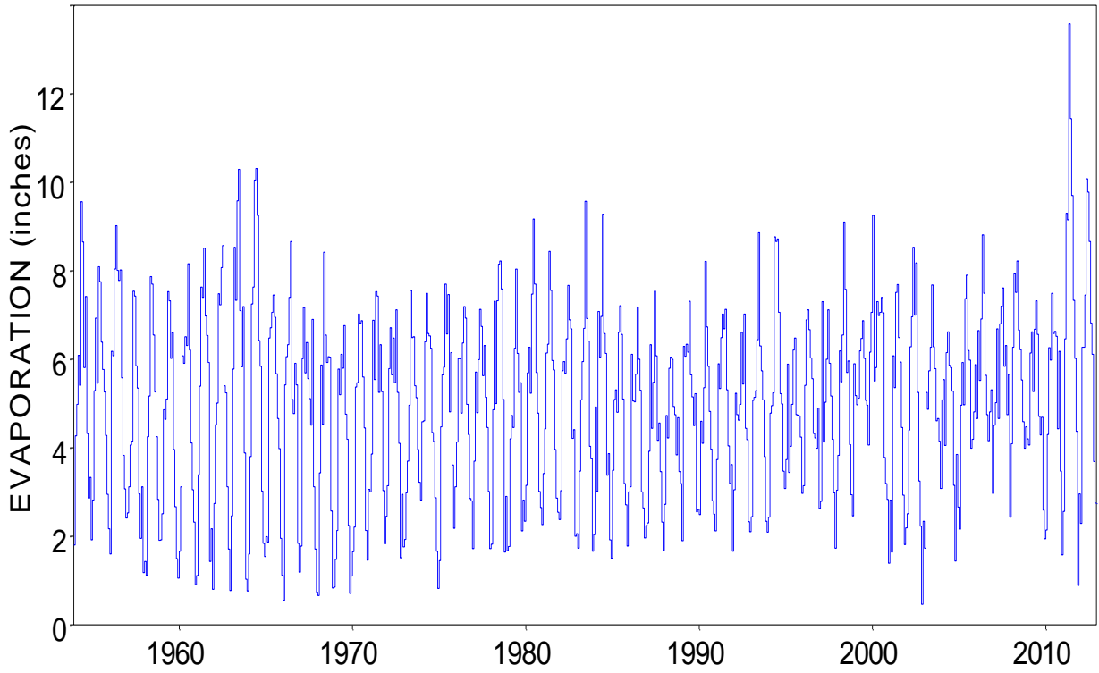
Monthly Evaporation for Quadrangle 104
