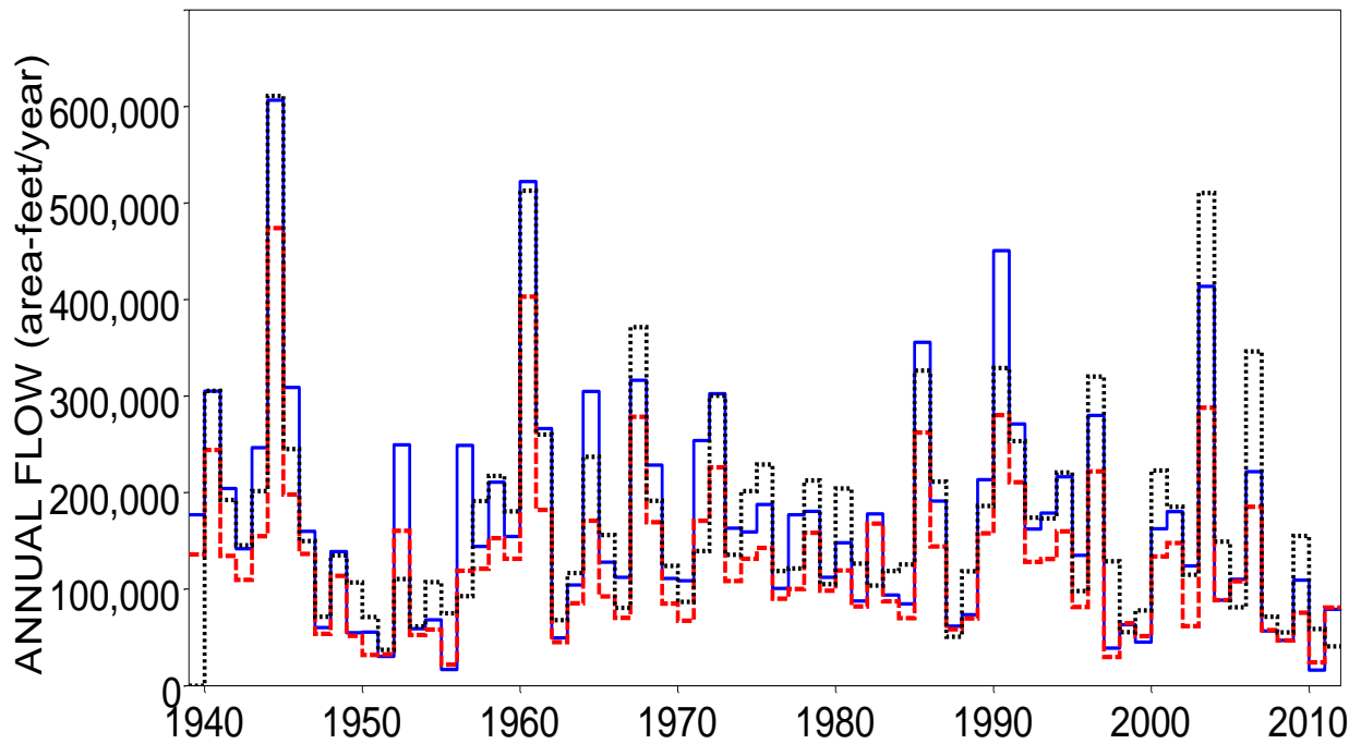
Naturalized (blue solid) and regulated (red dashed) Observed (black dotted) 2-Month Minimum Annual Flows for Brazos River at Richmond
