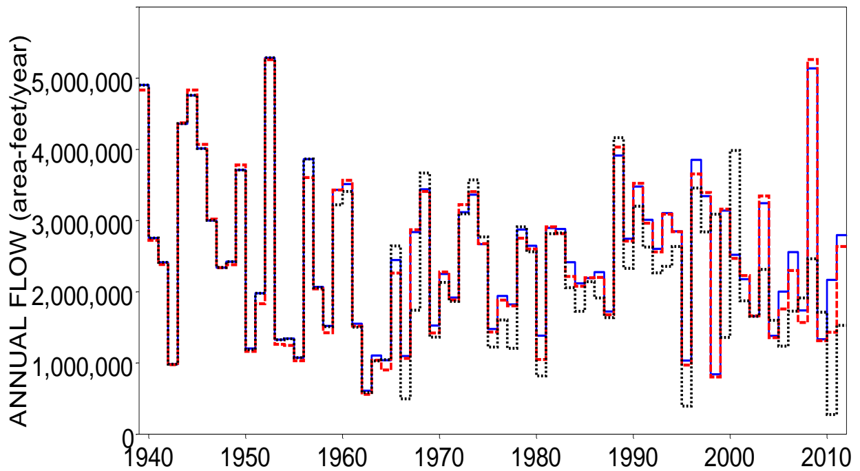
Naturalized (blue solid), Regulated (red dashed), and Observed (black dotted) 2-Month Maximum Annual Flows for Sabine River near Ruliff
