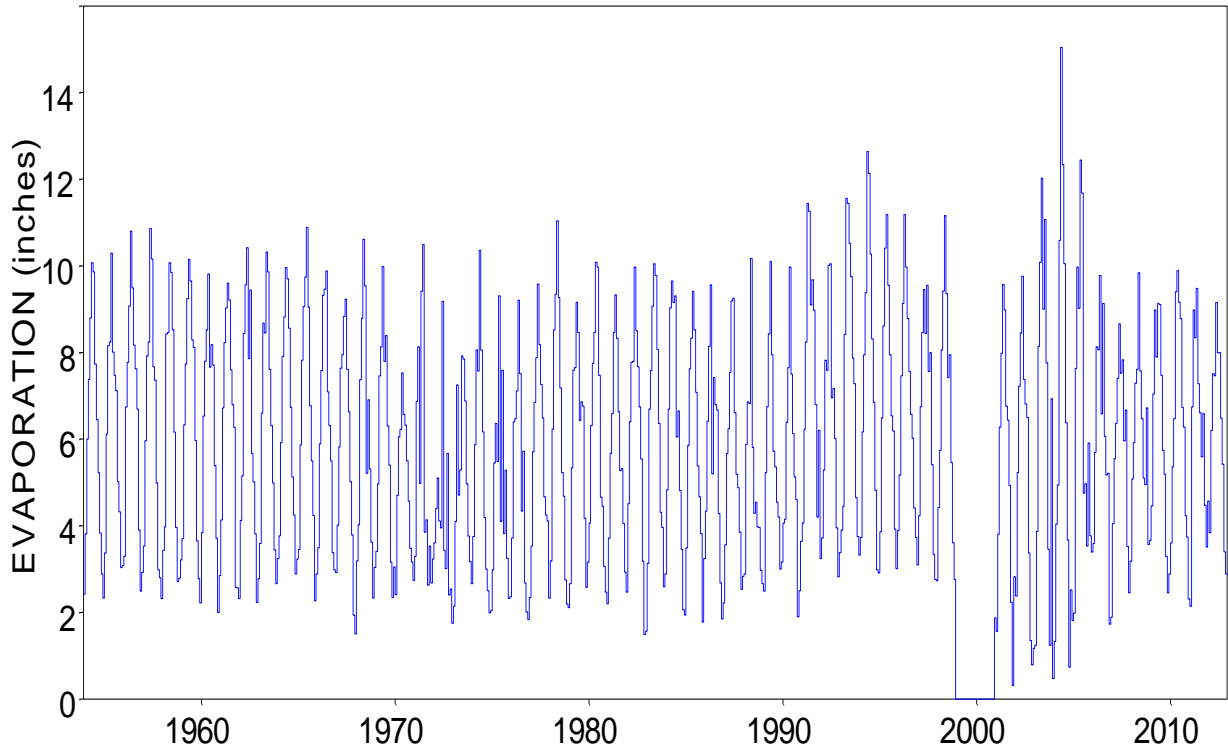
Monthly Evaporation for Quadrangle 701(missing date form 1999-2000)
