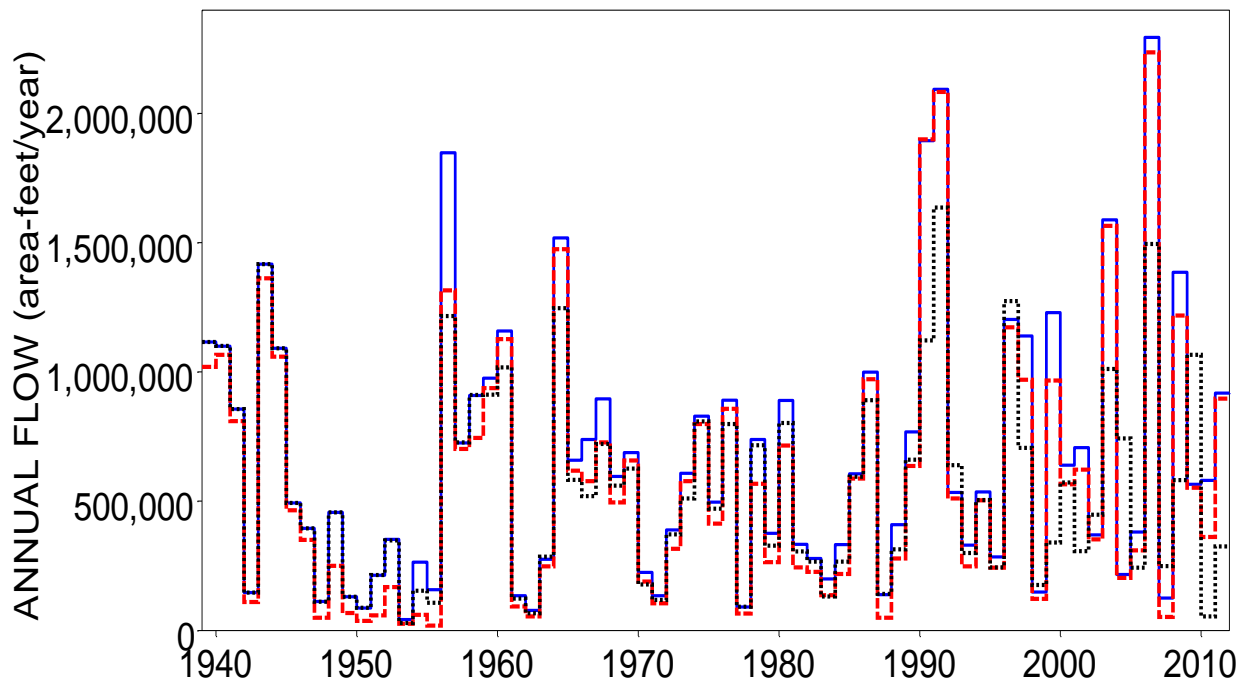
Naturalized (blue solid), Regulated (red dashed), and Observed (black dotted) 2-Month Maximum Annual Flows for Little River at Cameron
