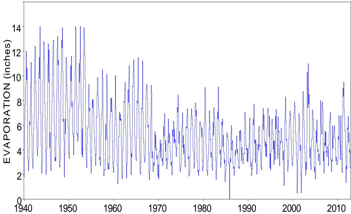
Monthly Evaporation for Quadrangle 704
