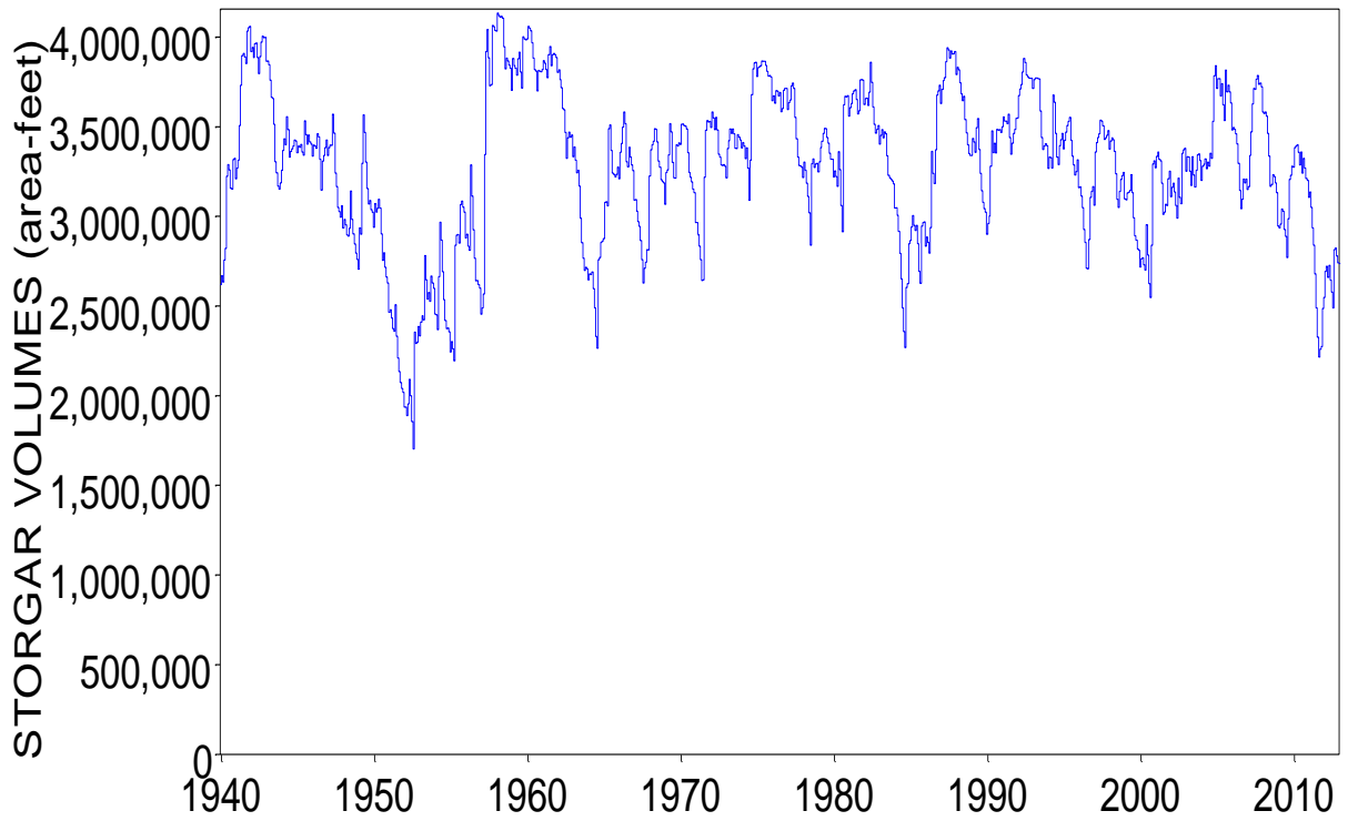
Total Storage all Reservoirs in the Colorado and Brazos-Colorado Coastal Basin
