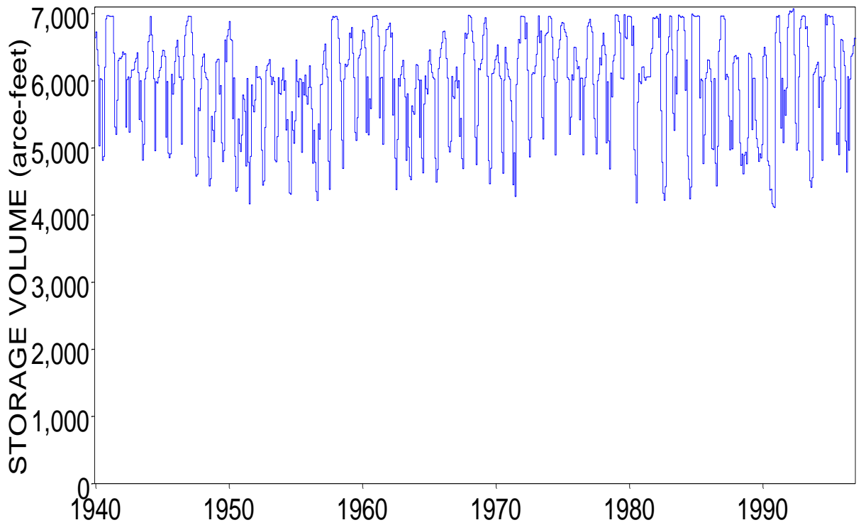
Total Storage all Reservoirs in the Colorado-Lavaca Coastal Basin
