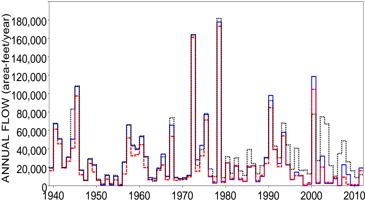
Naturalized (blue solid), Regulated (red dashed), and Observed (black dotted) 2-Month Minimum Annual Flows for Neches River near Rockland
