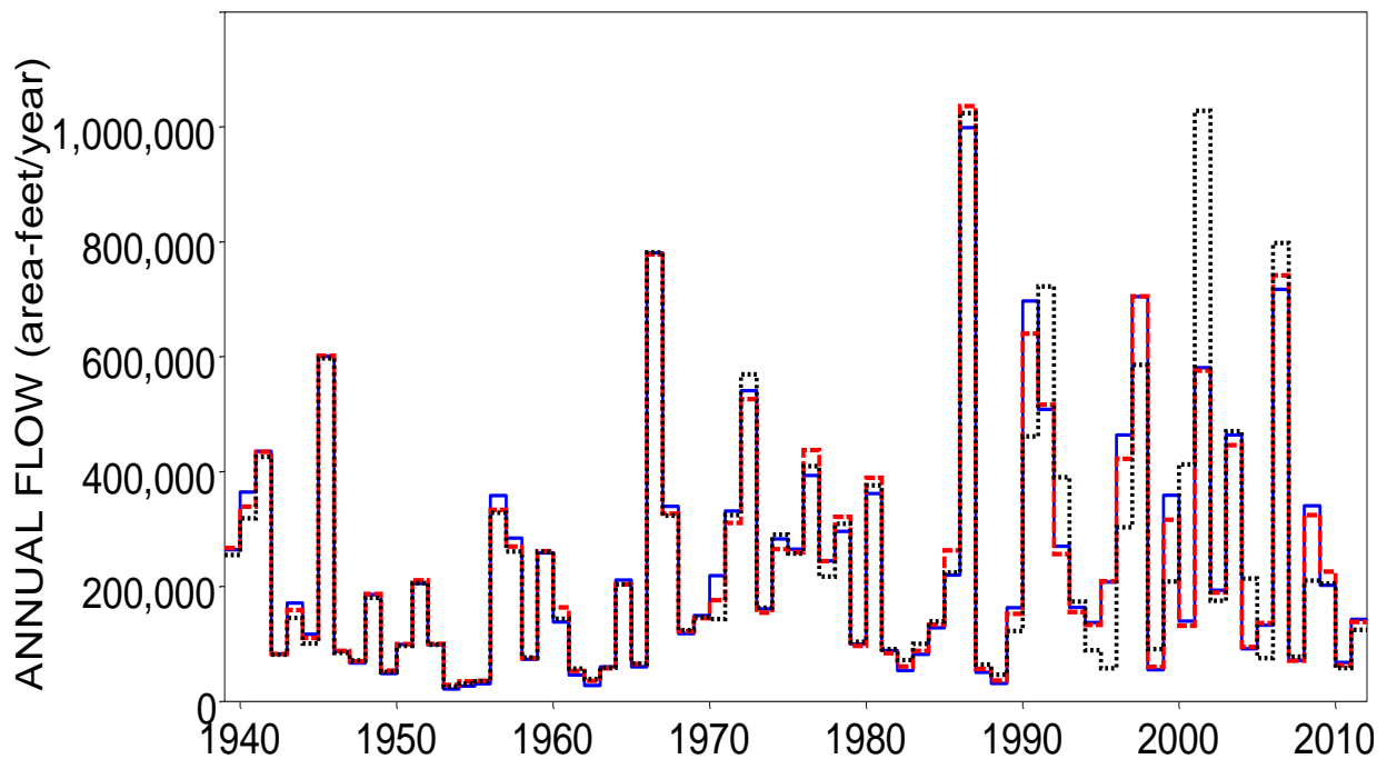
Naturalized (blue solid), Regulated (red dashed) and Observed (black dotted) 2-Month Maximum Annual Flows for San Antonio River at Goliad
