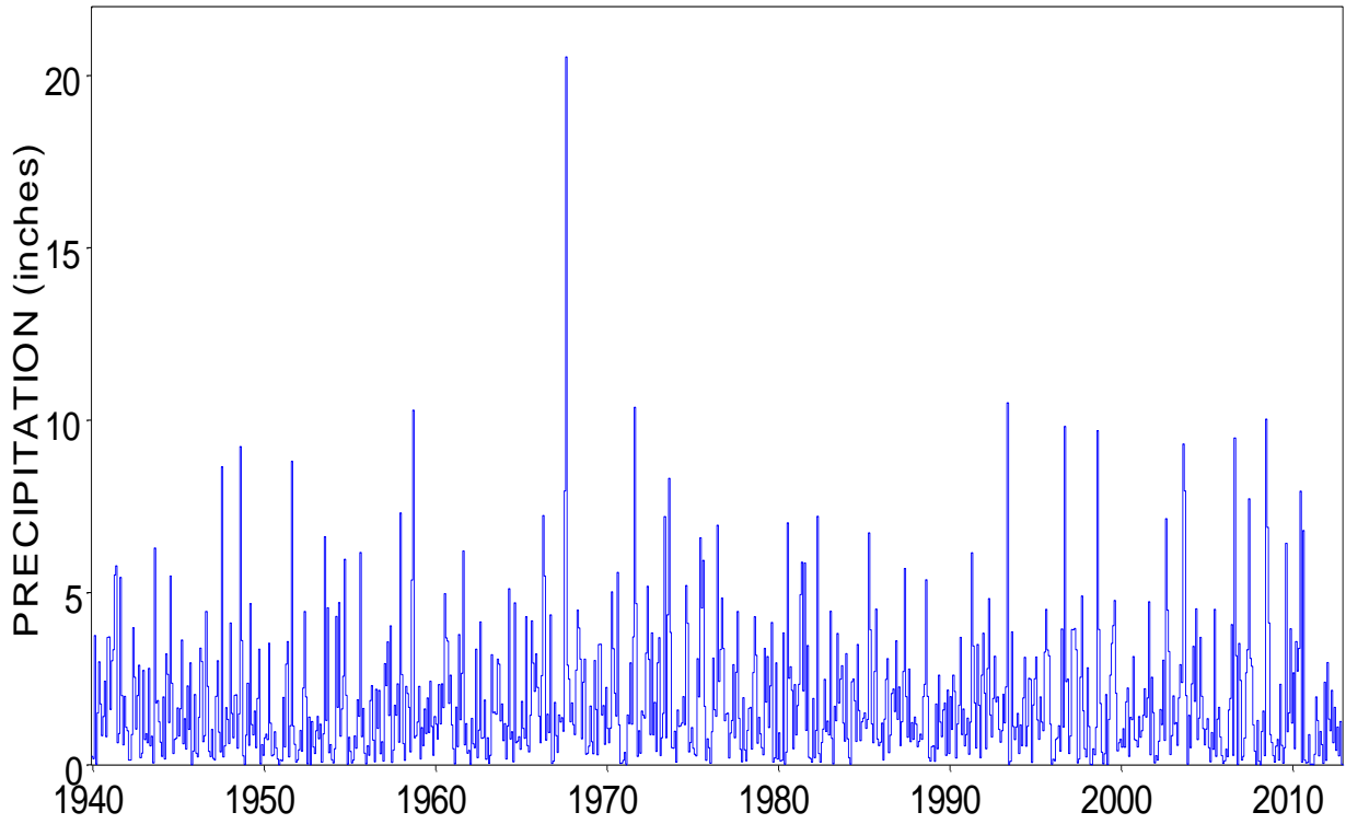
Monthly Precipitation for Quadrangle 1109
