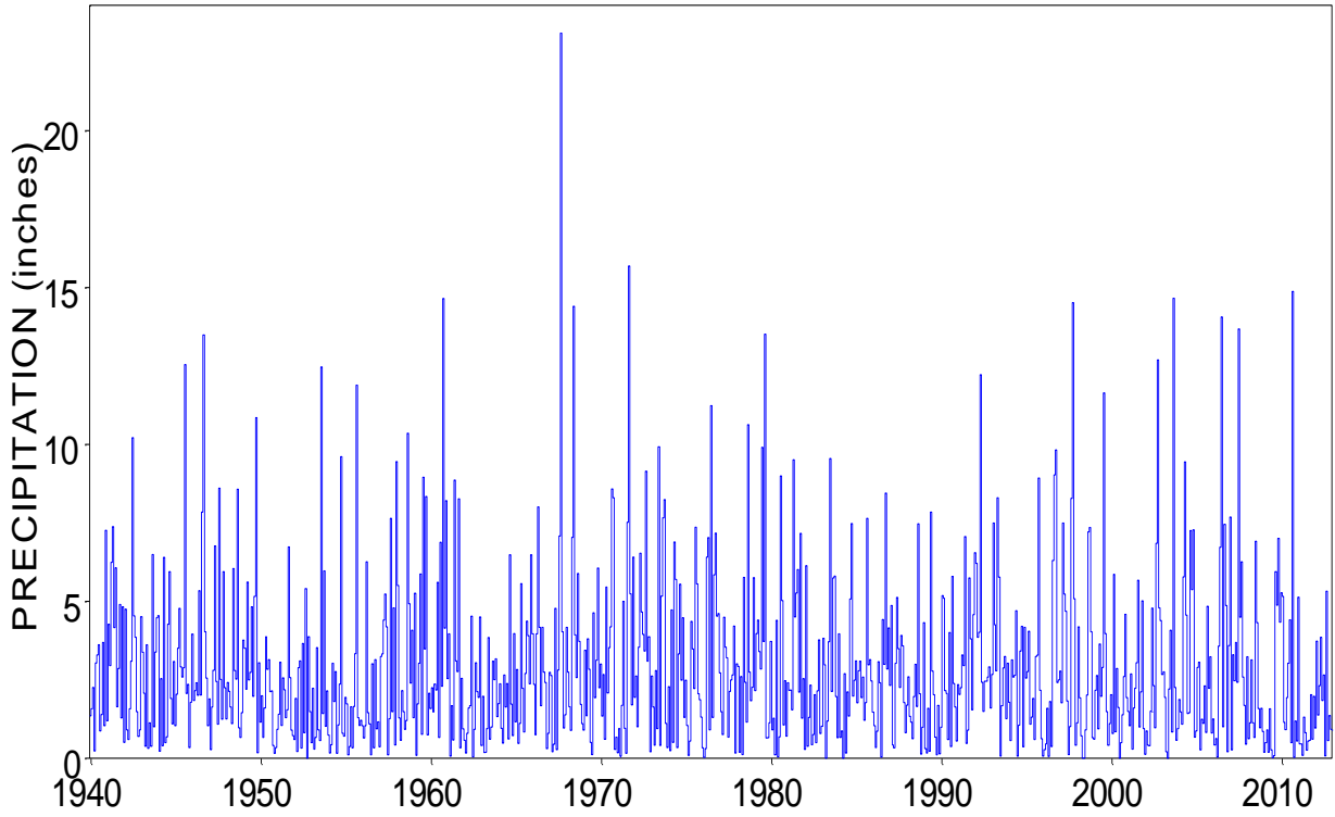
Monthly Precipitation for Quadrangle 1011
