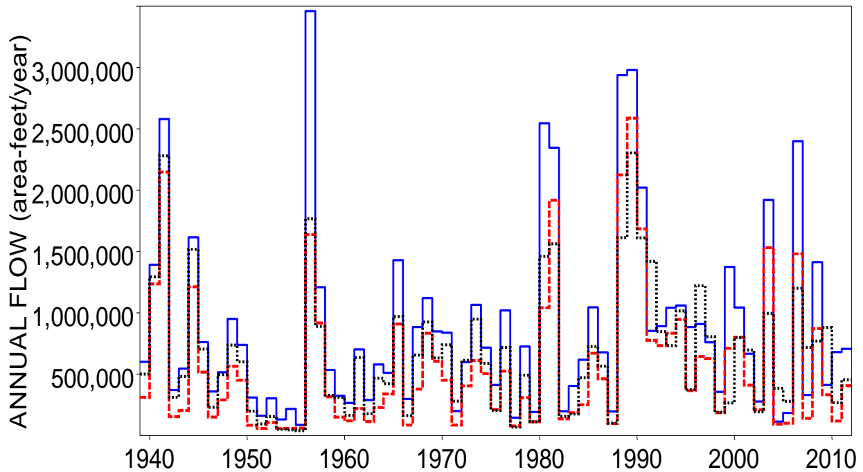
Naturalized (blue solid), Regulated (red dashed), and Observed (black dotted) 2-Month Maximum Annual Flows for Trinity River at Dallas
