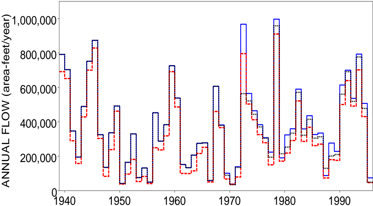
Naturalized (blue solid), Regulated (red dashed), and Observed (black dotted) Annual Flows for West Fork San Jacinto near Conroe
