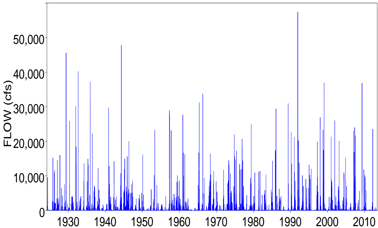
Daily Flows of Navasota River at Easterly
