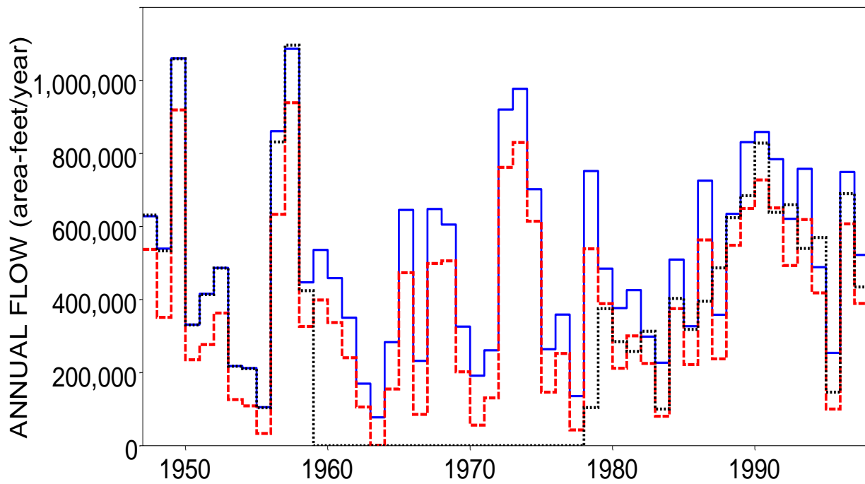
Naturalized (blue solid) and regulated (red dashed) Observed (black dotted) Annual Flows for Big Cypress Bayou at Jefferson
