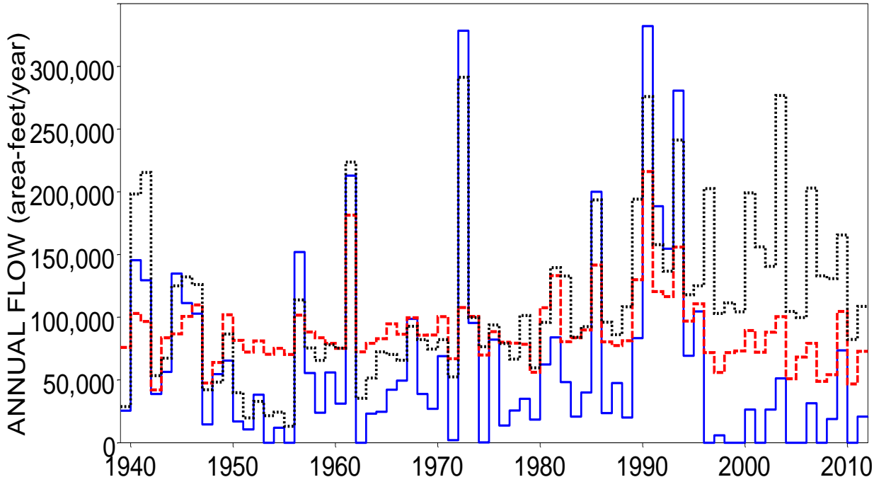
Naturalized (blue solid), Regulated (red dashed), and Observed (black dotted) 2-Month Minimum Annual Flows for Trinity River near Oakwood
