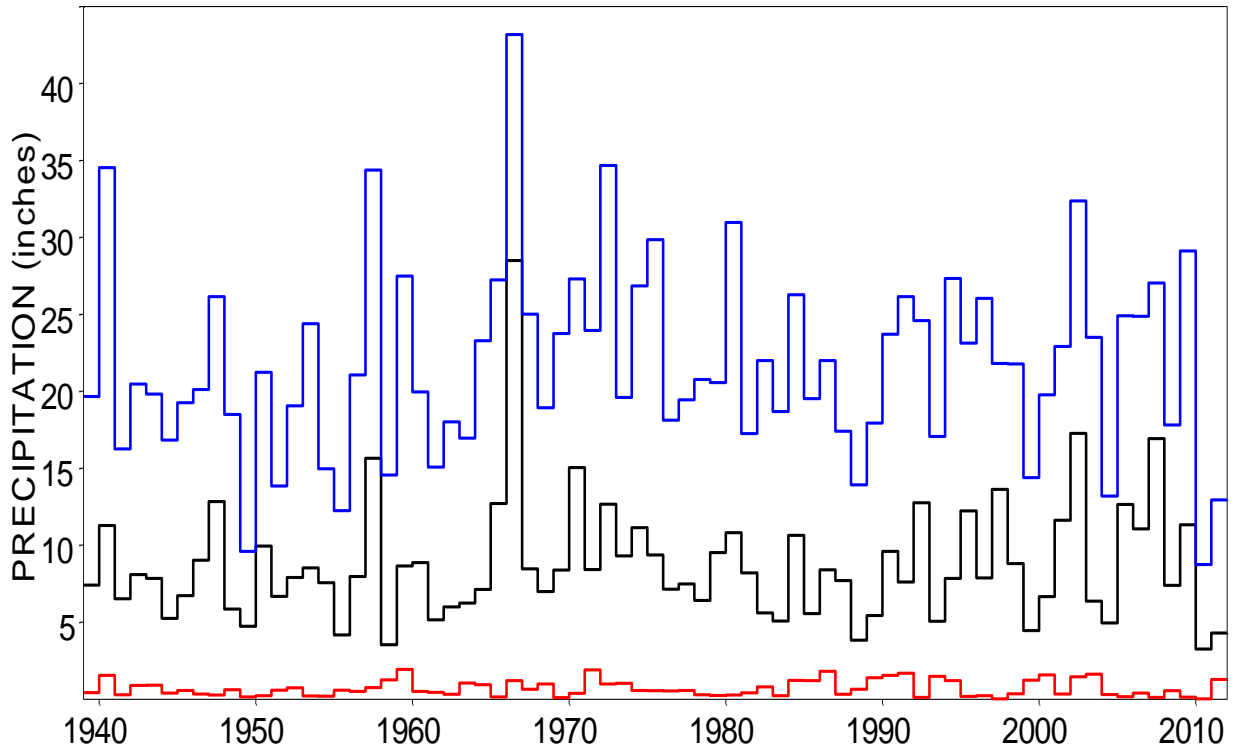
Annual Total, 2-Month Maximum, and 2-Month Minimum Precipitation for Quadrangle 1109
