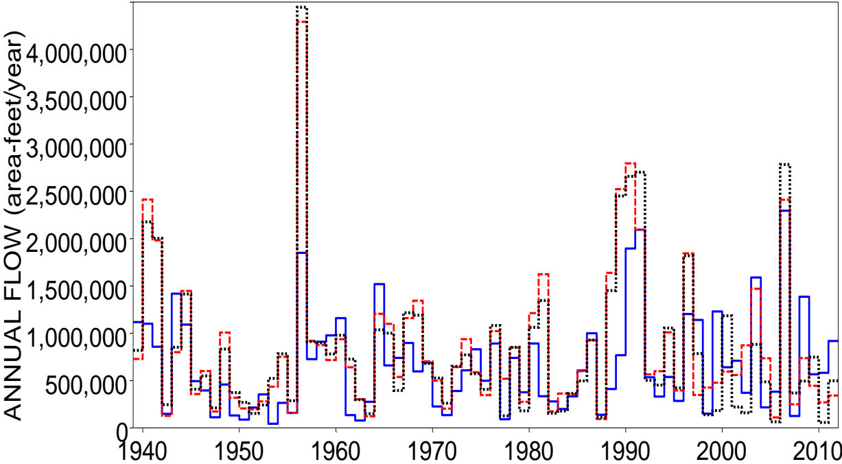
Naturalized (blue solid), Regulated (red dashed), and Observed (black dotted) 2-Month Maximum Annual Flows for Brazos River Waco
