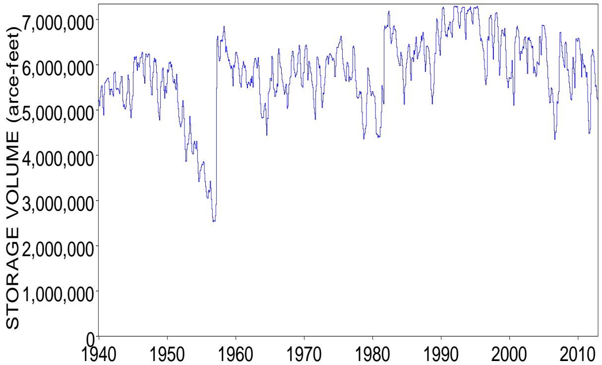
Total Storage all Reservoirs in the Trinity River Basin
