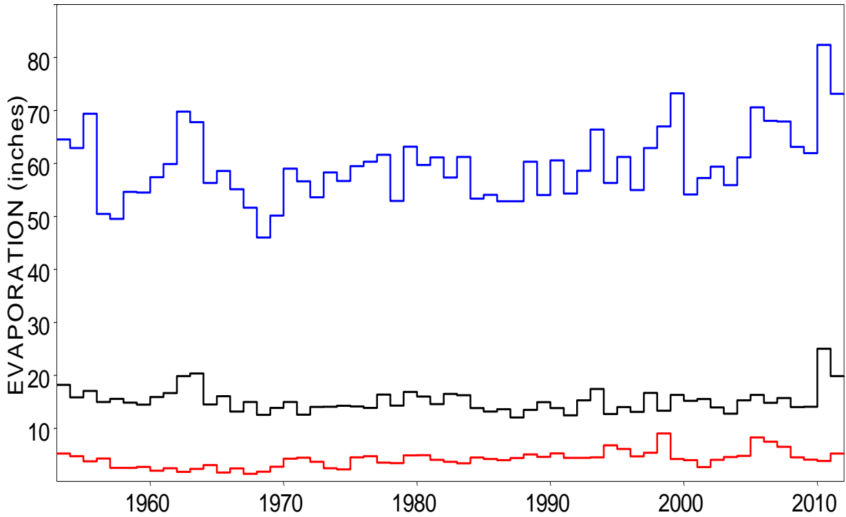
Annual Total, 2-Month Maximum, and 2-Month Minimum Evaporation for Quadrangles 104
