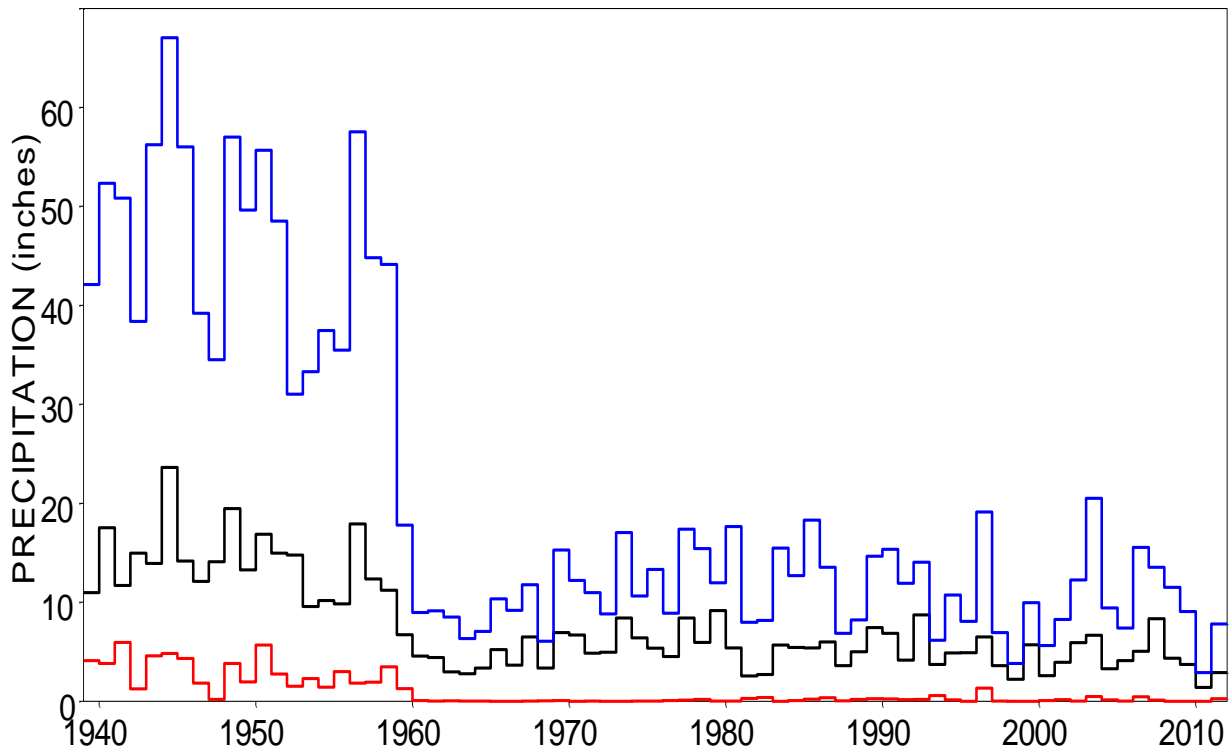
Annual Total, 2-Month Maximum, and 2-Month Minimum Precipitation for Quadrangle 803
