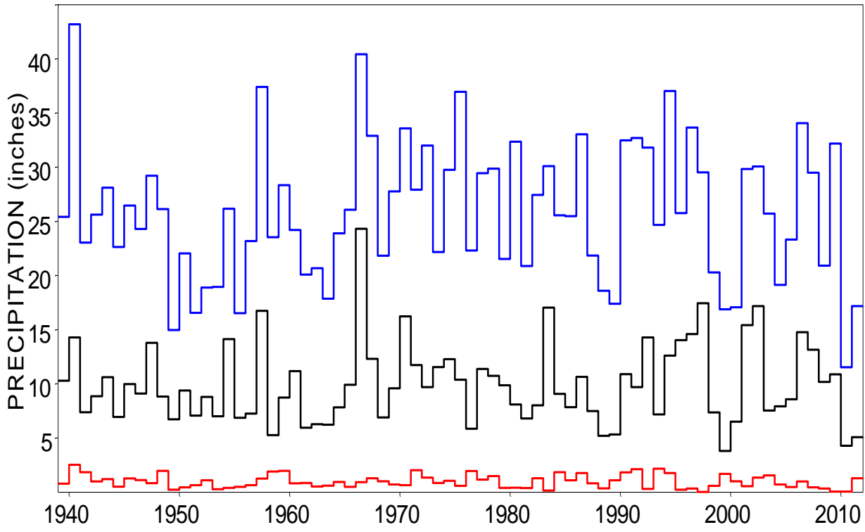
Annual Total, 2-Month Maximum, and 2-Month Minimum Precipitation for Quadrangle 1110
