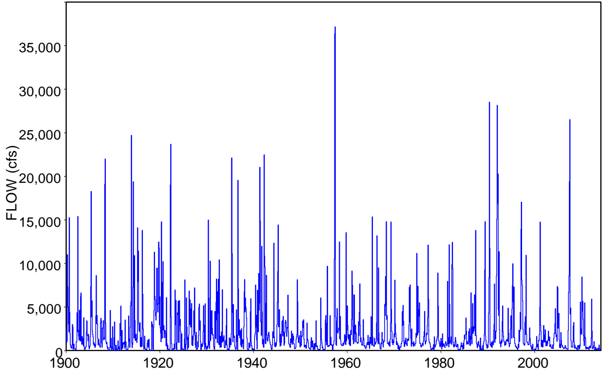
Monthly Flows of the Brazos River at the Gage at Waco
