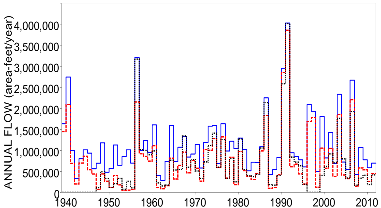
Naturalized (blue solid), Regulated (red dashed), and Observed (black dotted) 2-Month Maximum Annual Flows for Colorado River near Bay City
