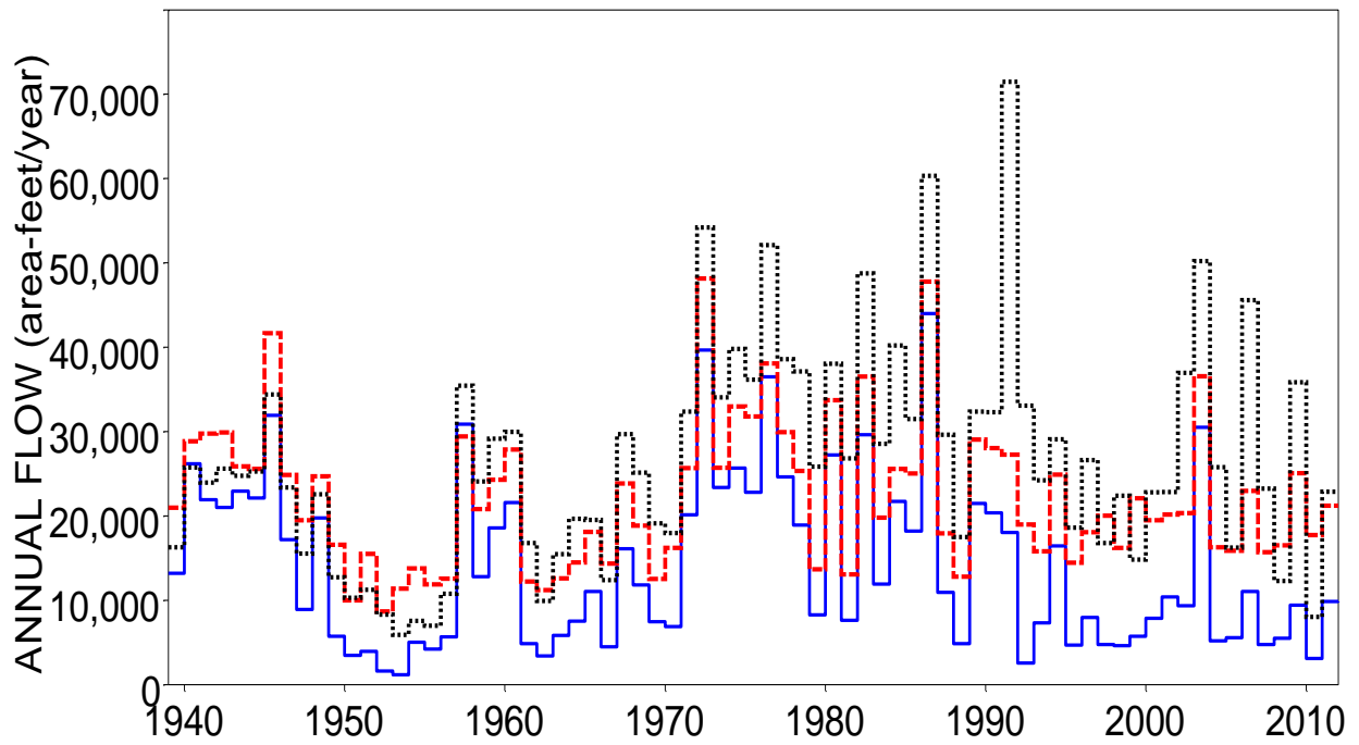
Naturalized (blue solid), Regulated (red dashed) and Observed (black dotted) 2-Month Minimum Annual Flows for San Antonio River at Falls City
