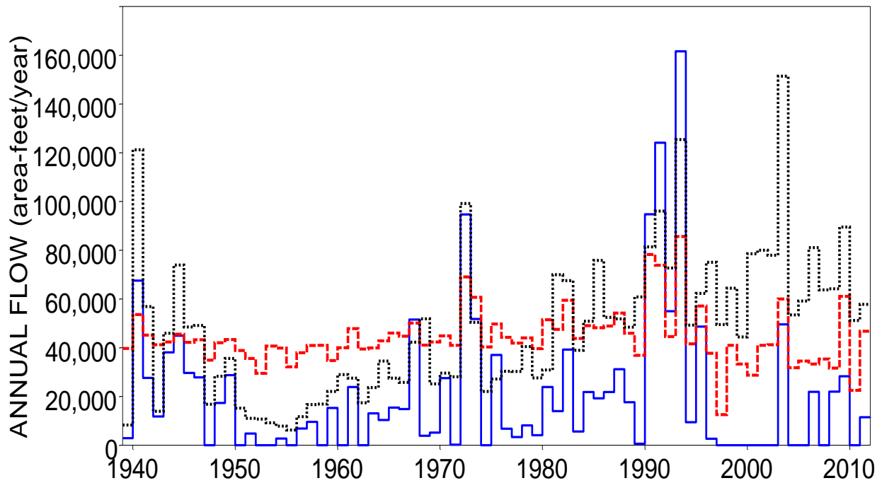
Naturalized (blue solid), Regulated (red dashed), and Observed (black dotted) 2-Month Minimum Annual Flows for Trinity River at Dallas
