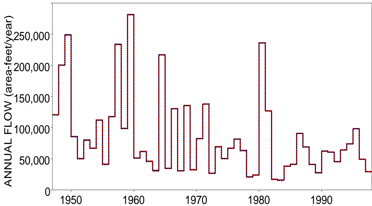
Naturalized (blue solid), Regulated (red dashed), and Observed (black dotted) 2-Month Maximum Annual Flows for Canadian River near Amarillo
