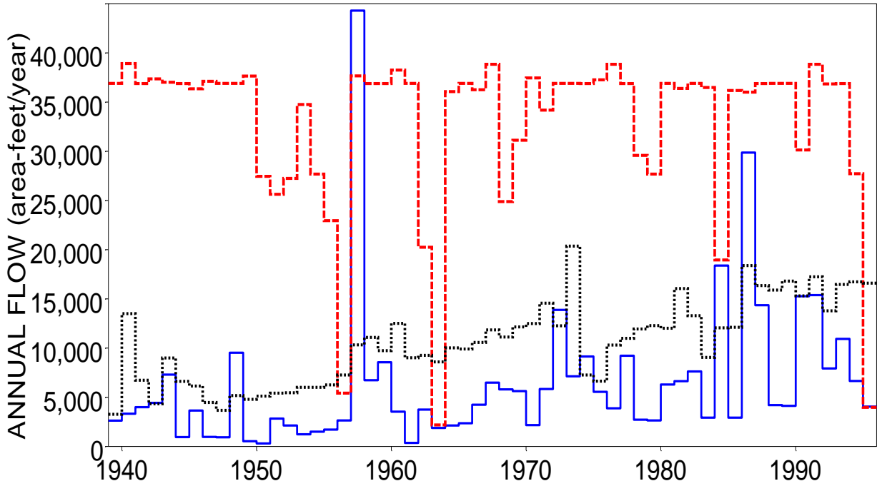
Naturalized (blue solid), Regulated (red dashed), and Observed (black dotted) 2-Month Minimum Annual Flows for Nueces River at Mathis
