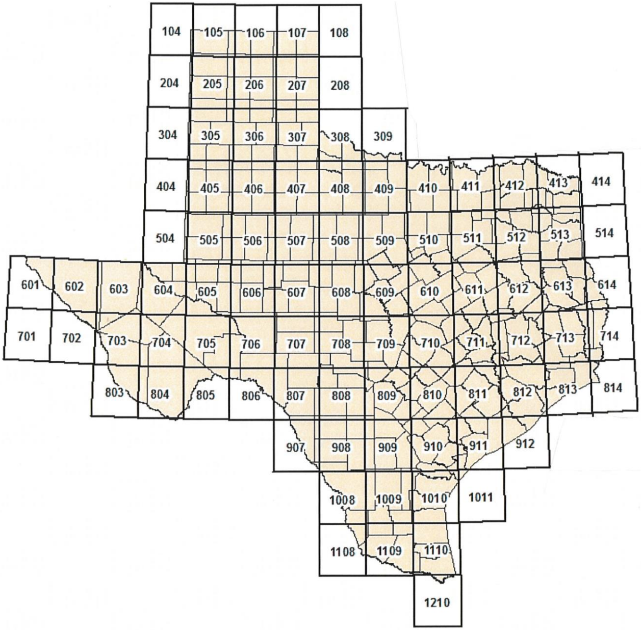
Figure 3.1 Grid of 92 One Degree Quadrangles Encompassing Texas
