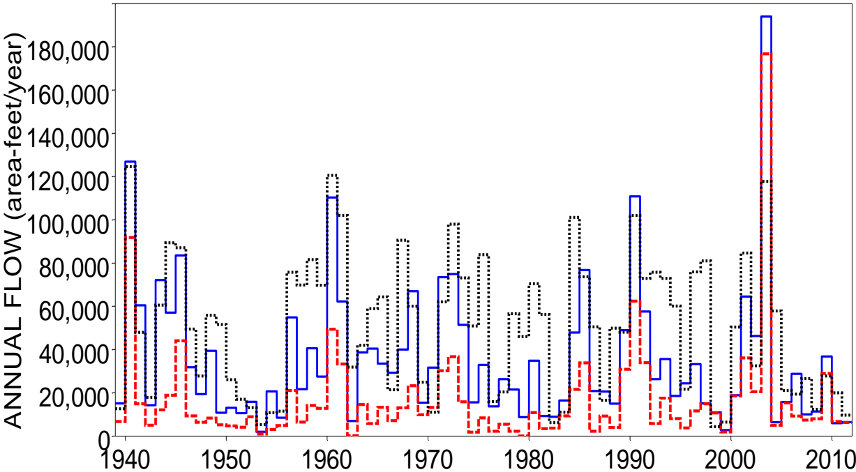
Naturalized (blue solid), Regulated (red dashed), and Observed (black dotted) 2-Month Minimum Annual Flows for Brazos River Waco
