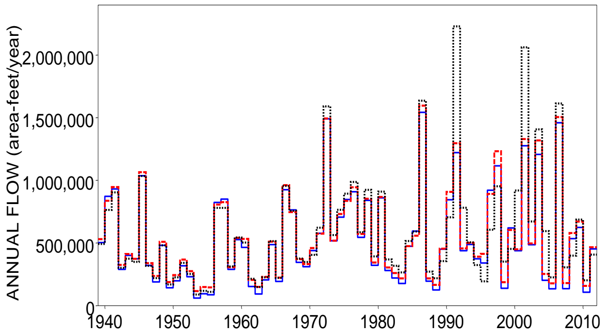
Naturalized (blue solid), Regulated (red dashed) and Observed Annual Flows for San Antonio River at Goliad
