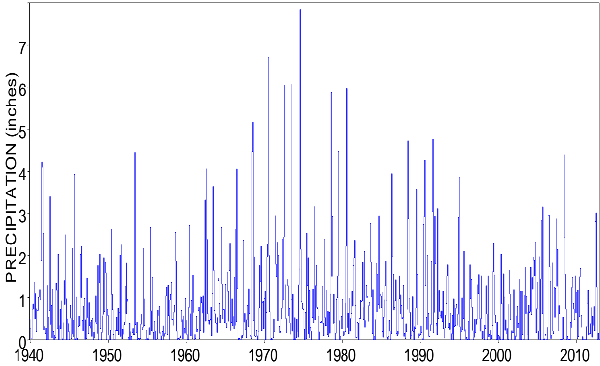
Monthly Precipitation for Quadrangle 701
