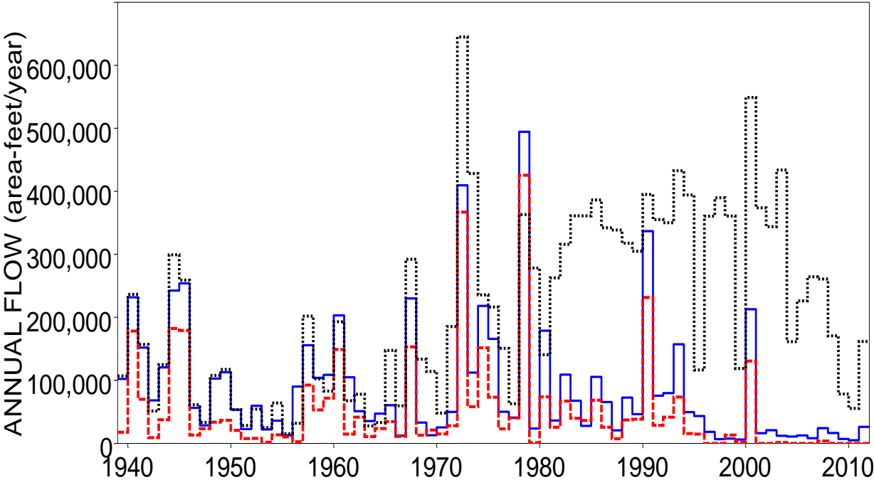
Naturalized (blue solid), Regulated (red dashed), and Observed (black dotted) 2-Month Minimum Annual Flows for Neches River near Evansdale
