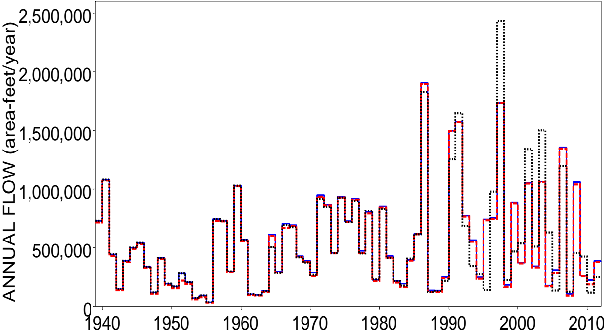
Naturalized (blue solid), Regulated (red dashed) and Observed (black dotted) 2-Month Maximum Annual Flows for Guadalupe River at Victoria
