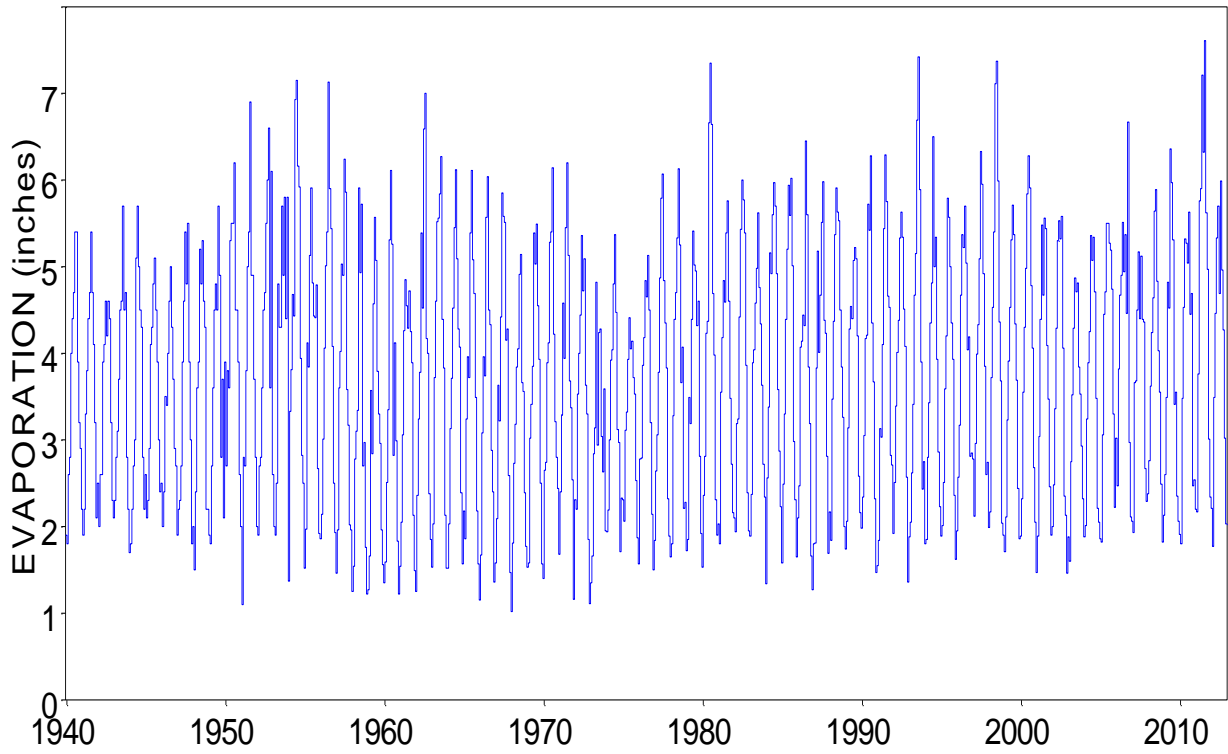
Monthly Evaporation for Quadrangle 713
