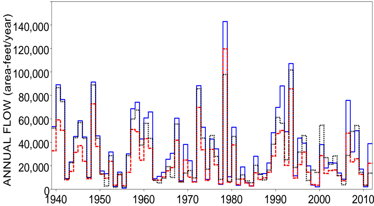
Naturalized (blue solid), Regulated (red dashed), and Observed (black dotted) 2-Month Minimum Annual Flows for Sabine River near Beckville
