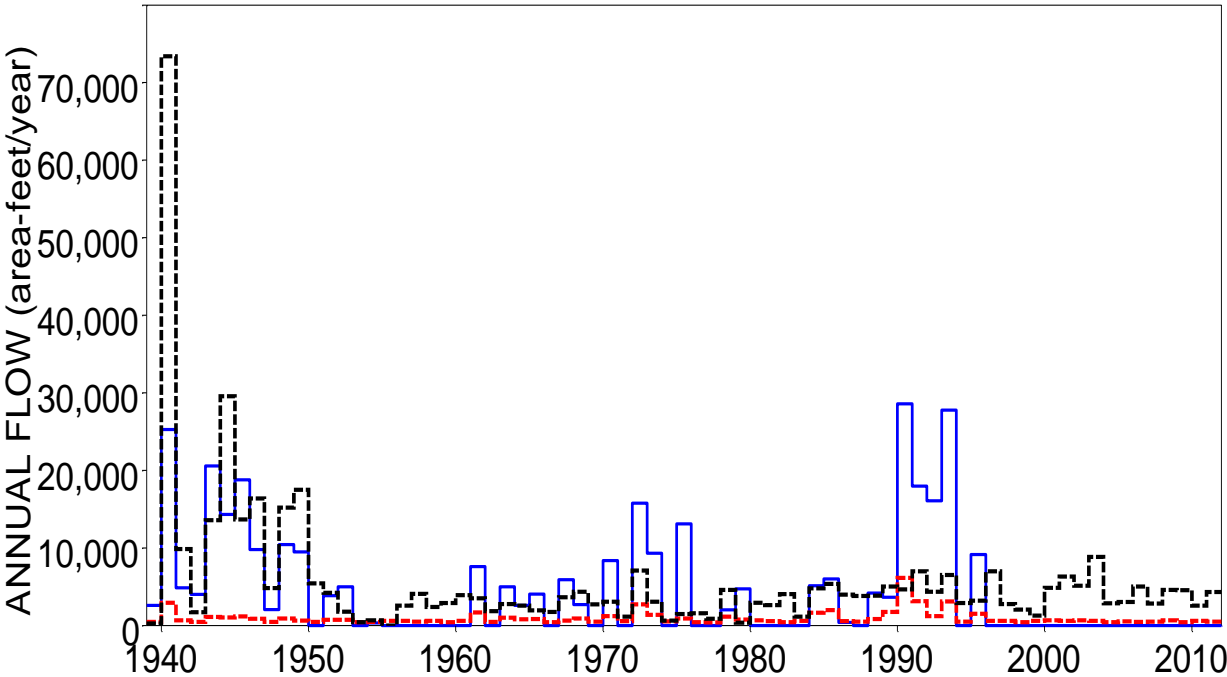
Naturalized (blue solid), Regulated (red dashed), and Observed (black dotted) 2-Month Minimum Annual Flows for West Fork Trinity at Fort Worth
