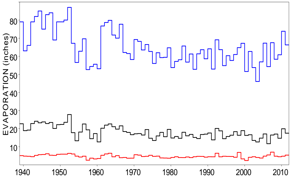
Annual Total, 2-Month Maximum, and 2-Month Minimum Evaporation for Quadrangles 707
