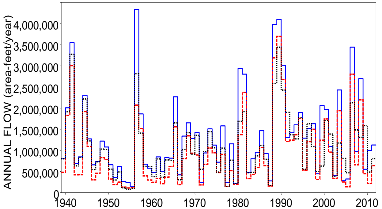
Naturalized (blue solid), Regulated (red dashed), and Observed (black dotted) 2-Month Maximum Annual Flows for Trinity River near Rosser
