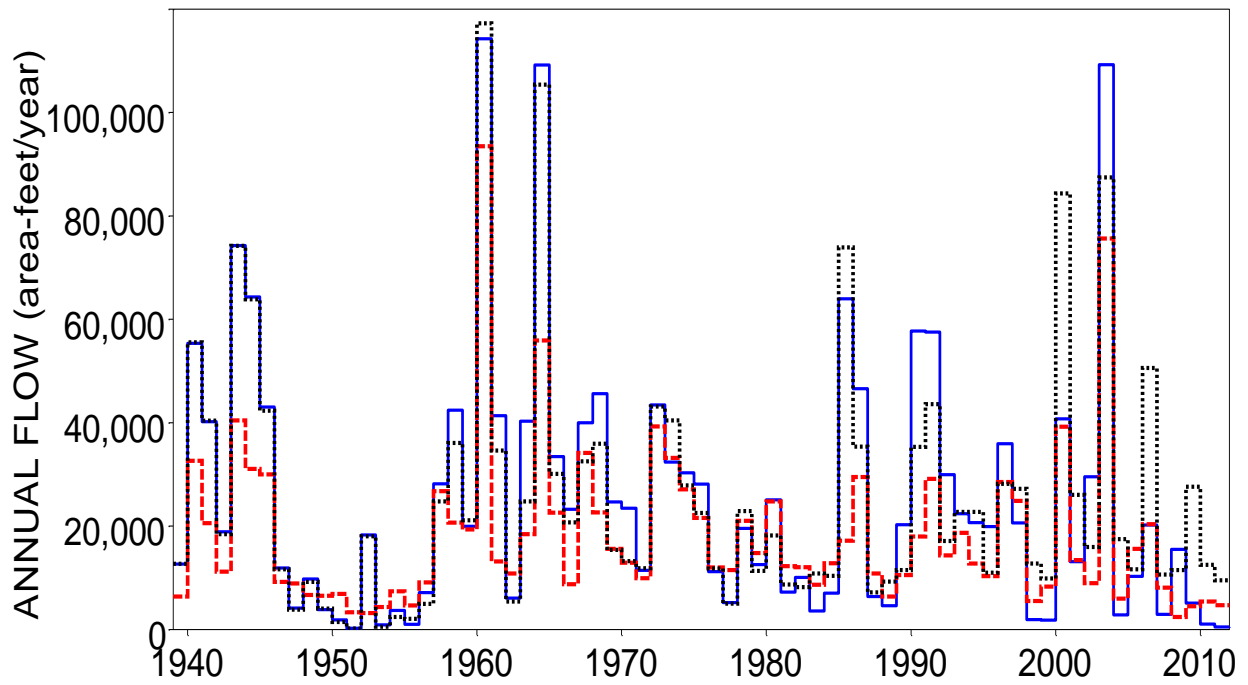
Naturalized (blue solid), Regulated (red dashed), and Observed (black dotted) 2-Month Minimum Annual Flows for Little River at Cameron
