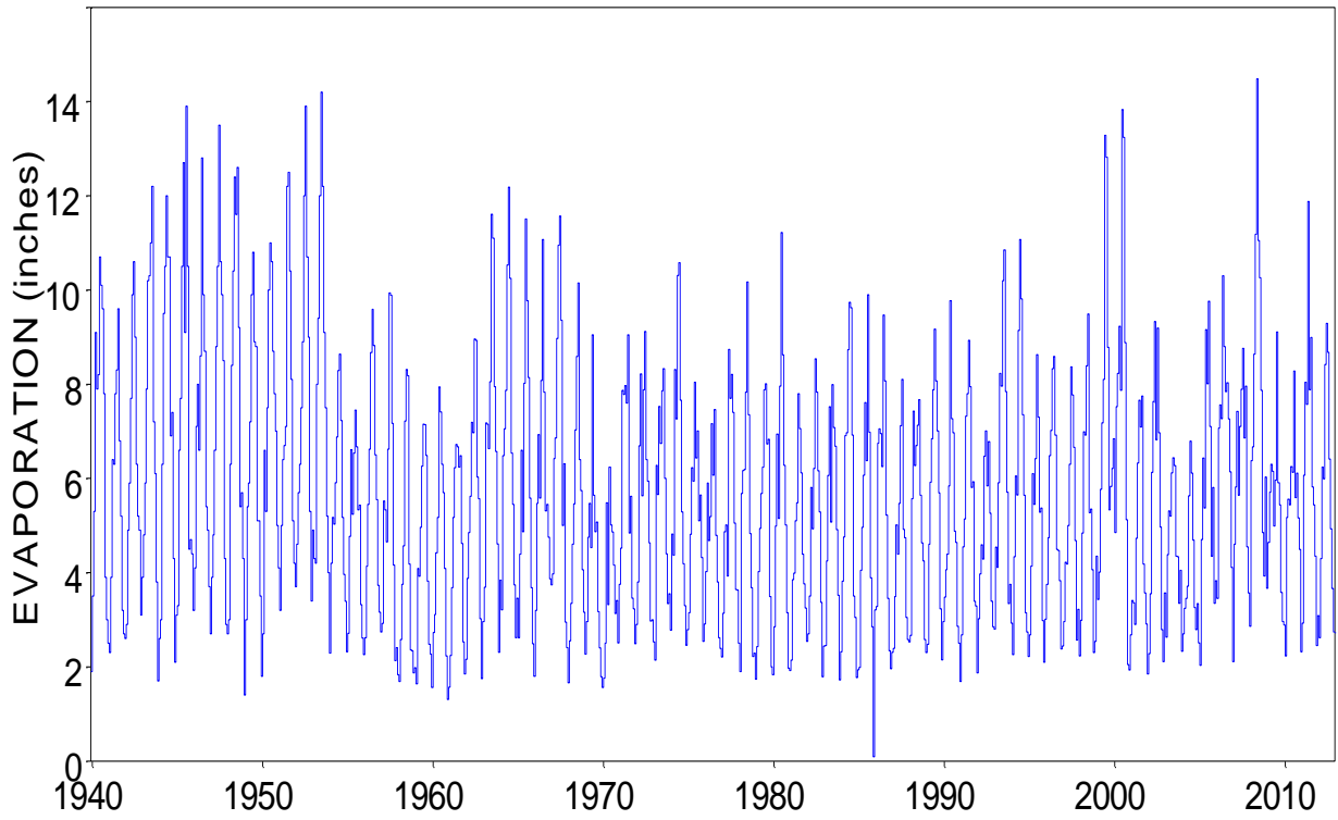
Monthly Evaporation for Quadrangle 706
