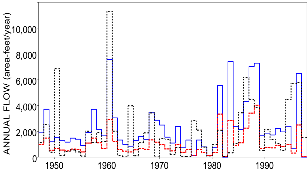
Naturalized (blue solid), Regulated (red dashed), and Observed (black dotted) 2-Month Minimum Annual Flows for Canadian River near Canadian
