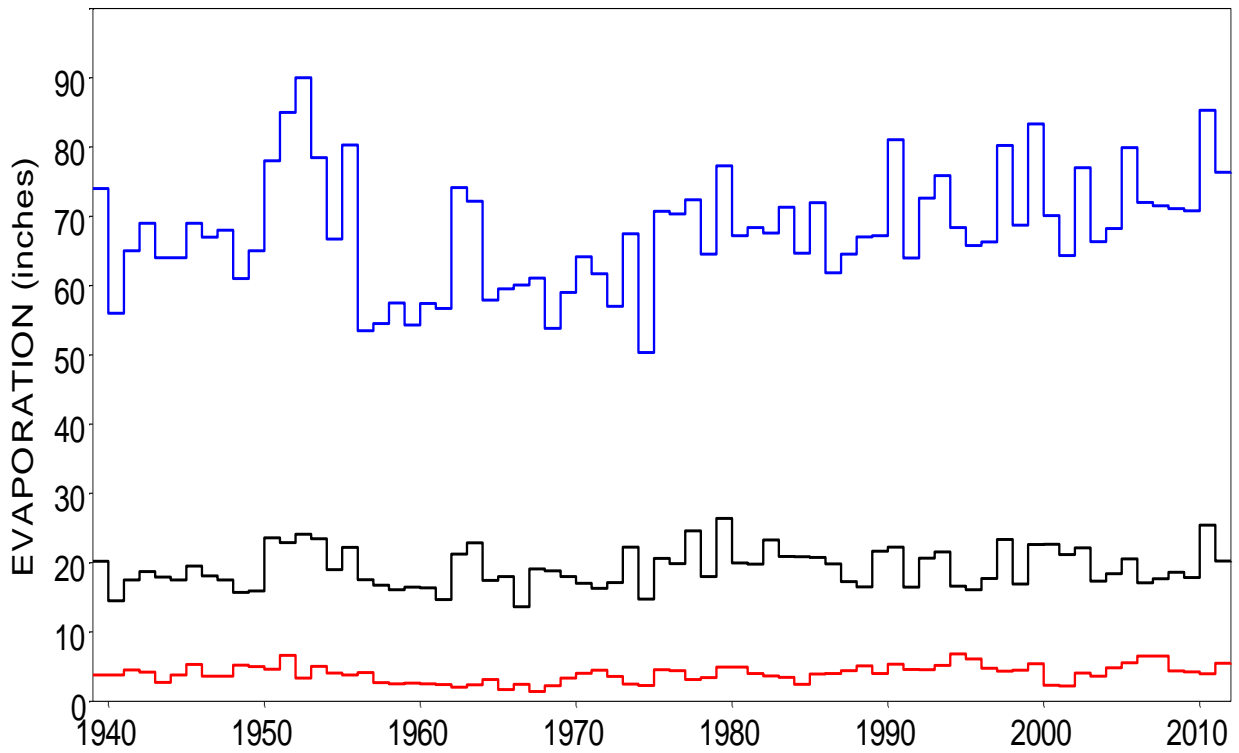
Annual Total, 2-Month Maximum, and 2-Month Minimum Evaporation for Quadrangles 106
