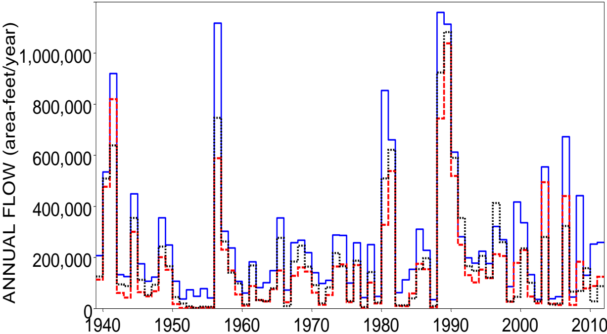
Naturalized (blue solid), Regulated (red dashed), and Observed (black dotted) 2-Month Maximum Annual Flows for West Fork Trinity at Fort Worth
