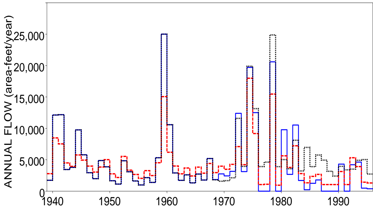
Naturalized (blue solid) and regulated (red dashed) Observed (black dotted) 2-Month Minimum Annual Flows for West Fork San Jacinto near Conroe
