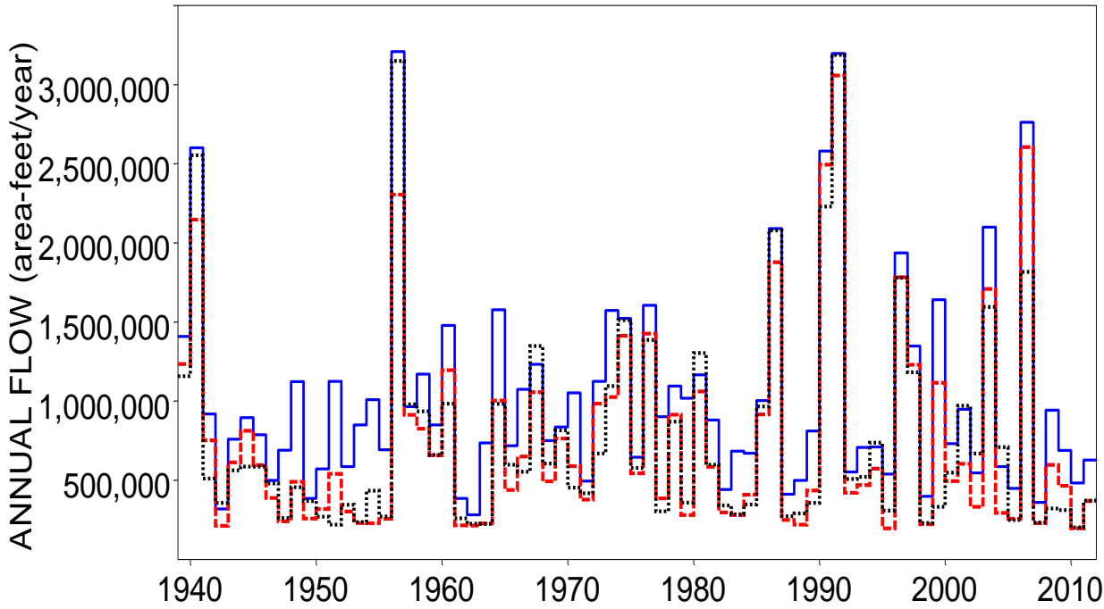
Naturalized (blue solid), Regulated (red dashed), and Observed (black dotted) 2-Month Maximum Annual Flows for Colorado River at Columbus
