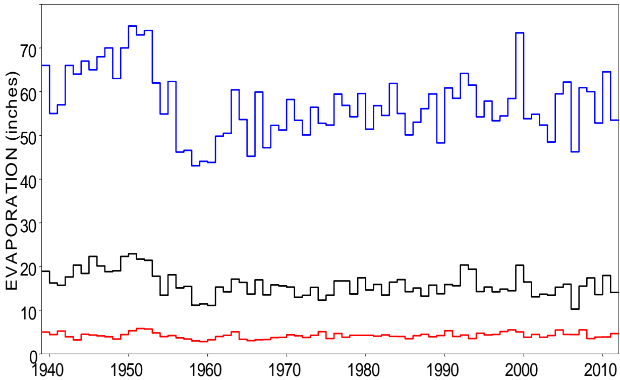
Annual Total, 2-Month Maximum, and 2-Month Minimum Evaporation for Quadrangles 709
