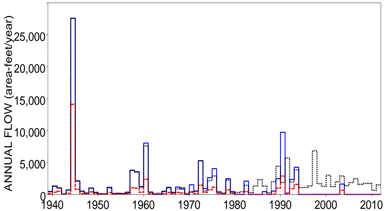
Naturalized (blue solid), Regulated (red dashed), and Observed (black dotted) 2-Month Minimum Annual Flows for Navasota River at Easterly
