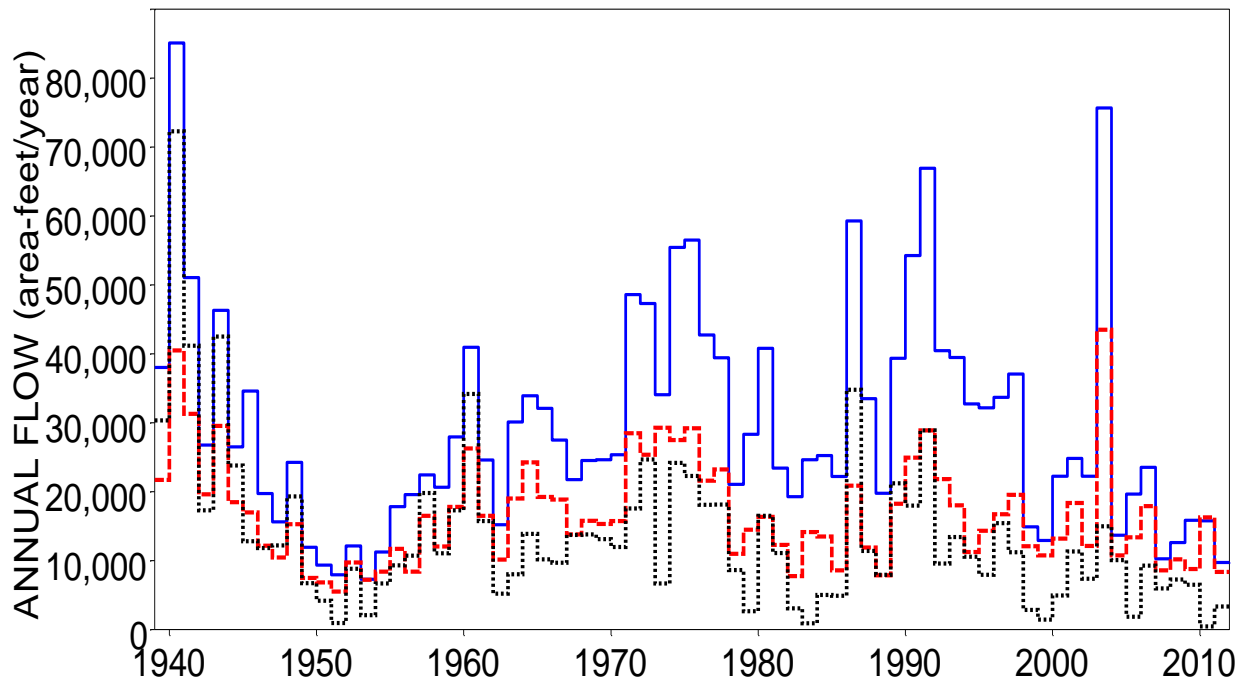
Naturalized (blue solid), Regulated (red dashed), and Observed (black dotted) 2-Month Minimum Annual Flows for Colorado River at San Saba gage (F10000)
