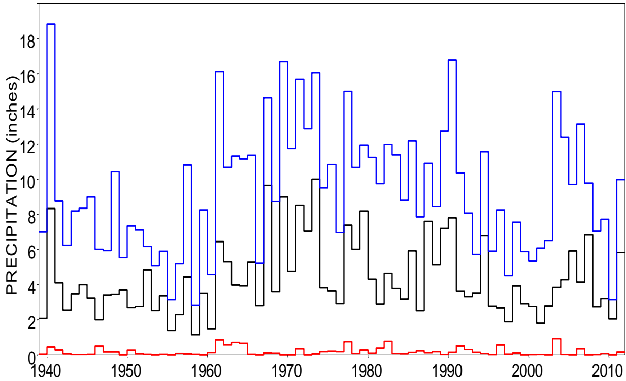
Annual Total, 2-Month Maximum, and 2-Month Minimum Precipitation for Quadrangle 701
