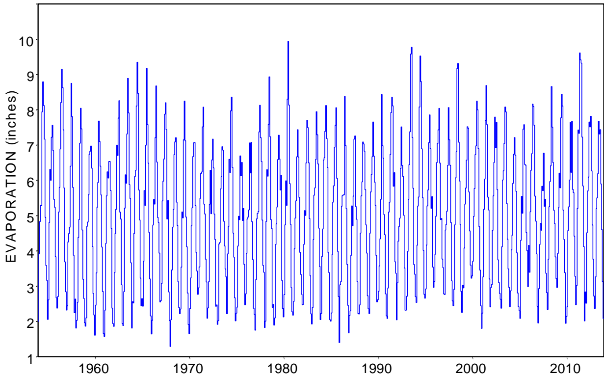
Figure 3.4 Monthly Reservoir Evaporation During 1954-2013 for the 92 Quadrangles
