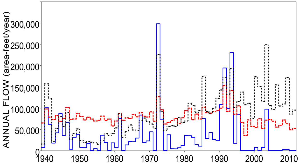
Naturalized (blue solid), Regulated (red dashed), and Observed (black dotted) 2-Month Minimum Annual Flows for Trinity River near Rosser
