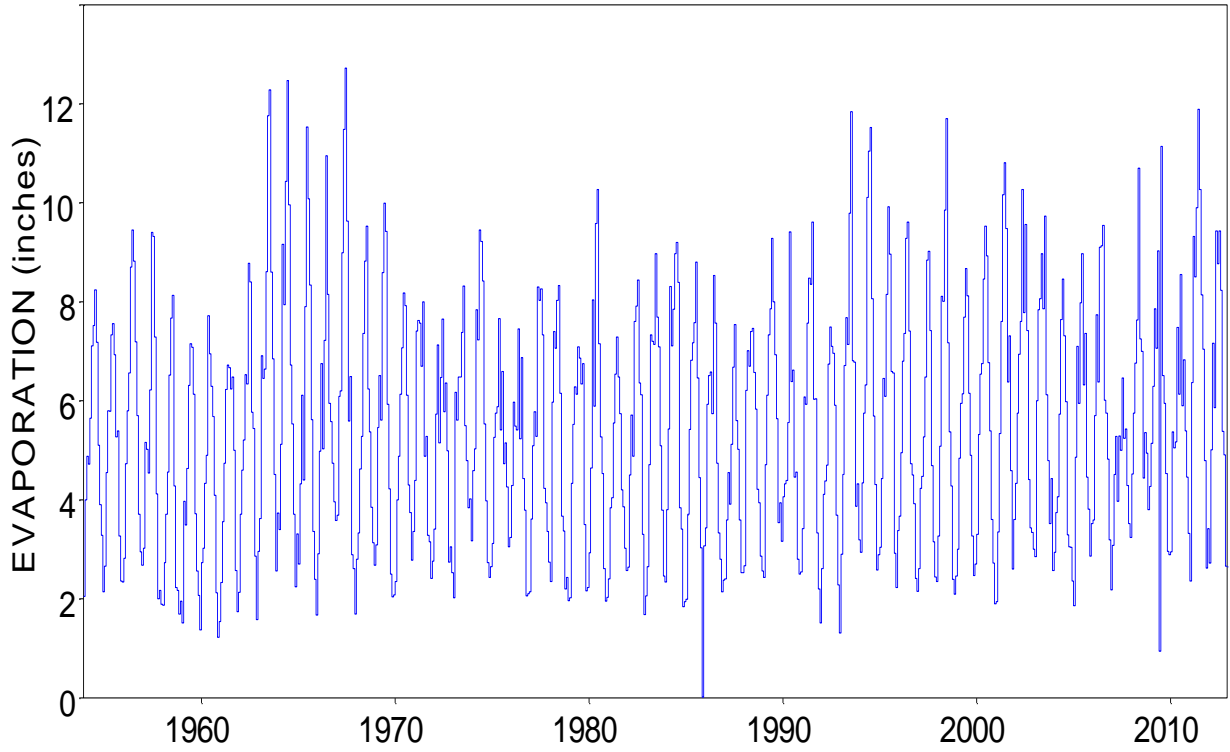
Monthly Evaporation for Quadrangle 805
