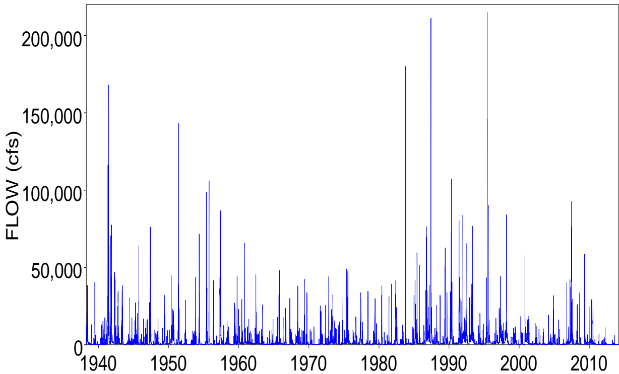
Daily Flows of Red River near Terrel
