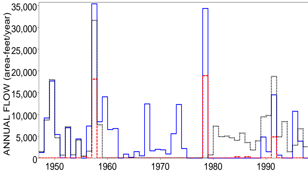
Naturalized (blue solid), Regulated (red dashed), and Observed (black dotted) 2-Month Minimum Annual Flows for Big Cypress Bayou at Jefferson
