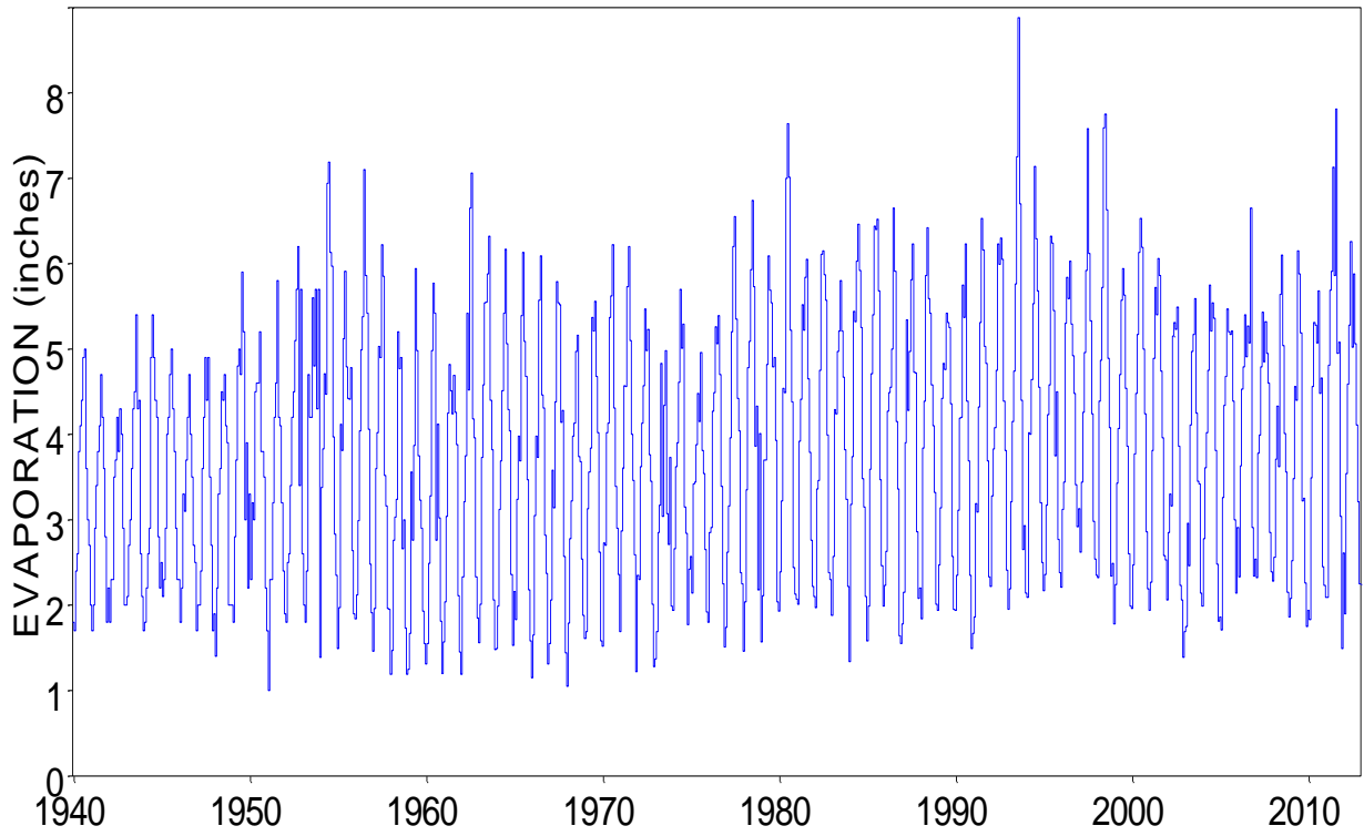
Monthly Evaporation for Quadrangle 714
