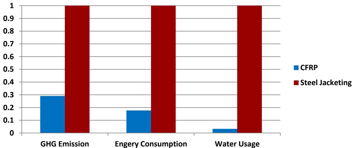
Figure 9. Characterization for the two retrofit techniques in this study
