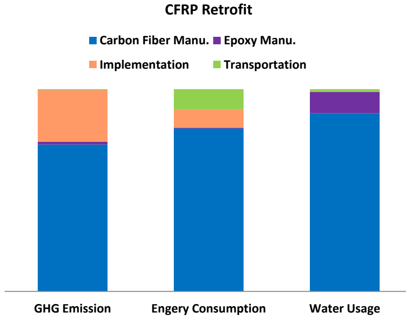
Figure 11. Contributions of each phase to the total impact - CFRP retrofit
