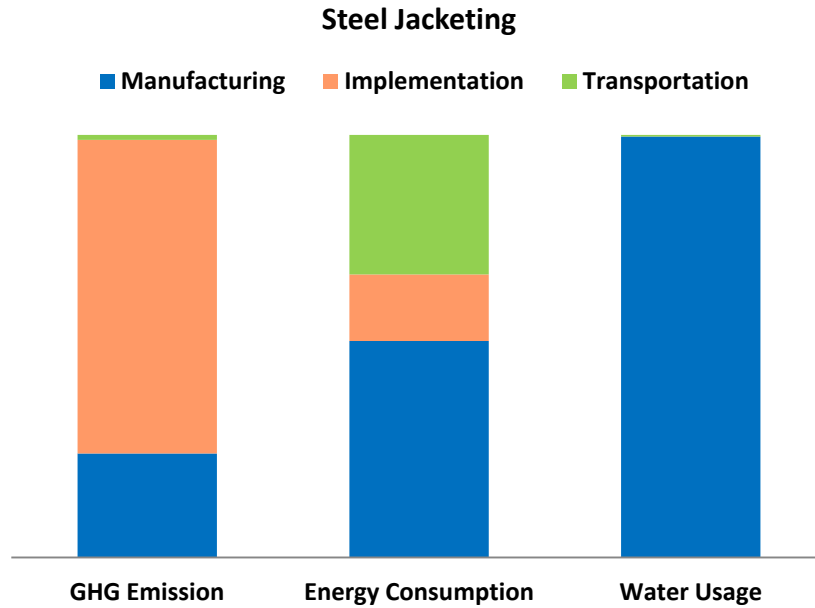
Figure 10. Contributions of each phase to the total impact - steel jacketing
