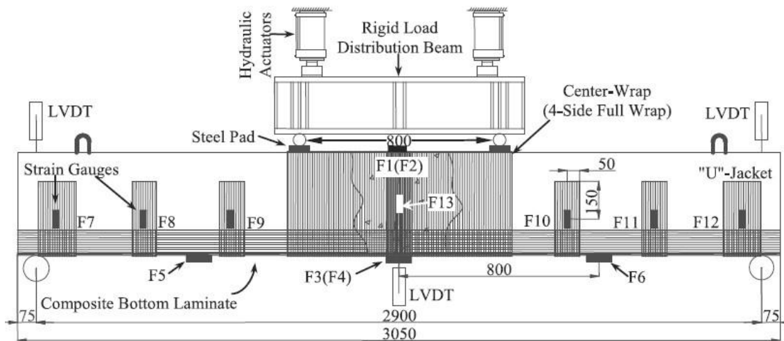
Figure 8. Retrofit schemes for CFRP retrofitting [5]
