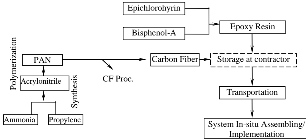
Figure 7. Elementary Flow of CFRP production (Cradle to Gate)
