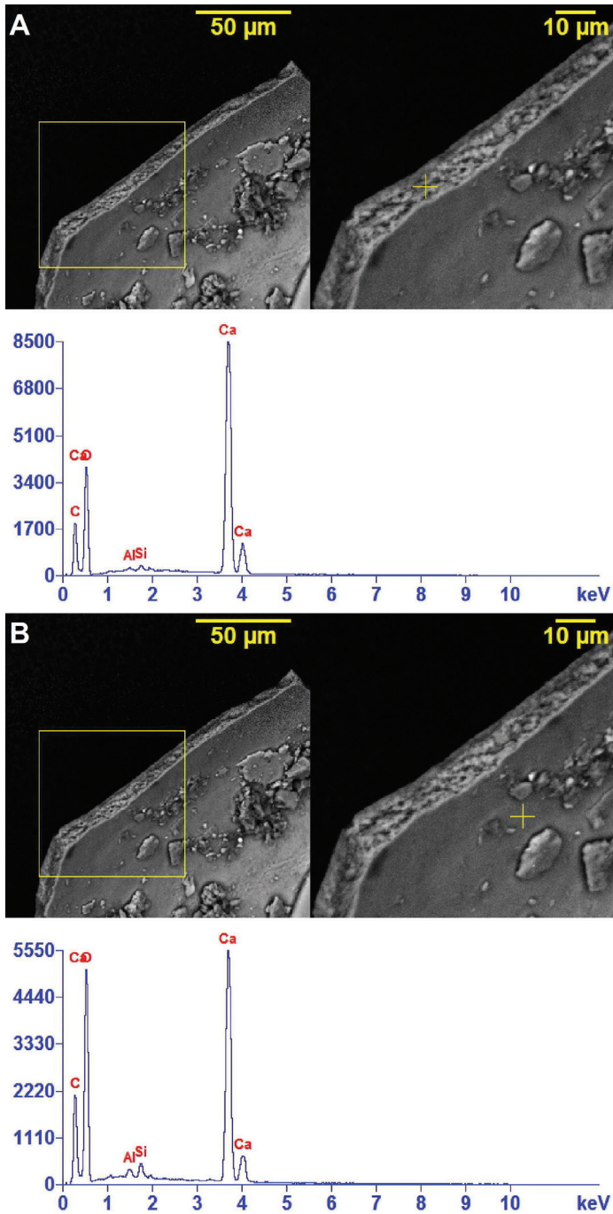
Figure 10. SEM-EDX spectroscopic images showing the spectrum of the elemental content in two regions of the inner shell of K. nodongense sp. n. paratype (NMBE 534361/2). A surface of shell edge B the inner layer of the shell. Both regions (yellow +) show the presence of calcium (Ca), aluminum (Al), silicon (Si) and carbon (C).
