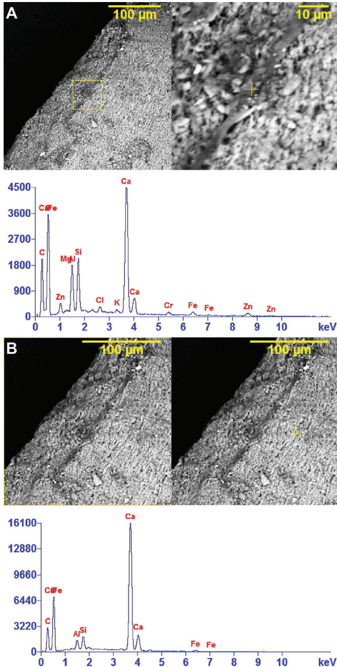
Figure 11. SEM-EDX spectroscopic images showing the elemental spectrum of two regions (yellow +) on the outside surface of the shell of K. nodongense sp. n. paratype (NMBE 534361/2). A band of compacted residue (sediment?) on the surface of the shell containing calcium (Ca), aluminum (Al), silicon (Si), oxygen (O), carbon (C), Iron (Fe), zinc (Zn), chromium (Cr) and potassium (K) B region to the left of A showing presence of calcium (Ca), aluminum (Al), silicon (Si), oxygen (O), carbon (C) and iron (Fe).
