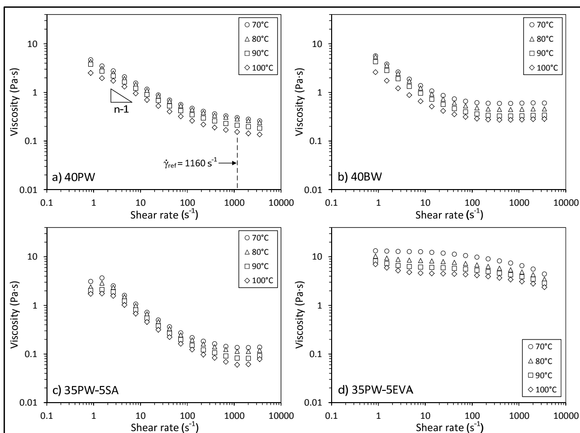
Figure 4.2 Viscosity profiles of feedstocks at different temperatures
