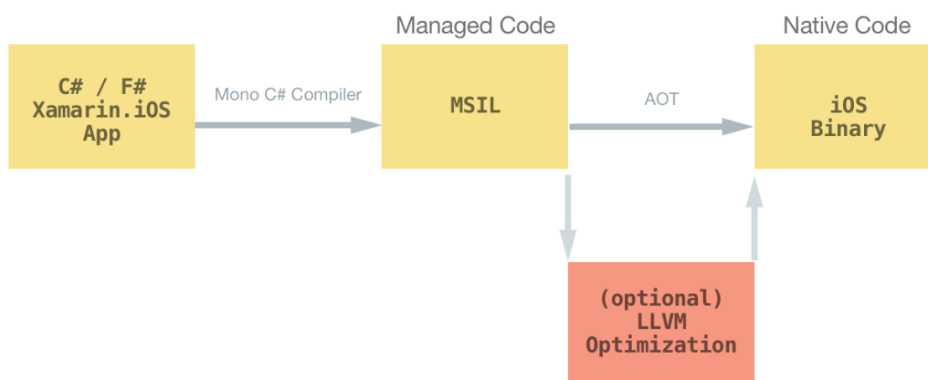
Figure 9 : Compilation Xamarin.iOS
