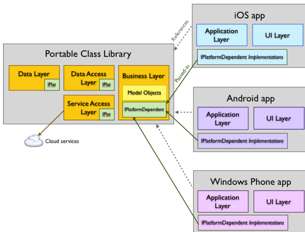
Figure 7 : Portable Class Library
