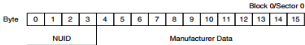
Figure 16 : Manufacturer Block
