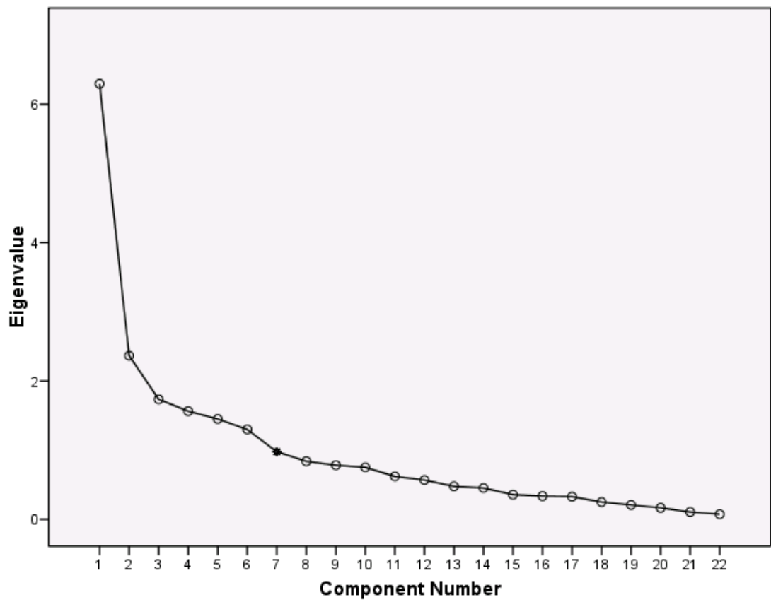
Figure 1: Scree plot – factor analysis of 22 items
