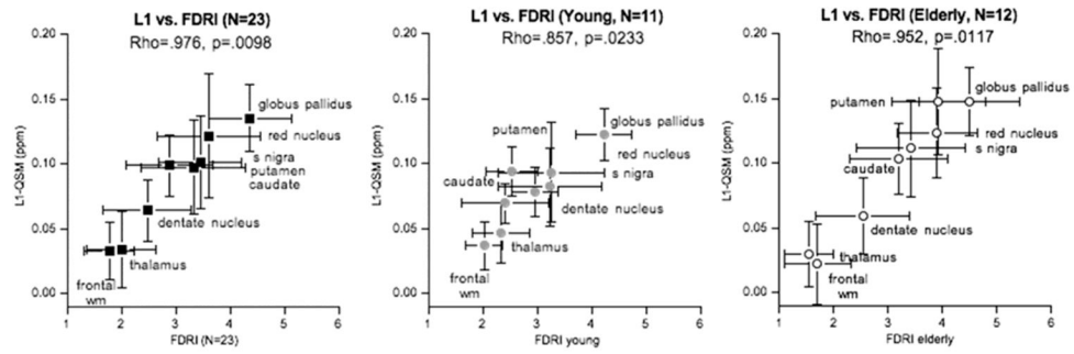
Fig. 5. Correlation between FDR I and \ell_1 -regularized QSM results on the regions of interest. Results indicate strong relationship between the two methods ( Rho = 0.976 , p = 0.0098 ). Left: all 23 subjects; middle: young group; right: elderly group.
