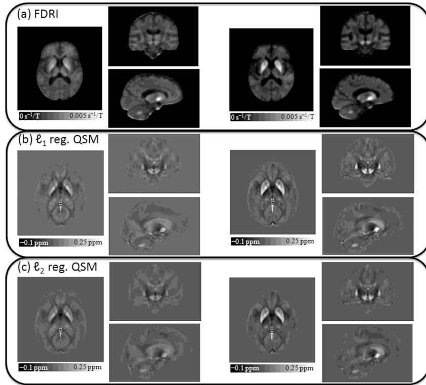
Fig. 3. Young (left) and elderly (right) group averages for FDR (a), \ell_1 -regularized QSM (b), and \ell_2 -regularized QSM (c). Greater iron concentration yields brighter QSM and FDR images. Splenium reference ROIs are indicated with a white box on the axial QSM slices.
