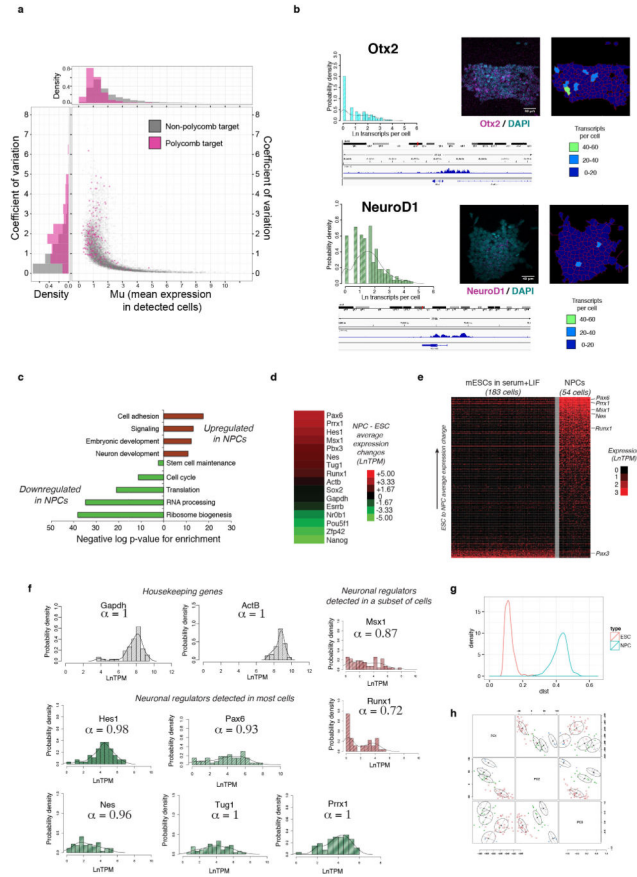
Extended Data Figure 4. Expression of Polycomb target genes in ESCs and NPCs (A) Polycomb target genes show highly variable expression in mESCs. Relationship between \mu (mean expression in detected cells, x-axis) and coefficient of variation (standard deviation normalized by mean expression in all cells, y-axis) is shown for Polycomb target genes (purple) and non-Polycomb target genes (grey). Distributions for \mu and coefficients of variation for the two gene sets are shown above and to the left of the graph, respectively. Polycomb target genes show pronounced variability in expression, even when controlling for expression level. (B) Expression of the neural regulators and Polycomb target genes Otx2 ( top ) and NeuroD1 ( bottom ) measured by RNA FISH in mESCs cultured in serum +LIF. ( left ). Overall distributions within the population and representative colonies are shown, along with gene tracks from IGV showing ChIP-Seq reads for H3K27me3 at the Otx2 and NeuroD1 genes. (C) Enriched gene ontology categories among genes significantly upregulated ( red ) or downregulated ( green ) in neural precursor cells as compared to embryonic stem cells. (D) Expression changes of selected genes in neural precursor cells as compared to the embryonic stem cells they were derived from. As expected, neural regulators and ES Polycomb target genes Pax6 , Prrx1 , Hes1 , Msx1 , Pbx3 , Nes , and Runx1
