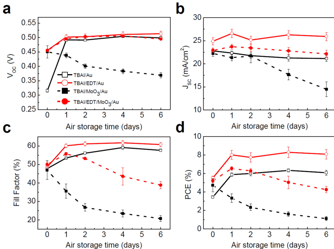
Figure 3. Evolution of photovoltaic parameters with air storage time in devices with Au and MoO 3 /Au anodes
