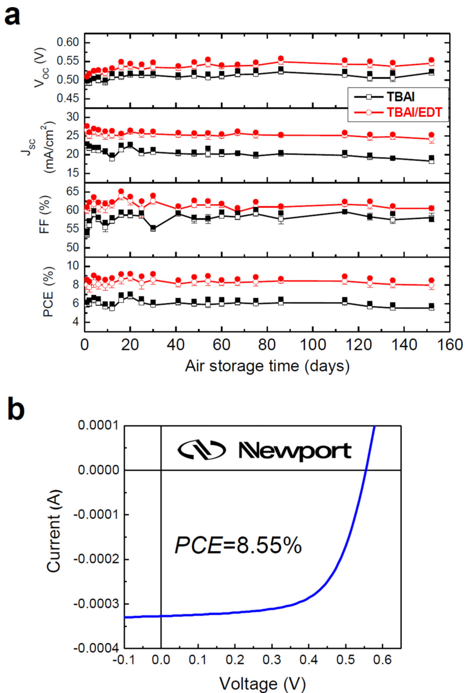
Figure 4. Long-term stability assessment of unencapsulated devices with Au anodes a , Evolution of photovoltaic parameters of PbS-TBAI (black) and PbS-TBAI/PbS-EDT (red) devices. Open symbols represent the average values and solid symbols represent the values for the best-performing device. b , Device performance of a PbS-TBAI/PbS-EDT device certified by an accredited laboratory after 37 days of air-storage.
