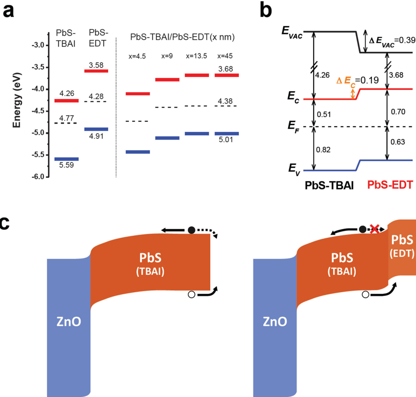
Figure 2. Energy level diagrams of PbS QDs and photovoltaic devices containing the QDs a , Energy levels with respect to vacuum for PbS-TBAI, PbS-EDT, and PbS-TBAI films covered with different thicknesses of PbS-EDT layers. The Fermi levels ( E_F , dashed line) and valence band edges ( E_V , blue lines) were determined by UPS. The conduction band edges ( E_C , red lines) were calculated by adding the optical bandgap energy of 1.33 eV, as determined from the first exciton absorption peak in the QD thin films, to E_V . b , Schematic energy level alignment at PbS-TBAI and PbS-EDT interfaces deduced from UPS. E_{VAC} : vacuum level. c , Schematic illustration of band bending in ZnO/PbS-TBAI and ZnO/PbS-TBAI/PbS-EDT devices at short-circuit conditions.
