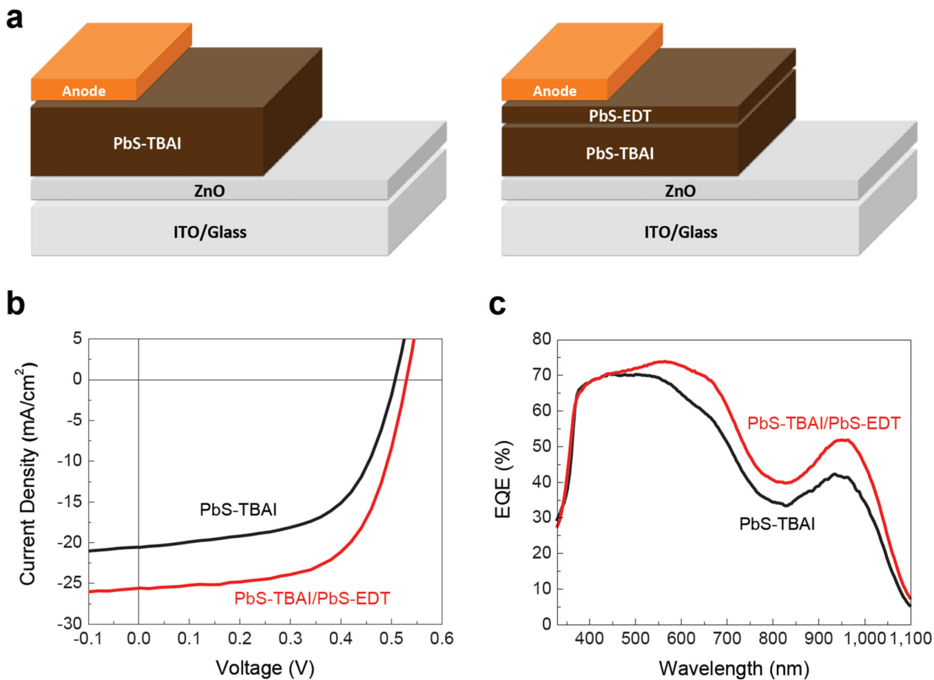
Figure 1. Photovoltaic device architectures and performance
