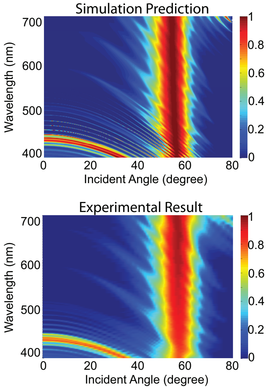
Fig. 4: Simulation and experimental measurement. Comparison between the p -polarized transmission spectrum of the Rigorous Coupled Wave Analysis (RCWA) simulation (27) and the corresponding experimental measurements.
