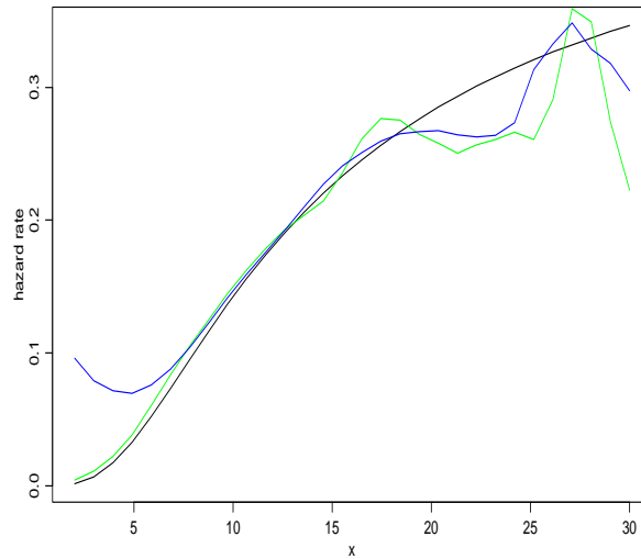
Figure 4.2: Estimation of the hazard rate of \chi_{12}^2 distribution (black line) by \hat{\lambda}_{T,2} (green) and \hat{\lambda}_{n,2} (blue).
