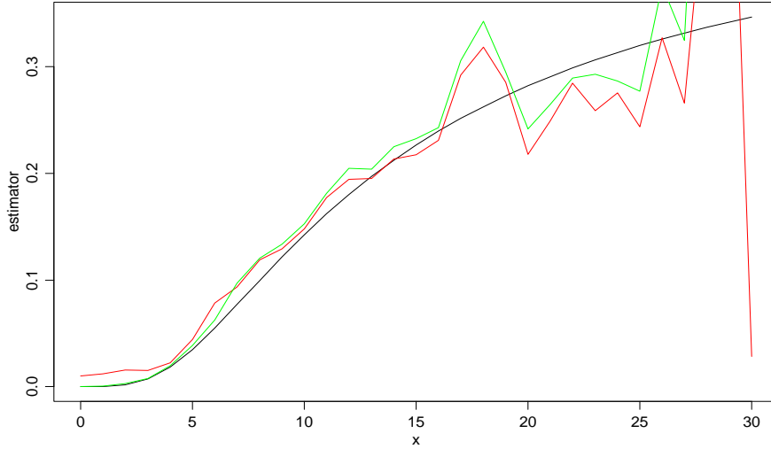
Figure 2.1: Comparison of \hat{\lambda}_L (green line) with estimator \hat{\lambda}_2 (red line). The black line is the true hazard rate of the \chi_{12}^2 distribution.
