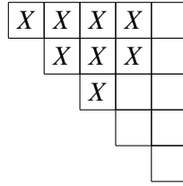
Figure 1. \lambda = (4, 3, 1) \subset \Lambda, n = 5 .
