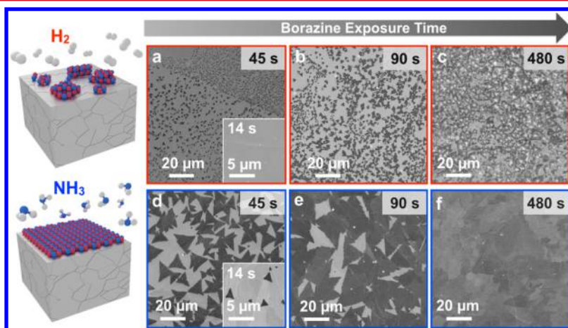
Figure 2. SEM images of h-BN domains grown at \sim 900\ ^\circ\text{C} and 6 \times 10^{-4} mbar borazine exposure on (a,b,c) \text{H}_2 -preannealed Fe foil for 45 s, 90 s, and 480 s borazine exposure time, respectively, and on (d,e,f) \text{NH}_3 -preannealed Fe foil for 45 s, 90 s, and 480 s borazine exposure time, respectively. The preannealing pressure in both \text{H}_2 and \text{NH}_3 is 4 mbar for all of the above growths. The insets in (a,d) correspond to 14 s exposures and illustrate the longer incubation time preceding nucleation of h-BN on the \text{H}_2 -preannealed sample.
