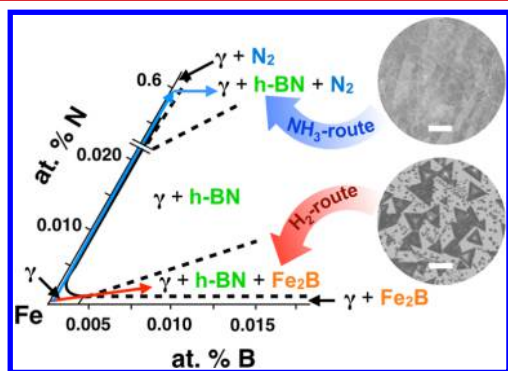
Figure 9. Fe-rich corner of the Fe–B–N phase diagram at 950 °C (adapted from Rogl and Schuster). 55 The red and blue arrows represent the reaction pathway for the H 2 - and NH 3 -preannealed foils respectively with the corresponding postgrowth SEM images of the sample surface. The scalebars are 20 μm.
