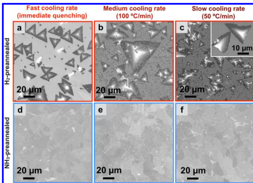
Figure 3. Morphology of h-BN on H 2 -preannealed Fe foil after (a) fast cooling (300 °C), (b) medium cooling (100 °C/min), and (c) slow cooling (50 °C/min). Inset: detail of multilayered domains with irregular edges, indicating possible dissolution of material back into the bulk during slow cooling. Morphology of h-BN on NH 3 -preannealed Fe foil after (d) fast cooling, (e) medium cooling, and (f) slow cooling. All growths were performed at ~900 °C and 6 \times 10^{-4} mbar borazine exposure for 5 min.
