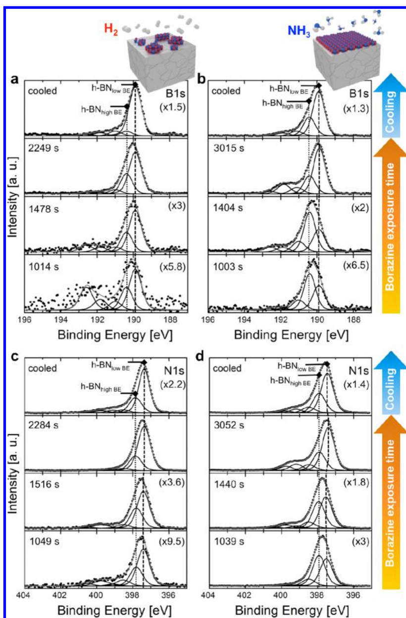
Figure 6. Time-resolved in situ XPS of the B1s core level for (a) H 2 - and (b) NH 3 -preannealed Fe foil and the N1s core level for (c) H 2 - and (d) NH 3 -preannealed Fe foil during borazine exposure and initial cooling stage ( \sim 900 °C, \sim 1 \times 10^{-4} mbar for NH 3 -preannealed sample and \sim 1 \times 10^{-3} mbar for H 2 -preannealed sample, \sim 10 min). Spectra are collected in normal emission geometry at photon energies of 620 eV ( \lambda_{\text{escape}} \approx 13 Å).
