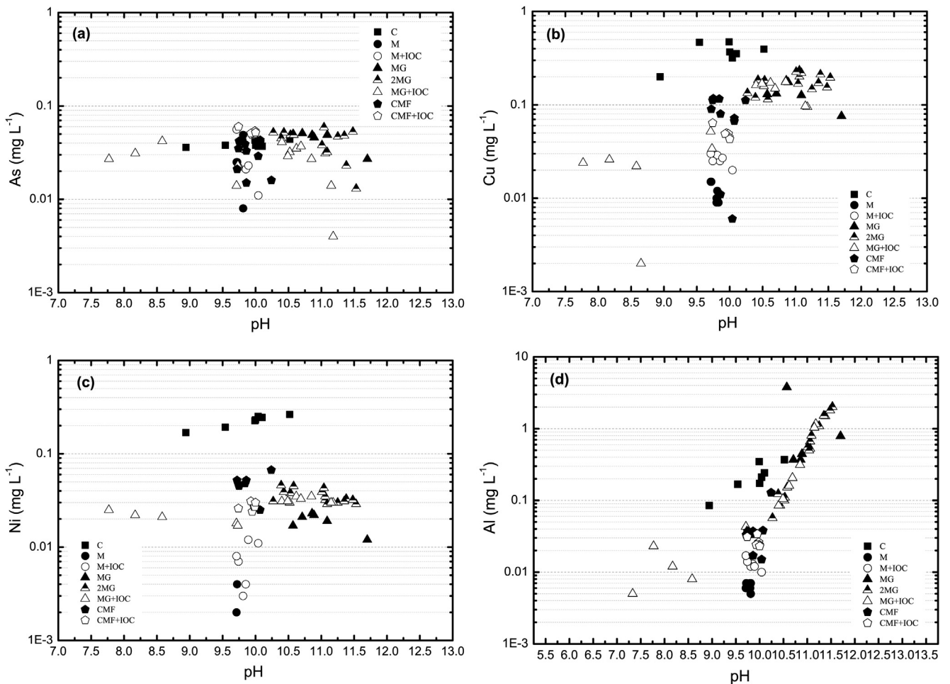
Fig. 5. Concentrations of (a) As, (b) Cu, (c) Ni, and (d) Al in the leachates as a function of pH.
