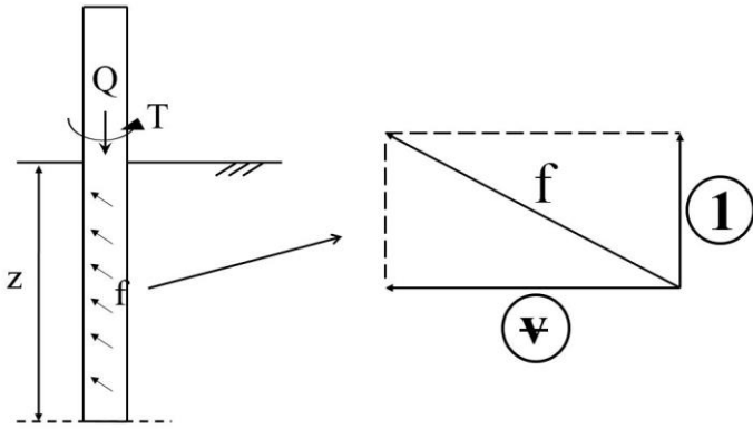
Fig. 4 Decomposition of pile-soil friction \delta f .
