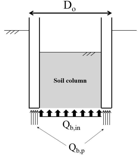
Fig. 11 Decomposition of Q_b in an open ended pile.
