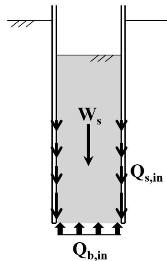
Fig. 9 Forces acting on the soil column.
