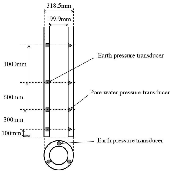
Fig. 12 Schematic illustration of the test pile.
