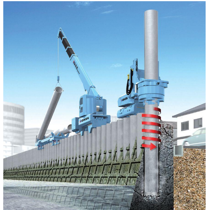
Fig. 1 ‘Gyropiler’ for rotary press-in, with GRB System.
