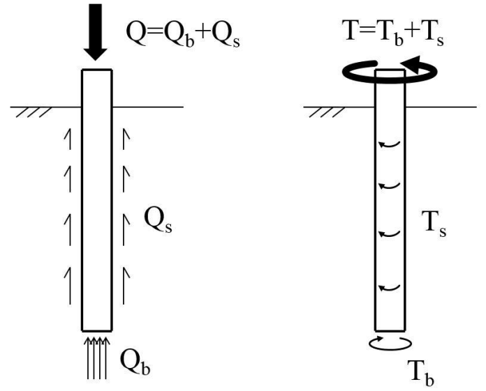
Fig. 3 Decomposition of Q and T.
