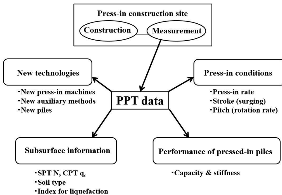
Fig. 2 Concept of ‘PPT’ - Pile Penetration Test.
