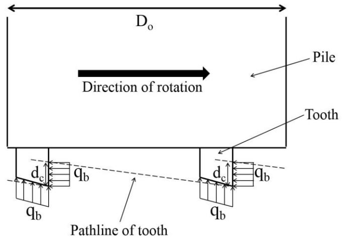
Fig. 14 Assumption of the resistance on the teeth.
