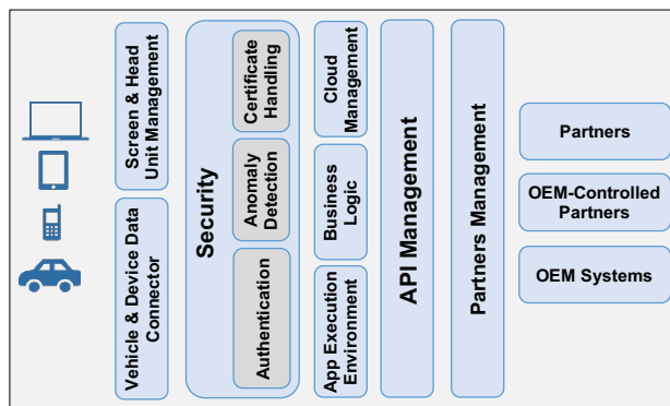
Figure 5 Ericsson Connected Vehicle Cloud Overview [16]
