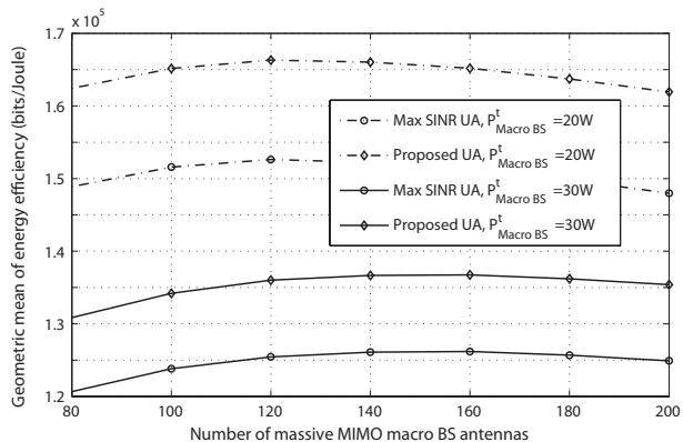
Fig. 7. Energy efficiency versus the number of antennas for different downlink transmit powers of the macro BS P_{\text{Macro BS}}^t .
