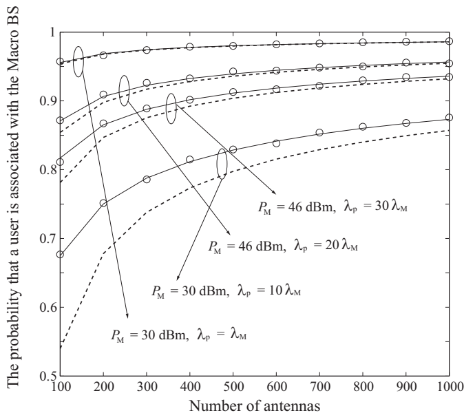
Fig. 6. The probability that a user is associated with the macro BS. The locations of the macro BSs and the pico BSs follow independent homogeneous Poisson point processes with densities \lambda_M and \lambda_p , respectively. The carrier frequency is 1 GHz, S = 5 , P_M is the macro BS transmit power, and P_p = 30 dBm is the pico BS transmit power. The solid lines are validated by Monte Carlo simulations marked with ‘o’ and the dashed lines represent the asymptotic results as the number of antennas goes towards infinity.
