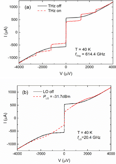
Fig. 2. DC IVCs under (a) the illumination of a 614.4 GHz signal and (b) LO pumping (at fundamental frequency) at T = 40 \text{ K} .
