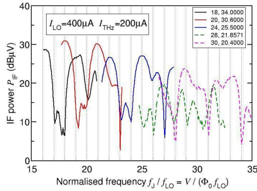
Fig. 8 Simulated P_{IF} as a function of the average voltage V , where V has been expressed in terms of the Josephson frequency f_j = V/\Phi_0 , and then normalized to the LO frequency f_{LO} . The legend box lists values of N , and the corresponding values of f_{LO} in GHz, for each of the sub-plots.
