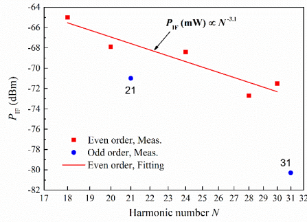
Fig. 5. Experimental result of IF output power versus the harmonic number.
