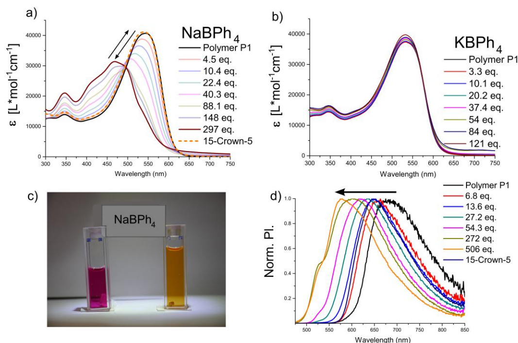
Figure 5: (Figure changed, \text{NaBPh}_4 was missing) Titration experiments of P1 and \text{MBPh}_4 ( \text{M} = \text{Na}, \text{K} ) in THF, a) addition of \text{NaBPh}_4 and 15-Crown-5 b) addition of \text{KBPh}_4 , c) color change after addition of 300 eq. \text{NaBPh}_4 . d) PL shift with \text{NaBPh}_4 .
