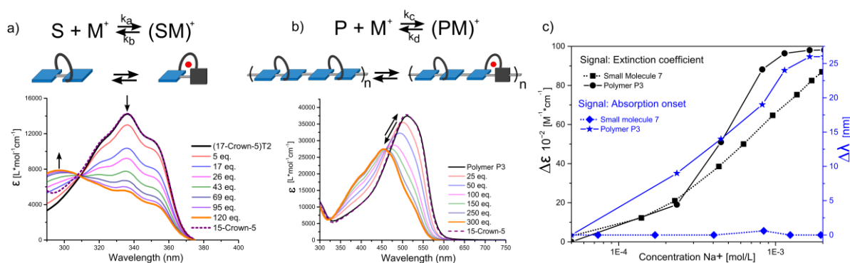
Figure 7: Comparison of a visible sensor based on a) small molecule and response of (17-Crown-5)T2 towards \text{NaBPh}_4 in THF b) polymeric structure, and response of polymer P3 towards \text{NaBPh}_4 in THF c) Sensitivity measurements of small molecule (17-Crown-5)T2 and polymer P3. The X-axis shows the concentration of \text{NaBPh}_4 in THF. a) Y-axis left: Difference in extinction coefficient ( \Delta\epsilon = \epsilon_0 - \epsilon ). Right Y-axis Difference in absorption onset \Delta\lambda = \lambda_0 - \lambda .
