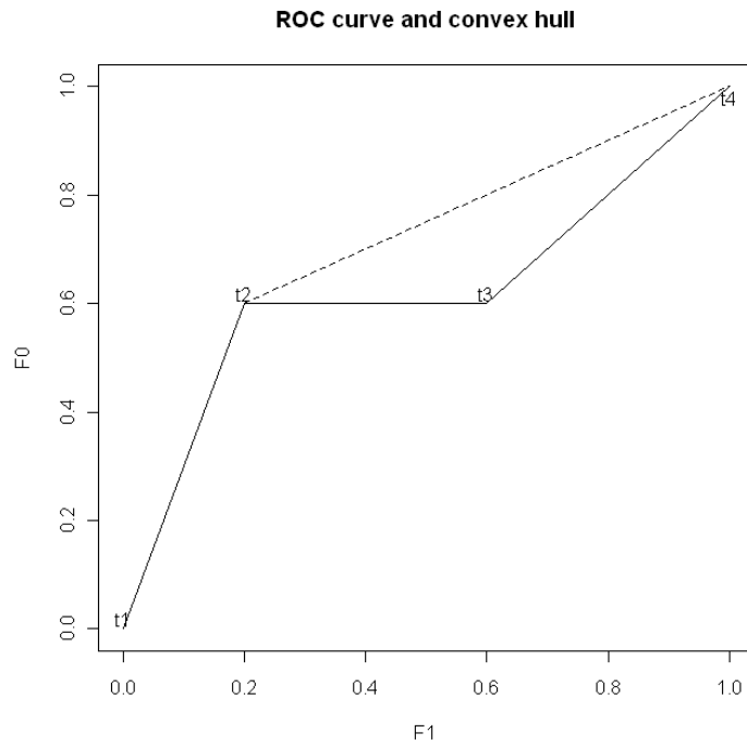
Figure 1: The ROC curve and the convex hull
