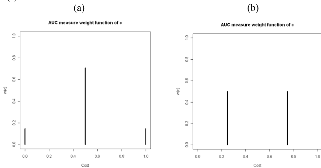
Figure 4: The w(c) functions corresponding to the ROC curves in Figures 3(b) and 3(c).
