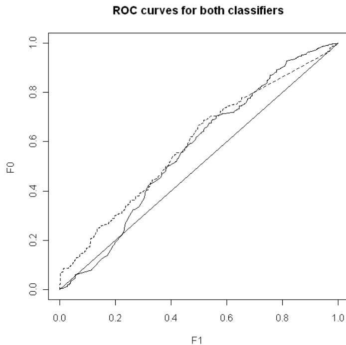
Figure 7: ROC curves for the two classifiers using the data from Thomas et al (2002).
