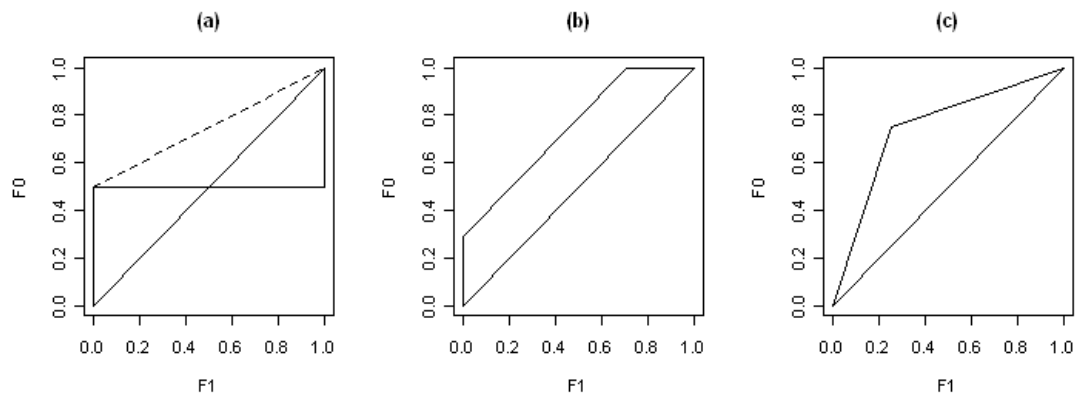
Figure 3: Examples of three ROC curves.
