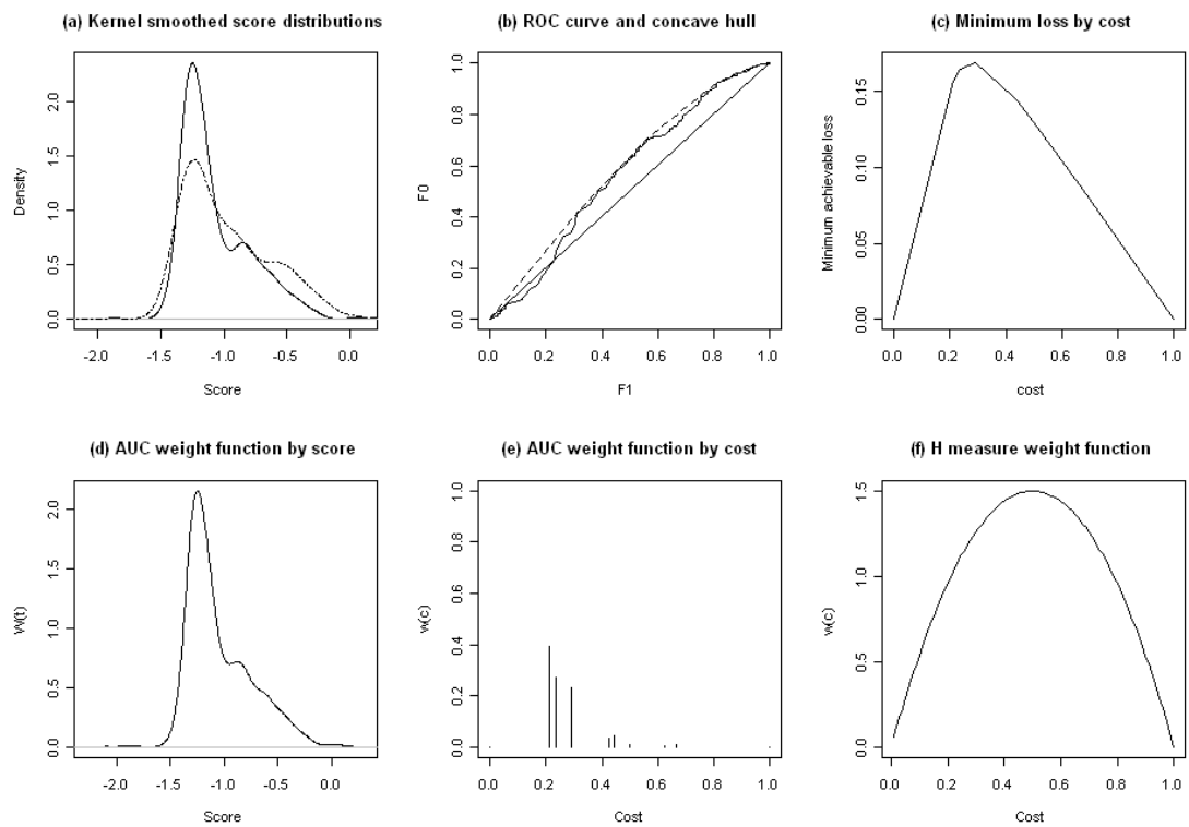
Figure 5: Plots for first classifier on data from Thomas et al (2002).
