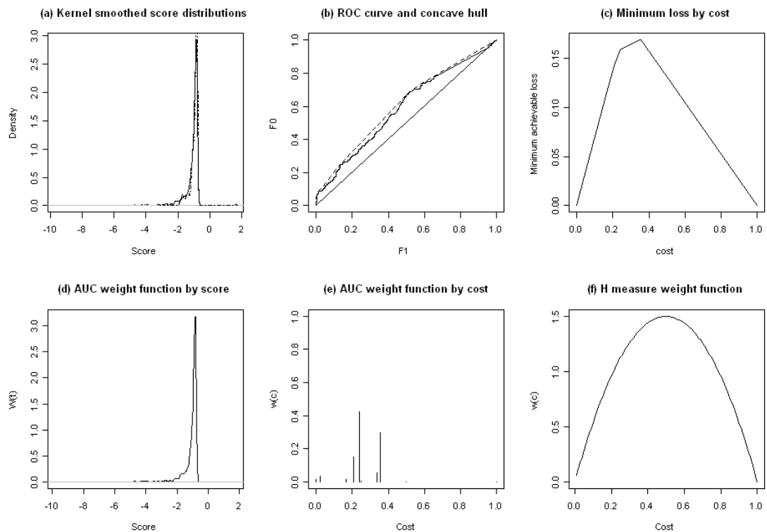
Figure 6: Plots for second classifier on data from Thomas et al (2002).
