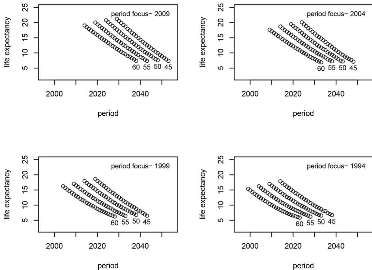
Fig 1. Simulated median deferred period life expectancy projections, focus ages 60(-)45, based on retirement age 65. UK male mortality 1961-2009(-)1994 experience (by panel), ages 1-89. MIRCO joint modelling with multiplicative bi-linear age-period parametric structure. ARI(1,0) time series.
