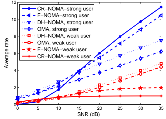
Fig. 2. The average rate for strong user and weak user in DH-NOMA systems compare to other multiple access schemes, where M = 4 , p = 1 , q = 4 , and \beta = 0.6 . For F-NOMA, \alpha_w = 0.25 ; For CR-NOMA, R_v = 1 bits/s/Hz.
