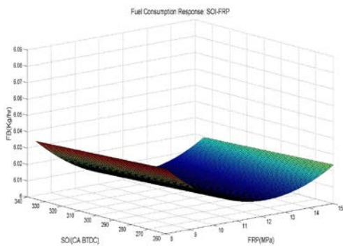
Fig.31 Fuel consumption response at MV1 Stage
