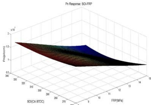
Fig. 30 PN response at MV4 Stage
