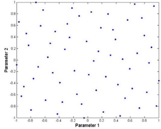
Fig. 6 MB Sequence (60 test points)
