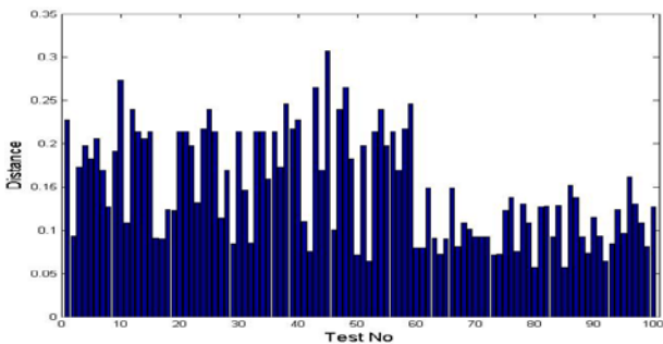
Fig. 13 Euclidean minimum distance for MB-MV test points
