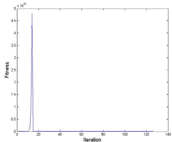
Fig. 20 Convergence plot for PermGA
