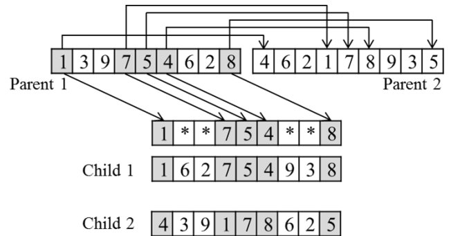
Fig. 3 Cycle crossover
