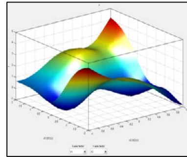
RBF Model (PRESS RMSE: 0.43)
