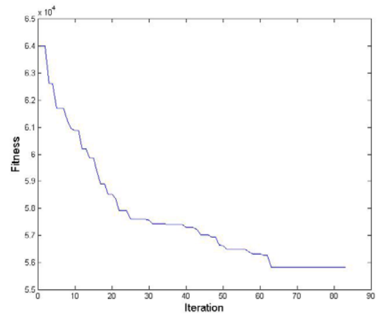
Fig. 11 Convergence plot for PermGA
