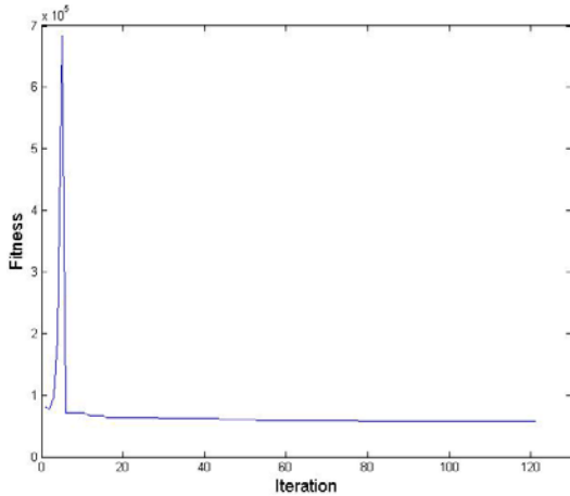
Fig. 17 Convergence plot for PermGA
