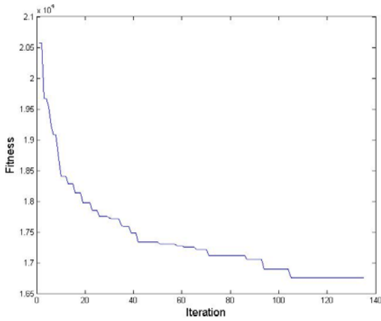
Fig. 8 Convergence plot of PermGA for generating the MB OLH DoE sequence (60 points in 2 dimensions)
