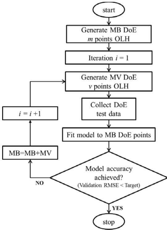
Fig. 1 MB-MV Strategy Flowchart
