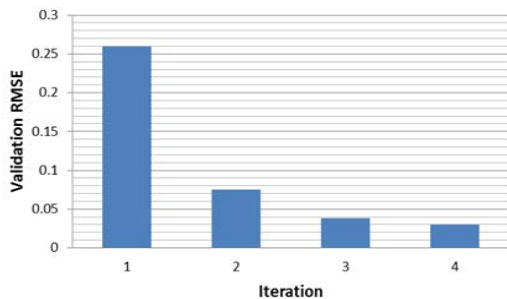
Fig. 25 External validation of the built models through MB-MV sequence (Stages 1 to 4)
