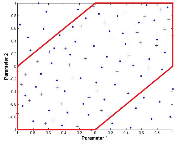
Fig. 18 MB-MV Sequence for asymmetric design space
