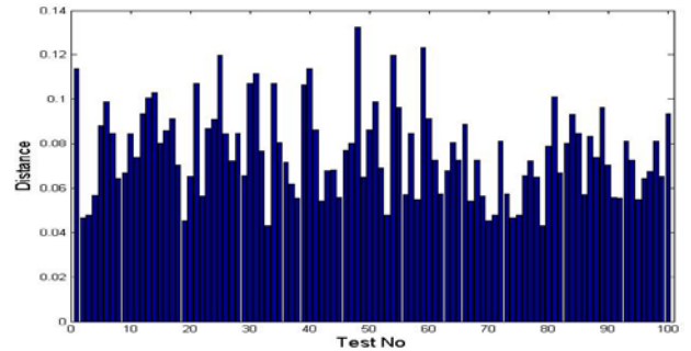
Fig. 19 Euclidean minimum distance for MB-MV test points
