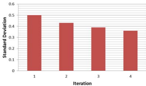
Fig. 24 Standard deviation ( \sigma ) of the Mm Distance (Stages 1 to 4)
