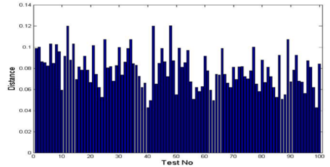
Fig. 10 Euclidean minimum distance for MB-MV test points
