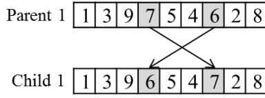
Fig. 5 Mutation operator
