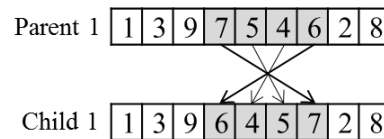
Fig. 4 Inversion crossover
