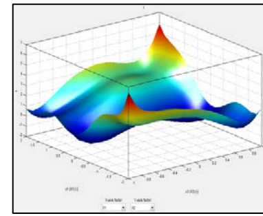
RBF Model (PRESS RMSE: 0.1)
