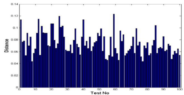
Fig. 16 Euclidean minimum distance for MB-MV test points
