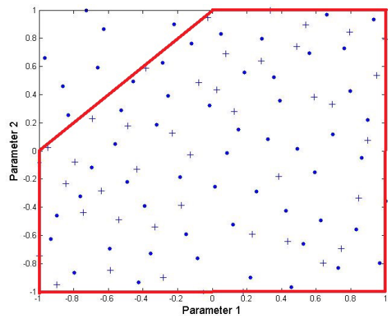
Fig. 15 MB-MV Sequence for asymmetric design space
