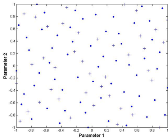
Fig. 9 MB-MV Sequence for symmetric design space
