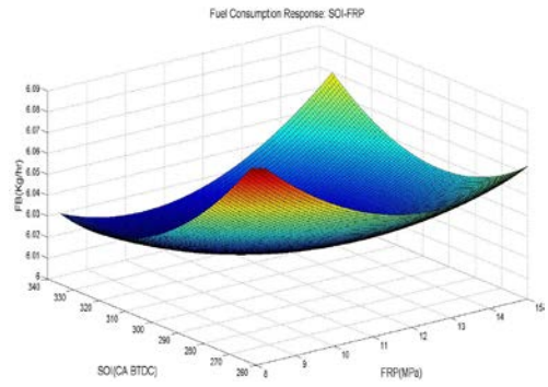
Fig. 32 Fuel consumption response at MV4 Stage
