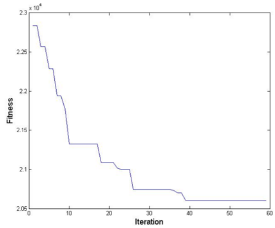
Fig. 14 Convergence plot for PermGA
