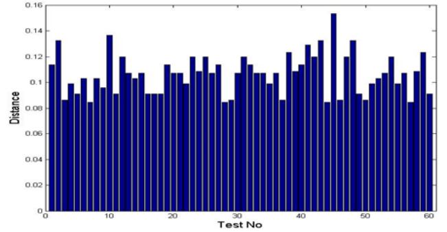
Fig. 7 Euclidean minimum distance for all MB DoE points
