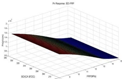
Fig. 29 PN response at MV1 Stage
