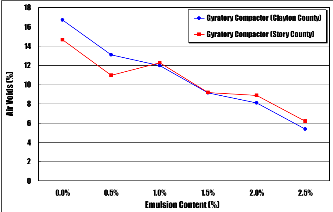
Figure 7-8. Plots of air void against emulsified asphalt content for gyrotory compacted CIR-HFMS-2p specimens using two different RAP materials
