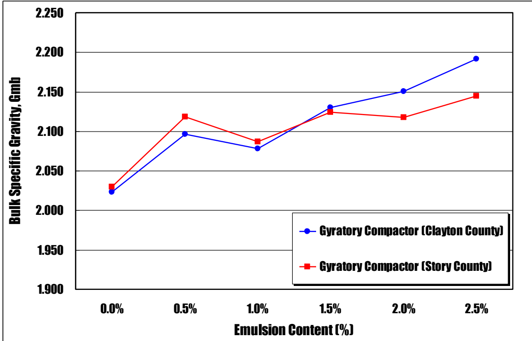
Figure 7-3. Plots of bulk specific gravity against emulsified asphalt content for gyrotory compacted CIR-HEMS-2p specimens using different RAP materials
