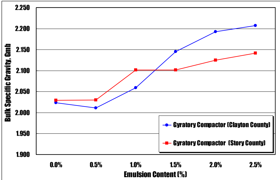
Figure 7-1. Plots of bulk specific gravity against emulsified asphalt content for gyrotory compacted CIR-CSS-1h specimens using different RAP materials
