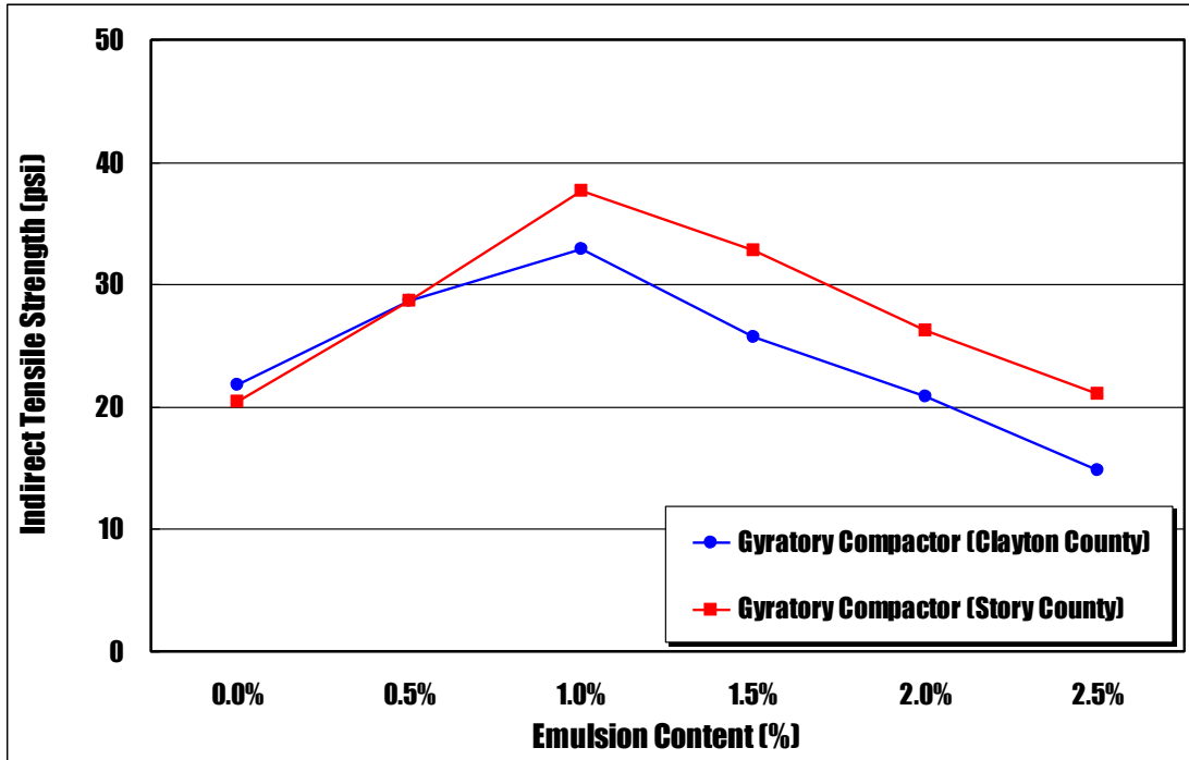
Figure 7-11. Plots of indirect tensile strength against emulsified asphalt content for Gyrotory compacted CIR-CSS-1 specimens using two different RAP materials
