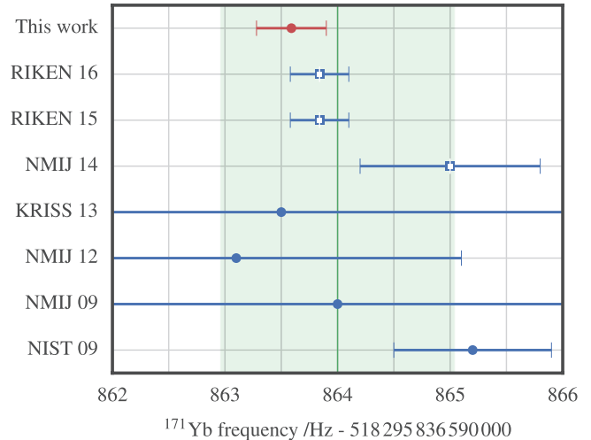
Figure 11. Absolute frequency measurement of the ^1\text{S}_0\text{--}^3\text{P}_0 transition of ^{171}\text{Yb} measured by different laboratories and years: NIST [8], NMIJ [25, 27, 28], KRIS [26], RIKEN [24, 29]. The shaded region gives the recommended frequency for ^{171}\text{Yb} as a secondary representation of the second of CIPM 2015, with its uncertainty. Open squares denote absolute frequencies deduced from ^{171}\text{Yb}/^{87}\text{Sr} ratio measurements and the recommended value of ^{87}\text{Sr} as a secondary representation of the second with its uncertainty. Circles denote measures relative to the realization of the second by caesium standards.
