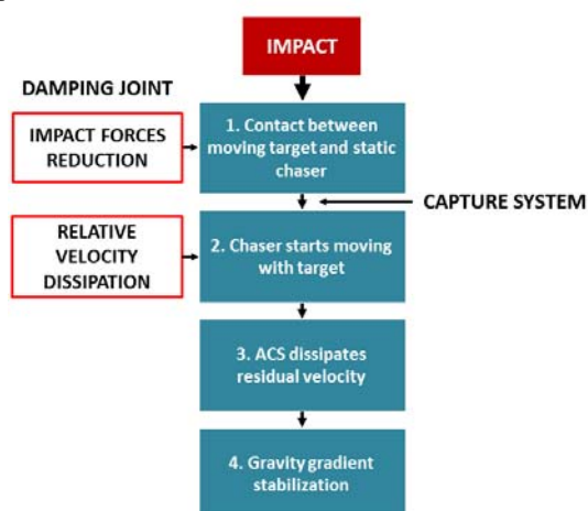
Fig. 8: Capture procedure main phases.
