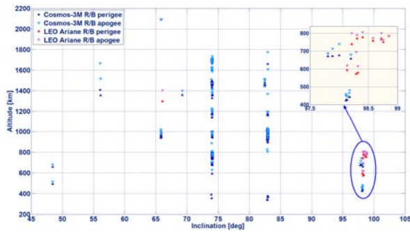
Fig. 3: Distribution of Ariane and Cosmos-3M rocket bodies (R/B) fully residing in LEO as a function of perigee/apogee altitude and inclination (19 July 2012).
