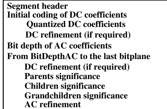
Fig. 7: CCSDS-IDC: Bit plane encoding processing order.
