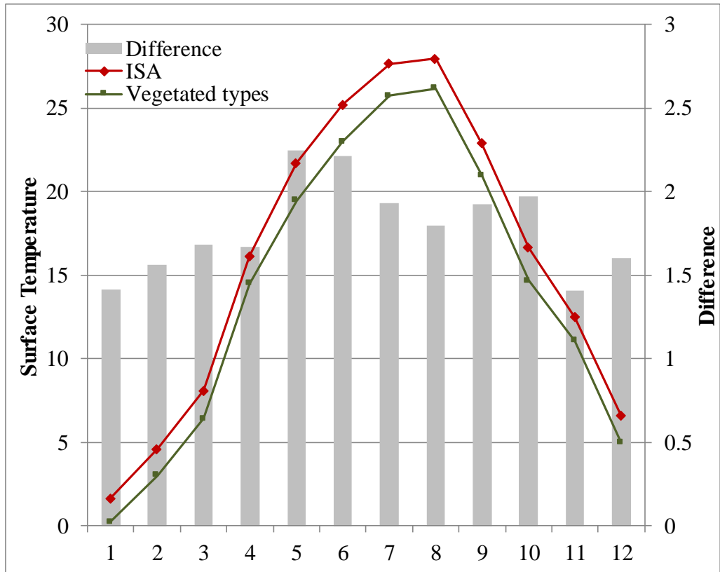
Figure 5: Annual average SiB2 modeled canopy temperature (left axis) for impervious surface area (red color) and the weighted vegetated land covers (green color) for all the ISA CMGs in USA. The average temperature difference is shown in grey bars (right axis).
