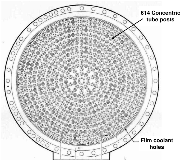
Figure 12-14: Coaxial injector face of the J-2 engine, consisting of 614 tube-within-a-tube elements. Material: austenitic stainless steel. (NASA archives)
