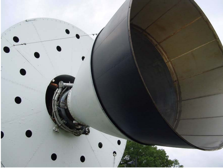
Figure 12-30. Apollo Service Propulsion Module Engine. Expansion nozzle is made from niobium alloy C103. Nozzle extension is welded titanium alloy sheet metal. (Photo taken at the Huntsville Space Museum)
