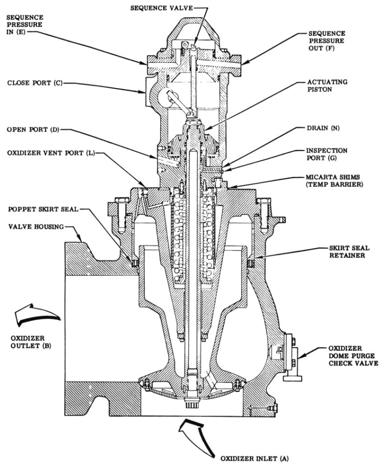
Oxidizer Valve
