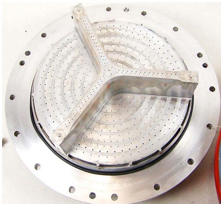
Figure 12-12. A baffled, concentric-ring injector for an Atlas launch vehicle. OFHC Copper rings brazed into a stainless steel body. (NASA archives)
