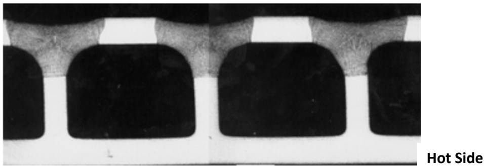
Figure 12-29. Volvo laser welded sandwich expansion nozzle. Tubes and cover sheet are stainless steel. [11][12] (Courtesy of Volvo Aero)
