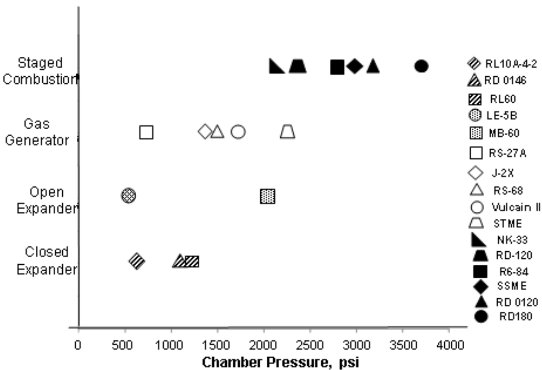
Figure 12-5. Chamber Pressure Range for Various Pump-Fed Cycles
