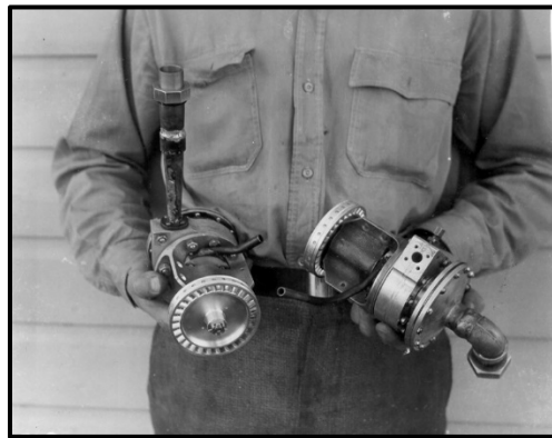
Figure 12-36 Fuel and oxidizer turbopumps for Dr. Robert Goddard’s rocket. (Clark University archives)
