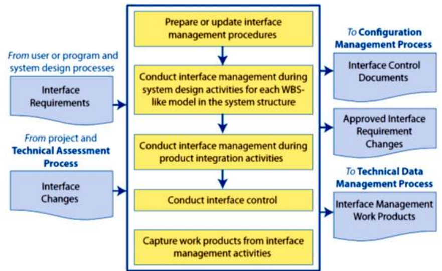
Figure 5. Interface Management Flow Diagram
