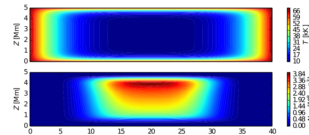
Figure 3 Vertical slice of the model FC defined by Eq. (1). Top panel: temperature; bottom panel: neutral hydrogen density. The thread is infinite in the Y direction. The geometry of the PCTR depend strongly on location in the FC and the parameters \gamma_x and \gamma_z , here \gamma_x = 2 and \gamma_z = 5 .
