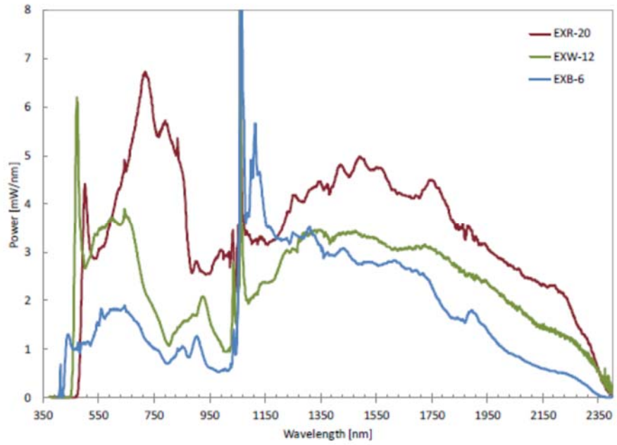
Figure 3. NKT Spectral Coverage, 6W, 12W and 20W sources
