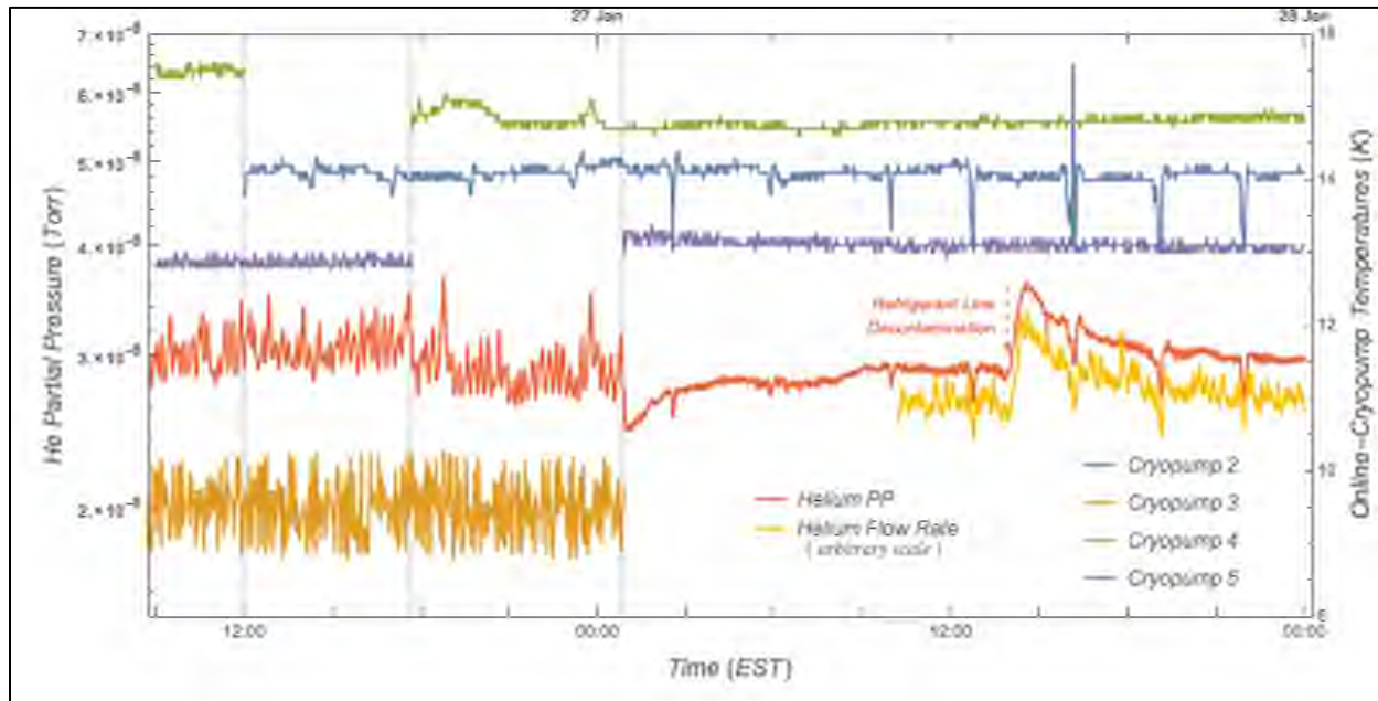
Figure 11. Plot of cryopump temperatures and Helium partial pressure during a period of various online cryopump combinations (trios) and initiation of cryocooler refrigerant line decontamination (exterior surface). Also shown is the flow rate profile from a Helium leak detector – plumbed in parallel with a mechanical pump and, together, backing the main chamber turbopump – during decontamination
