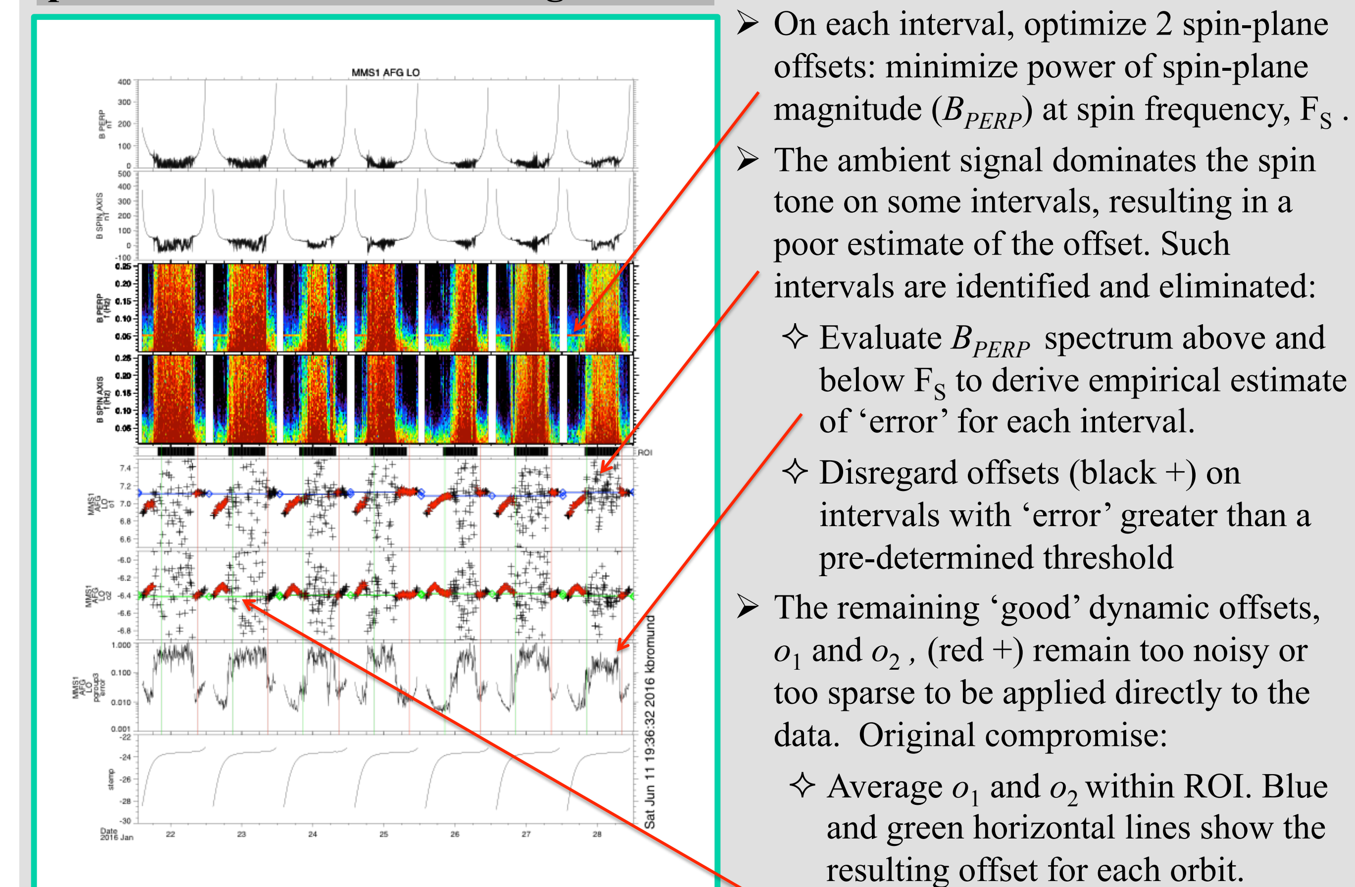
Fig. 1. Low-range calibration diagnostic, for typical week of Phase 1A: 21-28 January, 2016
