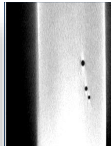
CT Scan of Stainless Steel
