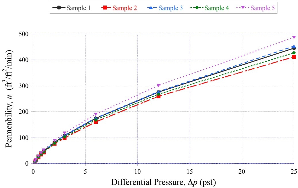
(a) Full differential pressure range: 0.146-25 psf (7-1197 Pa).
