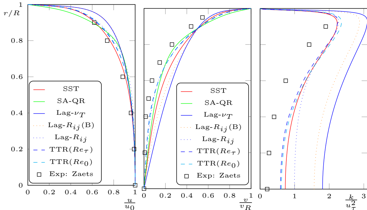
(a) Axial Velocity (b) Circumferential Velocity (c) Turbulent Kinetic Energy
