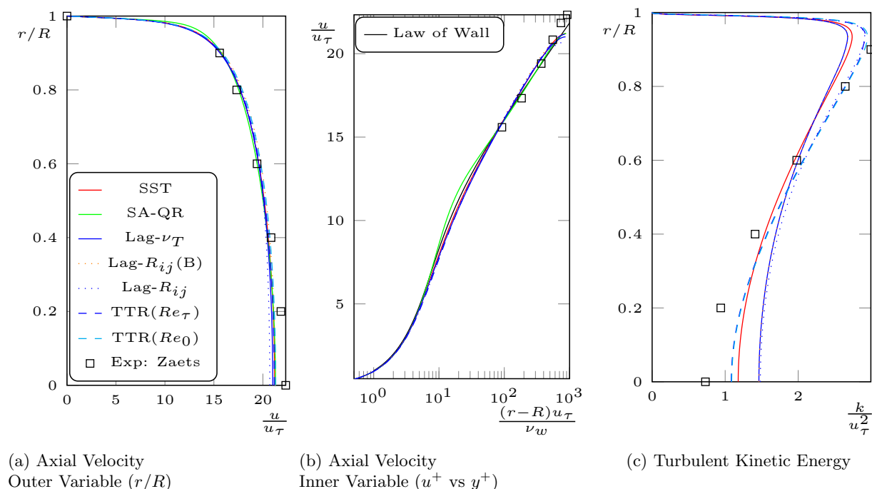
Figure 6: Inflow velocity and k profiles( x/R = -10 )
