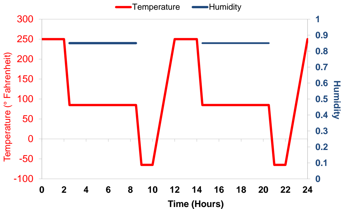
Figure 2. Daily Temperature and Humidity Aging Cycle
