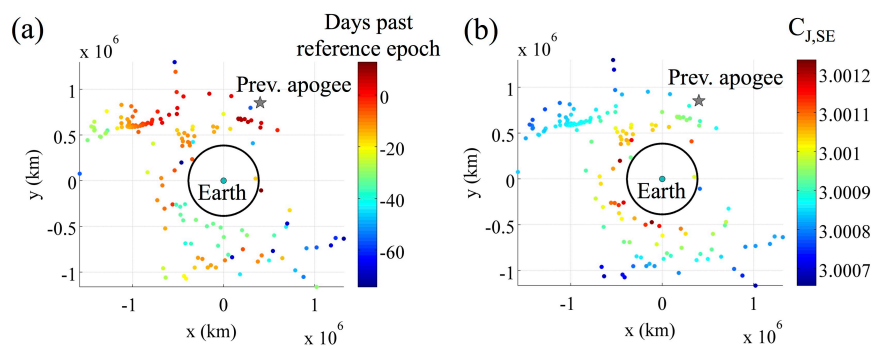
Figure 14: Apoapsis map representing trajectories that approach the lunar science orbit, projected into planar configuration space and colored by the epoch at each apogee.
