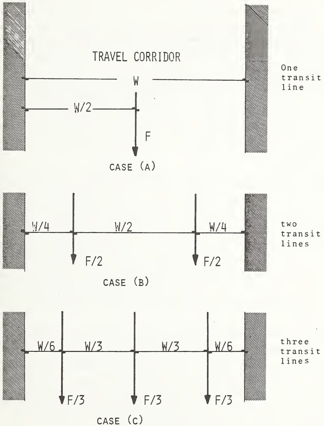
Figure 2.9. Relationship between line spacing and frequency of service for a given fleet size
