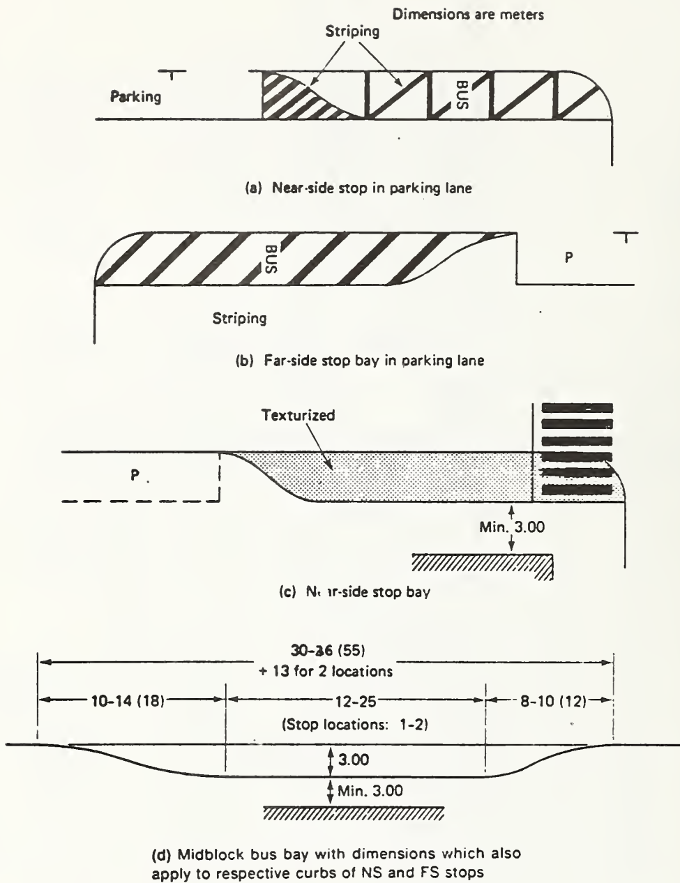
Figure 5.5 Design details and dimensions of bus bays
