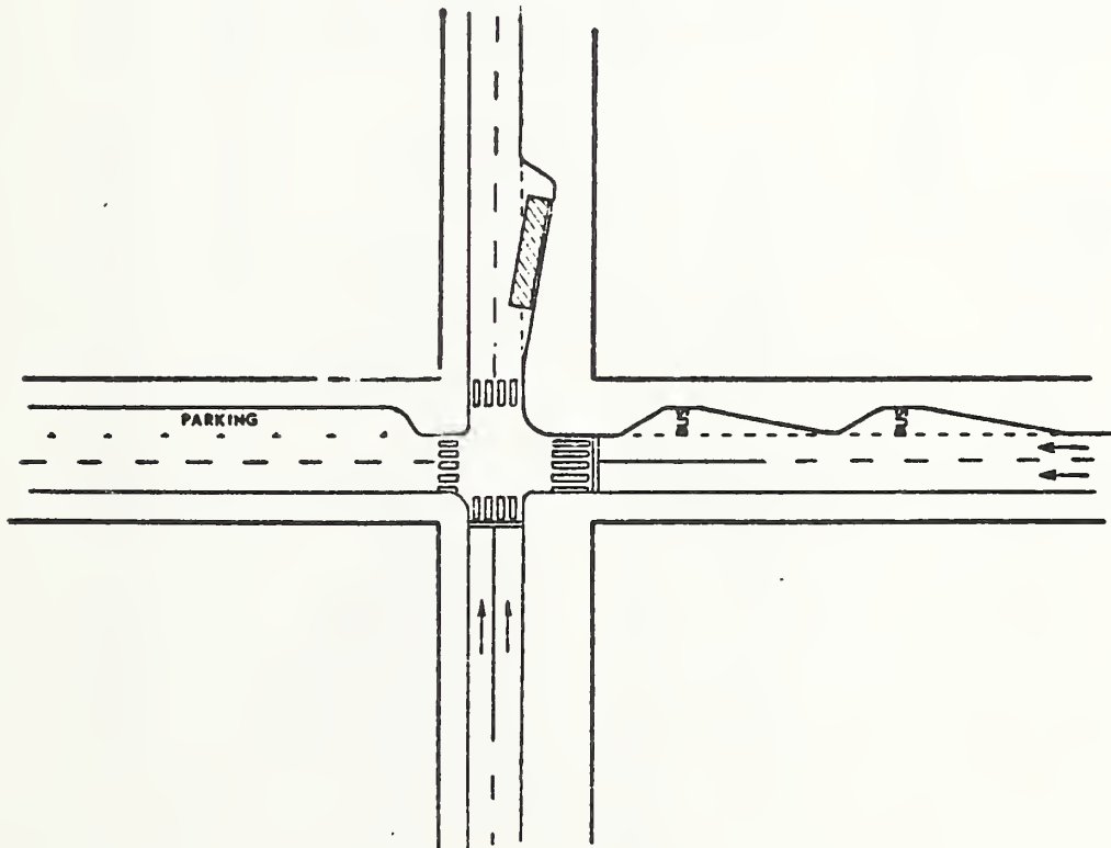
Figure 5.2 Sawtooth design of bus stops on street
