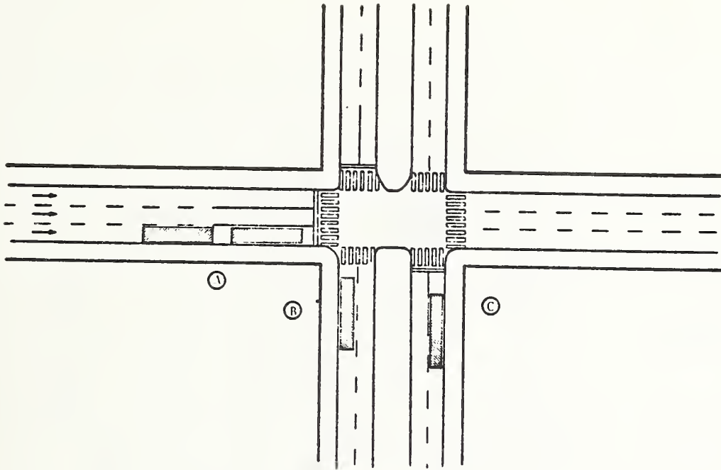
Figure 5.1 On-street transit center with curb stops
