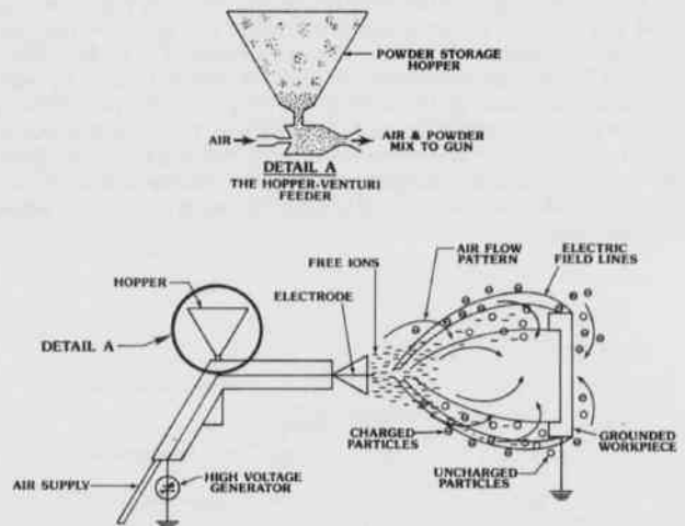
Figure 6. Electrostatic spray deposition method.
