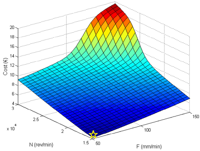
Figure 15. Cost per pass C_{tot}^{ith} [€] at Average Geometric Error, AGE=25%
