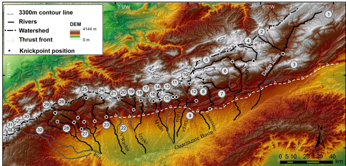
Figure 3. STRM DEM (USGS, 2006) of the area indicated in Figure 1, indicating the river long profiles extracted for this study. Each river is numbered corresponding to data in Table 1 and the long profile of selected rivers shown in figures 7, 8, 10.
