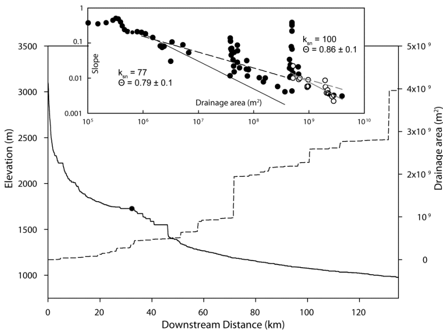
Figure 14. River long profile (elevation against downstream distance) of the Todra river (solid line) and drainage area downstream (dashed lines), the knickpoint is indicated with a solid circle. Inset shows the slope-area plot, steps in the long profile create noise in the data but a vertical step in the k_{sn} values can be determined across the knickpoint.
