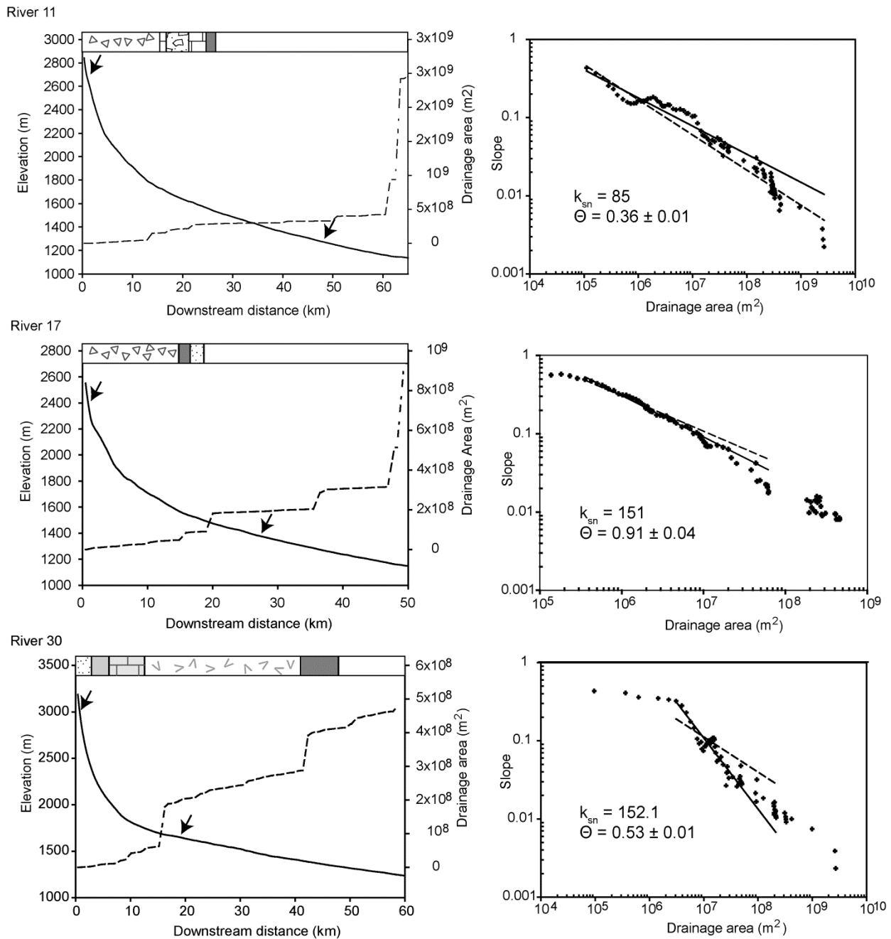
Figure 7. Representative examples of concave-up river profiles (solid lines) exhibiting consistent power-law scaling between drainage area and slope. Rivers profiles and drainage areas (dashed lines) were extracted from the SRTM DEM (USGS, 2006) and each river is labelled with a number that corresponds to those shown in figure 3. Arrows mark upstream and downstream limits of data used for regression analysis on the slope-area plots; the concavity, \Theta , and normalised steepness index, k_{sn} , where \Theta = 0.45 are also shown on the slope area plots. At the top of the long profile plot is a bar showing the lithology downstream (for key see Fig. 2)
