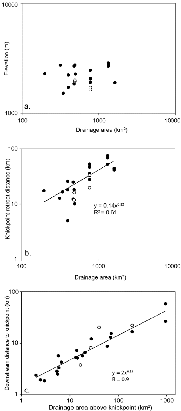
Figure 12. Graph of total drainage area versus elevation of the knickpoint, white circles indicate rivers where lithology plays a role in knickpoint position; b) Graph of total drainage area versus the distance the knickpoint has retreated from the thrust front. A linear regression yields the best fit power-law equation: y = 0.14A^{0.82} with R^2 = 0.61 ; c) Graph of drainage area (A) above knickpoint versus downstream distance from the divide (y) to the knickpoint. A linear regression yields the best fit power-law equation: y = 2A^{0.45} with R^2 = 0.9 .
