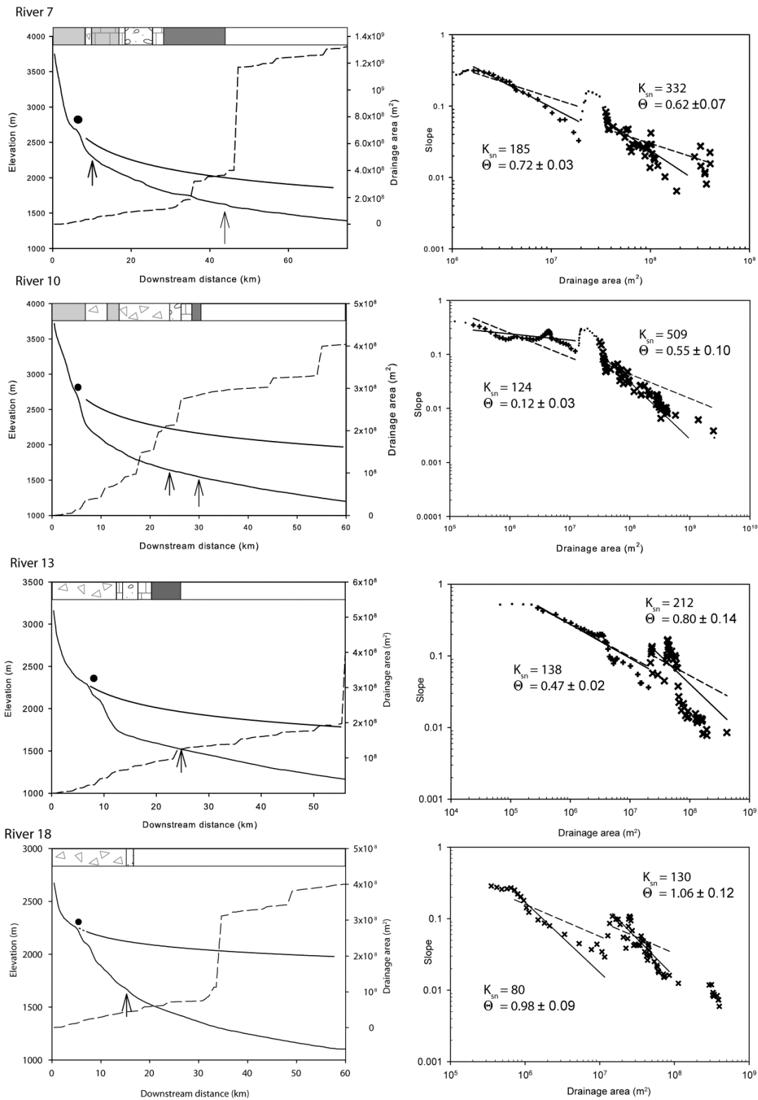
Figure 8. Representative examples of river profiles (solid lines) that exhibit knickpoints (circles) and segmented power-law scaling characteristic of slope-break knickpoints where k_{sn} increases downstream, each river is labelled with a number that corresponds to those shown in figure 3. Reconstructed relict profiles and position of the frontal thrust (arrow) are also shown. At the top of the long profile plot is a bar showing the lithology downstream (for key see Fig. 2).
