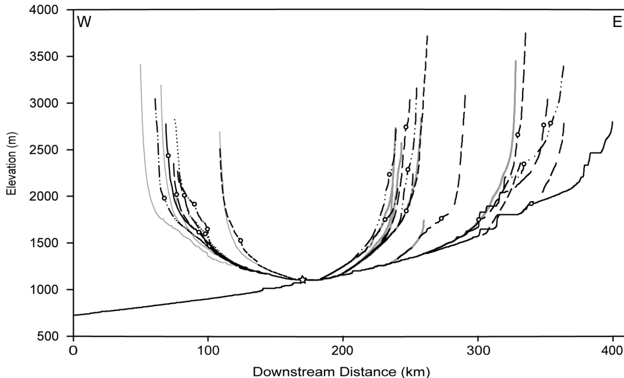
Figure 6. River long profiles of all rivers extracted; solid line is the Dades-Draa River, black dashed lines indicated rivers with knickpoints, and grey solid lines indicate rivers lacking knickpoints. The star shows the knickpoint associated with the Dades-Draa.
