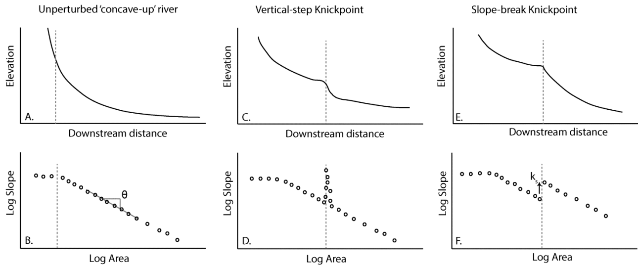
Figure 4. Schematic diagrams showing the river long profile and slope-area plot, respectively, for: a / b) an unperturbed concave-up river, the dashed line indicates the transition from debris flow to fluvial processes, note that downstream of this break.
