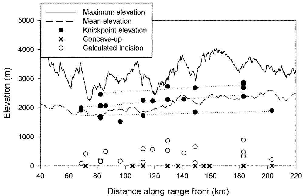
Figure 11. Knickpoint elevations (above mean sea level) and river incision plotted with maximum and average swath profiles of the range topography. Dotted lines shows potential vertical distribution of knickpoints into three elevation bands, analysis of horizontal knickpoint retreat distance against drainage area (Fig. 12b) shows that all knickpoints belong to the same generation and show a range in distribution.
