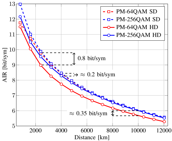
Fig. 2. AIRs vs. distance with nonbinary FEC and either SD or HD decoders, for PM-64QAM (red) and PM-256QAM (blue).
