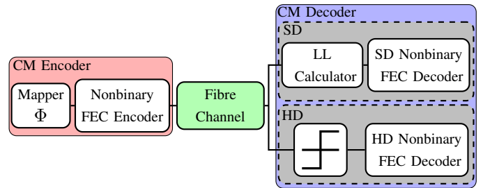
Fig. 1. Schematic diagram of a system using SD/HD nonbinary CM schemes.
