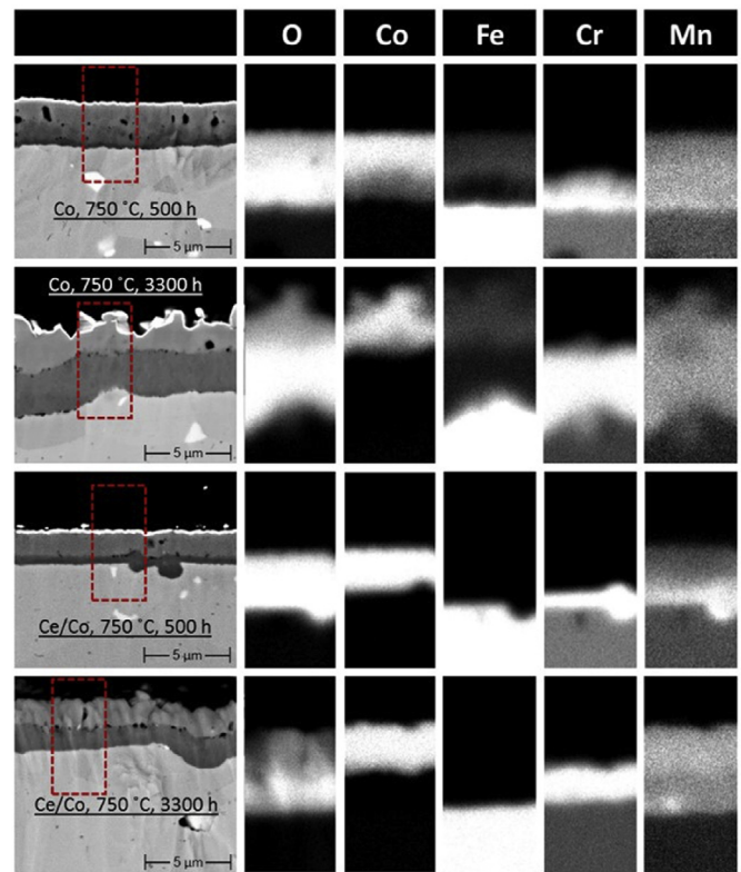
Fig. 6. Broad Ion Beam (BIB) cross-sections and their corresponding EDX maps of Co- and Ce/Co-coated Sanergy HT exposed for 500 and 3300 h at 750 °C in air containing 3% H 2 O using a flow rate of 6000 sml/min. The Ce content was too low and the resolution of SEM/EDX analysis is inferior to the size of the Ce-rich particles/layer. Thus mapping Ce was not possible.
