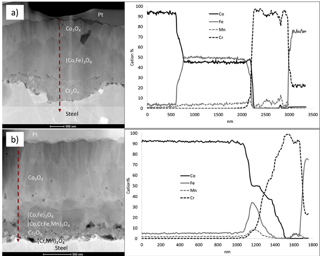
Fig. 4. STEM/EDX line scans along the oxide layer of Co-coated Sanergy HT exposed for 3300 h at 650 °C in air containing 3% \text{H}_2\text{O} with a flow rate set to 6000 sml/min. The two STEM images are taken from different areas of the oxide scale of the same sample, since rather large variations in thickness of the oxide scale were observed for the exclusively Co-coated samples exposed at 650 °C (See Fig. 5).
