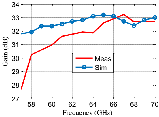
Fig. 6. Measured and computed realized gain of 16 \times 16 slot array antenna.
