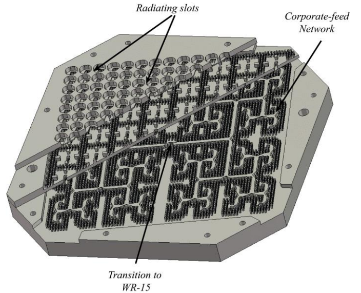
Fig. 3. Configuration of the proposed three-layer corporate-fed 16 \times 16 slot array antenna.
