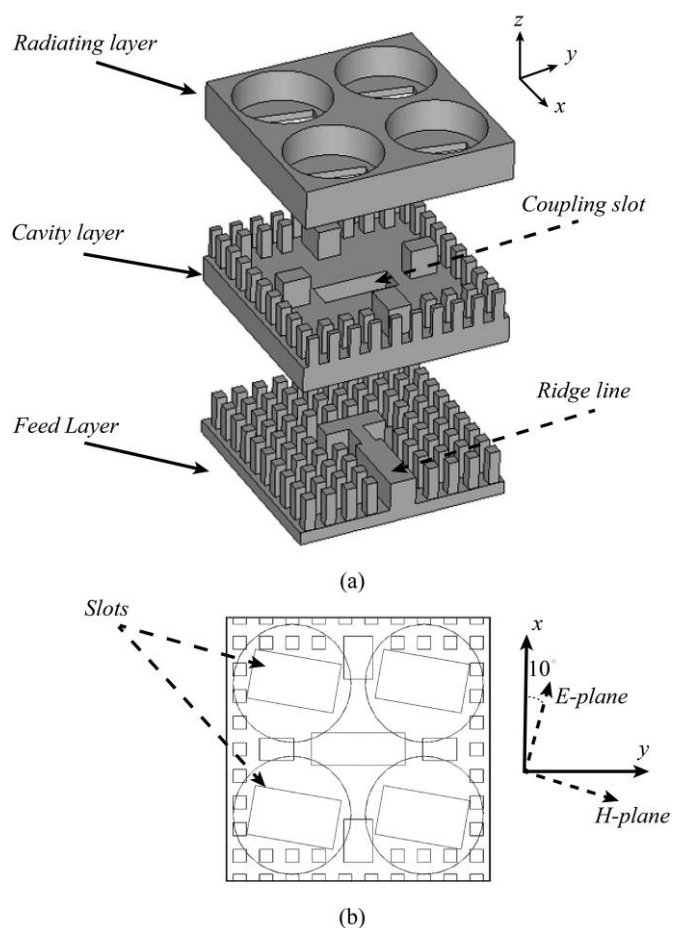
Fig. 1 The geometry of the cavity-backed 2 \times 2 slot subarray.
