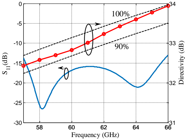
Fig. 2. Computed reflection coefficient of 2 \times 2 slot subarray and directivity of an array with 16 \times 16 slot aperture dimension in infinite array environment. The 100% and 90% lines corresponds to antenna efficiencies.
