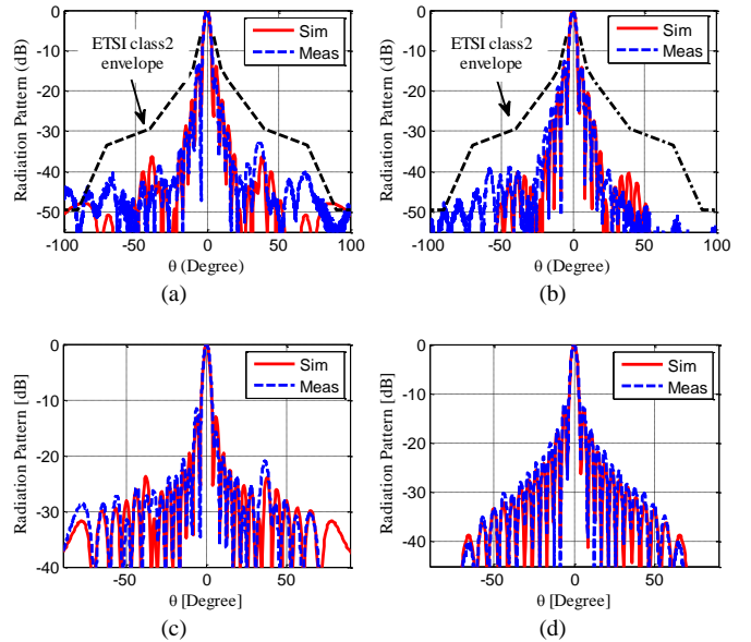
Fig. 7. Simulated and measured radiation patterns of the proposed array antenna at 64 GHz. (a) E-plane, (b) H-plane, (c) principle E-plane, and (d) principle H-plane.
