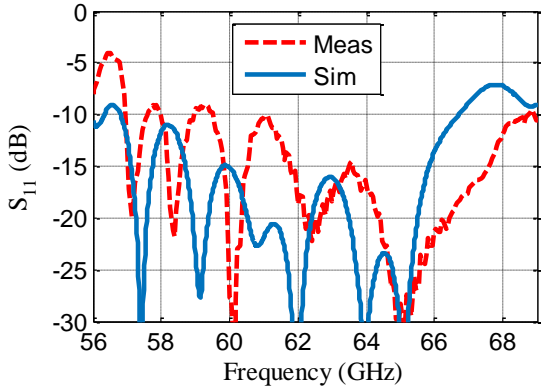
Fig. 5. Comparison of simulated and measured input reflection coefficient of the proposed 16 \times 16 slot array.
