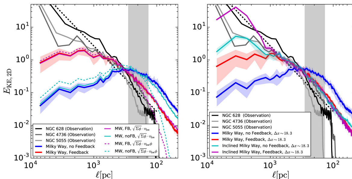
Figure 9. Direct comparison of the 2D kinetic energy ( \Sigma_{\text{HI}}^{1/2} v_{\text{los}} ) power spectra of NGC 628, 4736 and 5055 (black, dark grey and grey solid lines, respectively) from our THINGS sample and our MW simulation (red and blue solid lines). The grey shaded region indicates the range of beam sizes given for the subset of THINGS. Left: shown in magenta (feedback) and cyan (no feedback) are the results of first convolving the surface density map (solid lines) and the surface density map as well as the velocity map (dashed lines) with a Gaussian (FWHM = 100 pc). Right: inclination test. Time-averaged spectra of the simulations inclined at 40^\circ are shown in magenta (feedback) and cyan (no feedback). All simulation spectra in this panel are calculated at a resolution of \Delta x \sim 18.3 pc. These spectra are all normalized, see Section 3.3.2 for details.
