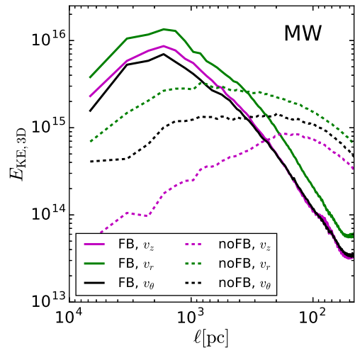
Figure 11. Time-averaged 3D kinetic energy ( \rho_{\text{all}}^{1/2} v_c ) power spectra for each velocity component of the MW simulations. We show the vertical ( v_z , magenta), radial ( v_r , green) and tangential ( v_\theta , black) velocity components. We distinguish between feedback and no feedback with solid and dashed lines, respectively. We note that we have not normalized, i.e. they show the relative power of each component.
