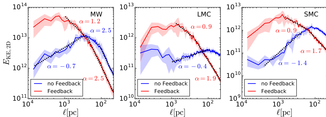
Figure 8. 2D kinetic energy ( \Sigma_{\text{HI}}^{1/2} v_{\text{los}} ) time-averaged power spectra for our simulations. From left to right, we show the resulting spectra from the MW, LMC and SMC models with feedback shown in red and no feedback shown in blue. The dashed black lines show our fitted power law with gradients next to each fit. The shaded regions around each power spectrum show the 1\sigma deviation from the mean. The E(k) presented here have not been normalized.
